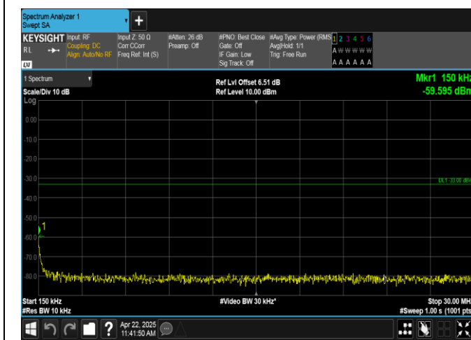
Band2-3MHz-QPSK-18900-15RB#0-0.15~30-PASS
