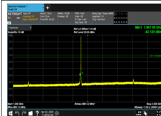
Band2-3MHz-16QAM-19185-15RB#0-1000~3000-PASS
