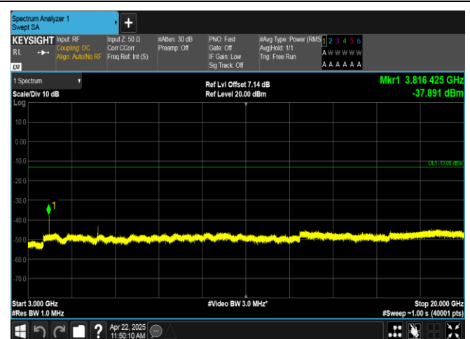
Band2-3MHz-16QAM-19185-15RB#0-3000~20000-PASS
