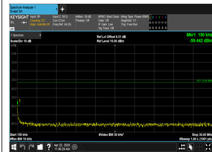
Band2-3MHz-16QAM-18615-15RB#0-0.15~30-PASS
