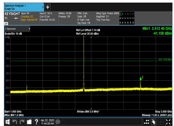
Band2-3MHz-QPSK-19185-1RB#0-1000~3000-PASS
