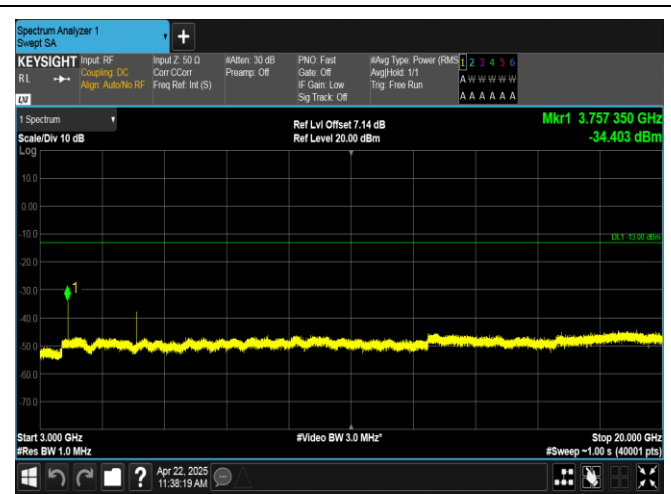
Band2-3MHz-QPSK-18900-1RB#0-3000~20000-PASS
