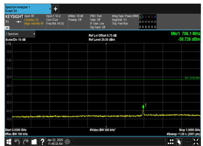
Band2-3MHz-16QAM-19185-15RB#0-30~1000-PASS
