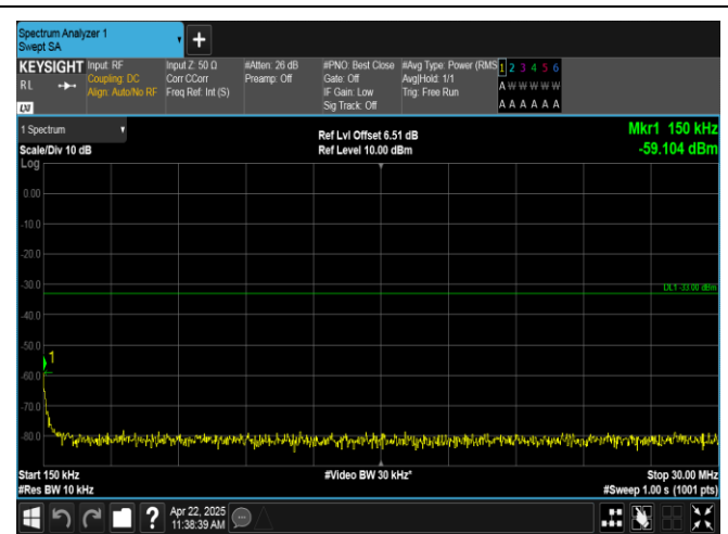
Band2-3MHz-16QAM-18900-1RB#0-0.15~30-PASS
