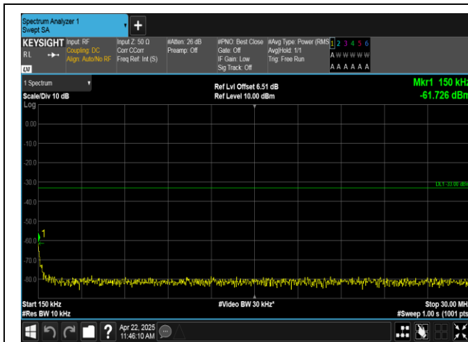
Band2-3MHz-QPSK-19185-1RB#14-0.15~30-PASS
