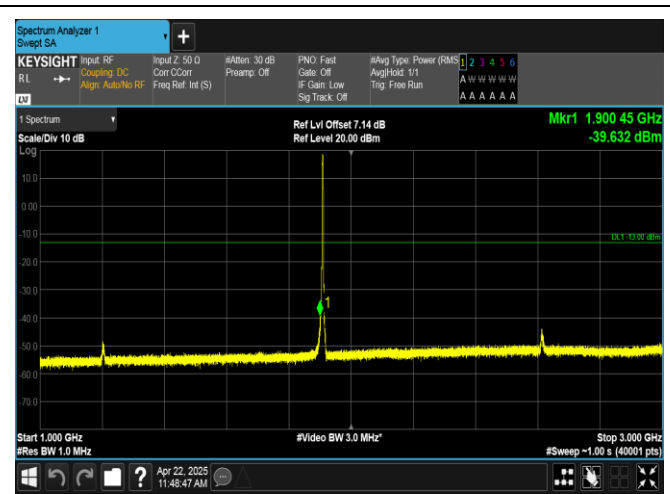
Band2-3MHz-QPSK-19185-15RB#0-1000~3000-PASS
