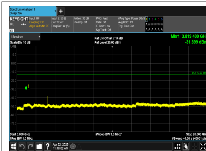
Band2-3MHz-16QAM-19185-1RB#14-3000~20000-PASS
