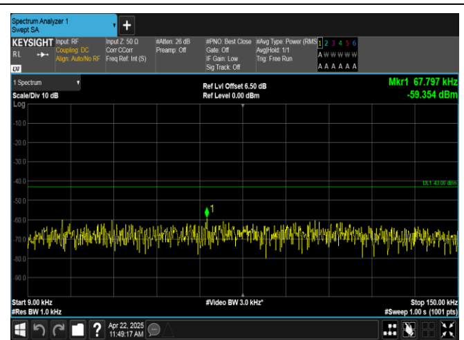
Band2-3MHz-16QAM-19185-15RB#0-0.009~0.15-PASS
