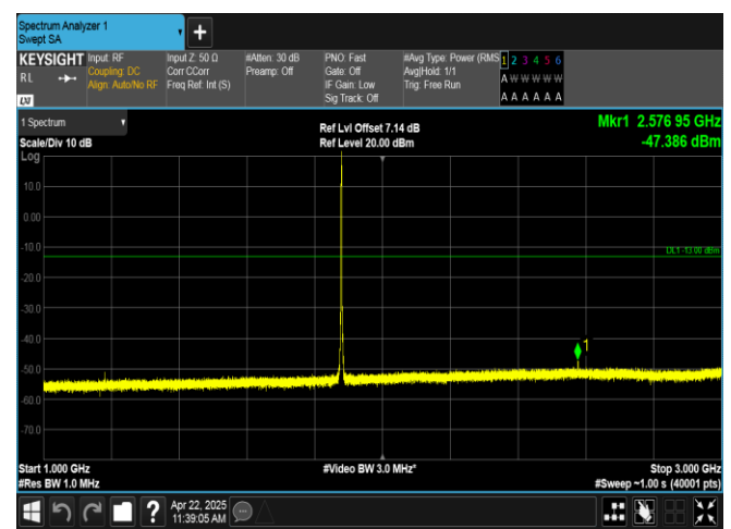
Band2-3MHz-16QAM-18900-1RB#0-1000~3000-PASS
