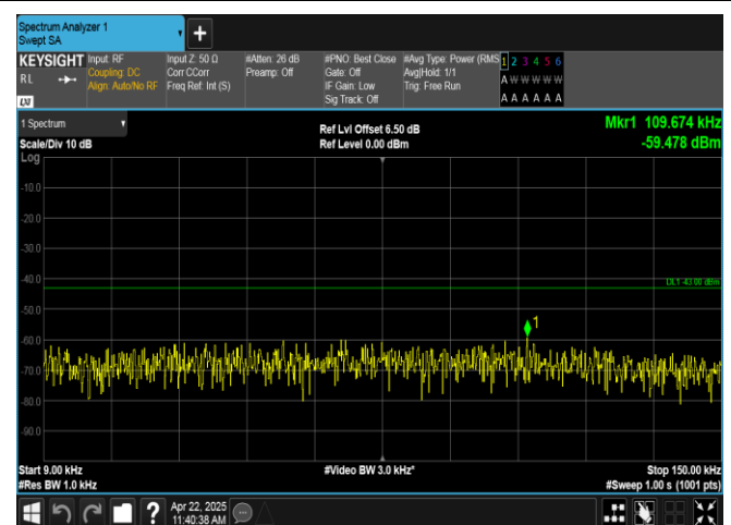
Band2-3MHz-16QAM-18900-1RB#14-0.009~0.15-PASS
