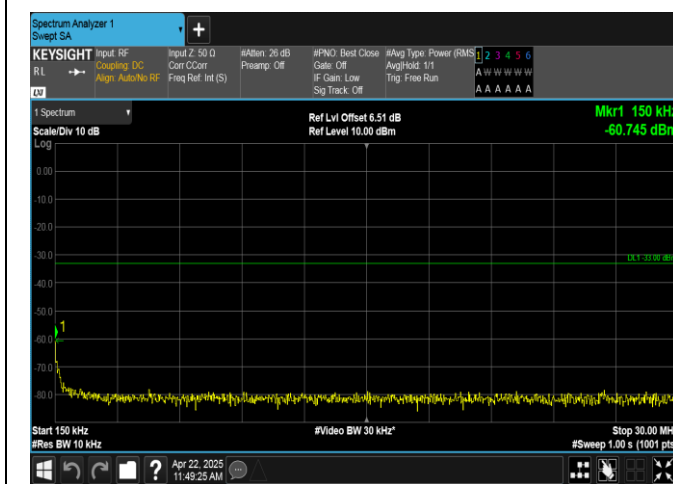
Band2-3MHz-16QAM-19185-15RB#0-0.15~30-PASS
