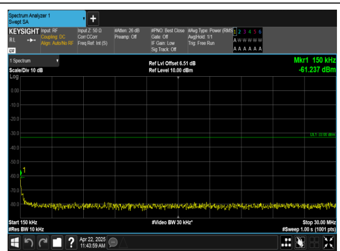
Band2-3MHz-QPSK-19185-1RB#0-0.15~30-PASS
