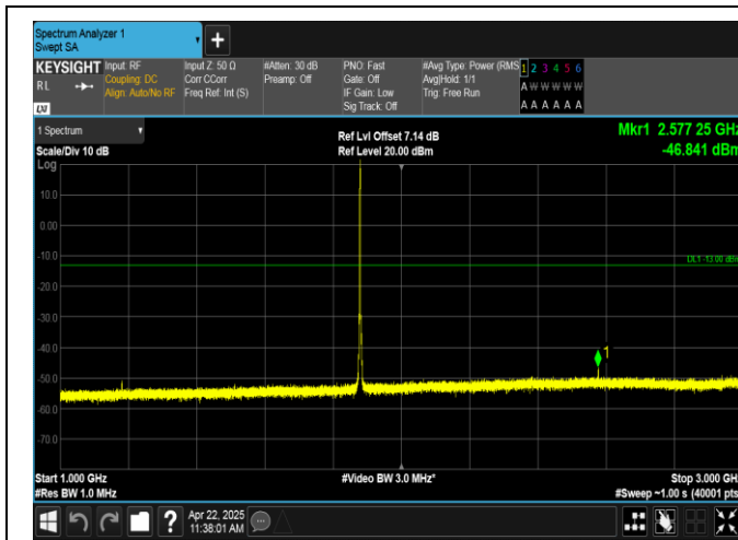
Band2-3MHz-QPSK-18900-1RB#0-1000~3000-PASS
