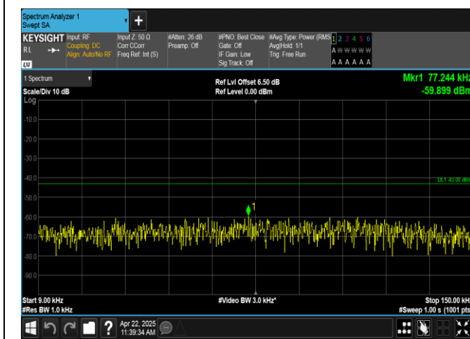
Band2-3MHz-QPSK-18900-1RB#14-0.009~0.15-PASS
