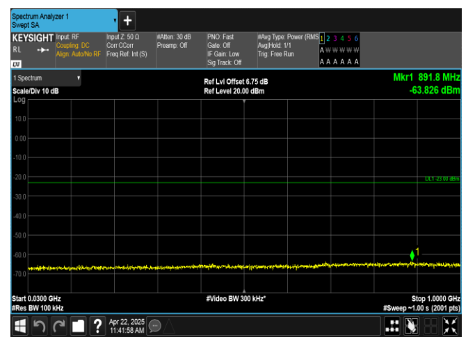
Band2-3MHz-QPSK-18900-15RB#0-30~1000-PASS
