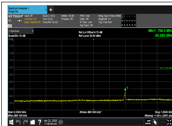
Band2-1.4MHz-QPSK-19193-6RB#0-30~1000-PASS
