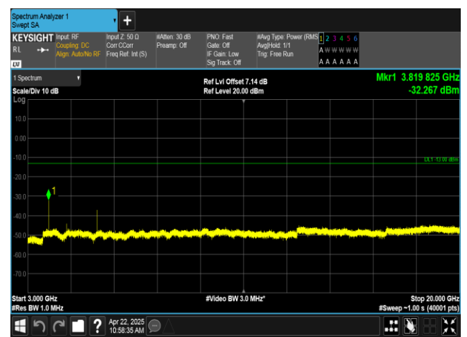
Band2-1.4MHz-QPSK-19193-1RB#5-3000~20000-PASS
