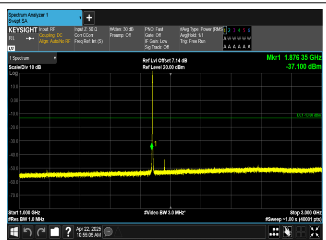
Band2-1.4MHz-16QAM-18900-6RB#0-1000~3000-PASS
