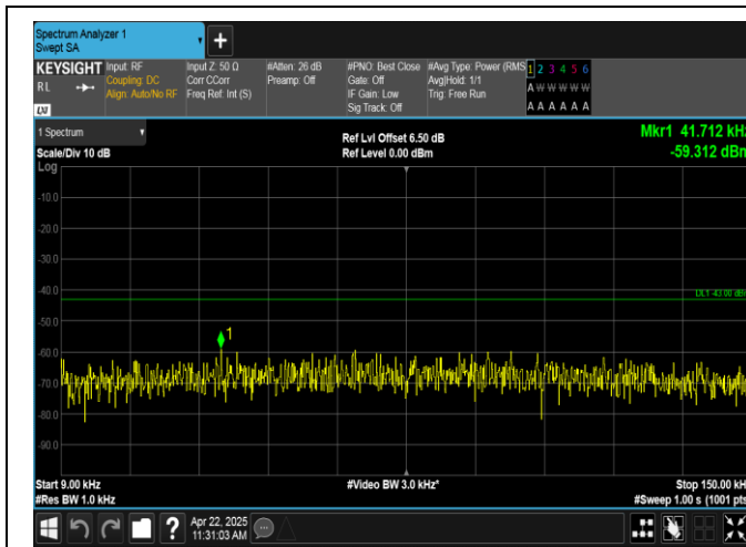
Band2-3MHz-QPSK-18615-1RB#0-0.009~0.15-PASS
