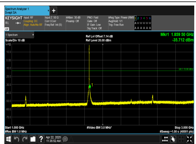
Band2-3MHz-QPSK-18615-15RB#0-1000~3000-PASS
