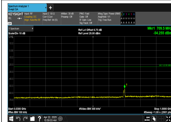
Band2-1.4MHz-16QAM-19193-1RB#5-30~1000-PASS
