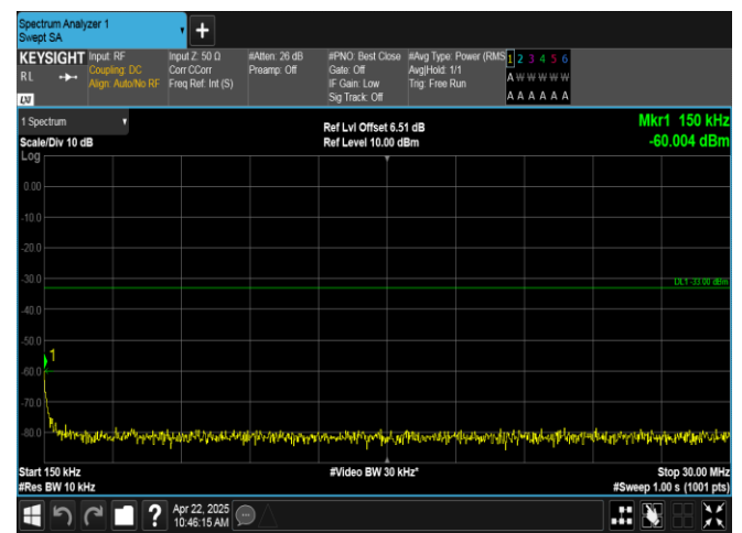
Band2-1.4MHz-16QAM-18607-1RB#5-0.15~30-PASS
