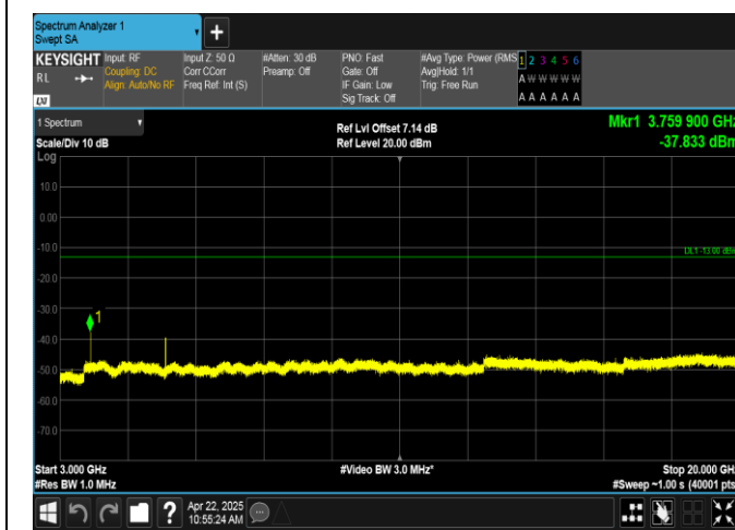
Band2-1.4MHz-16QAM-18900-6RB#0-3000~20000-PASS
