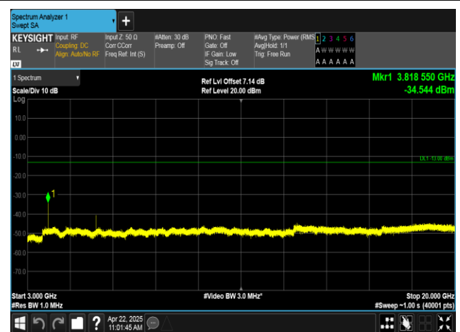
Band2-1.4MHz-16QAM-19193-6RB#0-3000~20000-PASS
