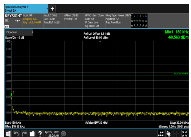
Band2-3MHz-QPSK-18615-15RB#0-0.15~30-PASS
