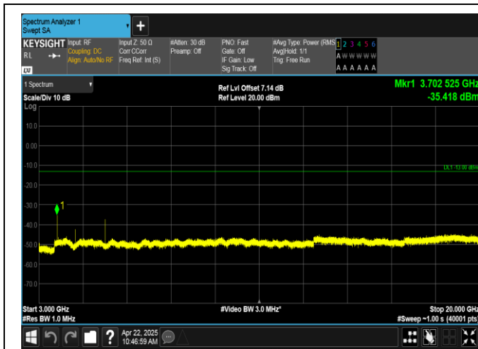
Band2-1.4MHz-16QAM-18607-1RB#5-3000~20000-PASS
