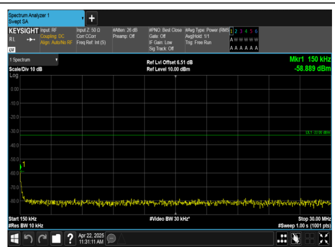
Band2-3MHz-QPSK-18615-1RB#0-0.15~30-PASS
