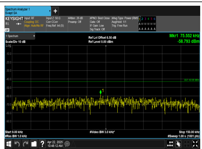
Band2-1.4MHz-16QAM-18607-6RB#0-0.009~0.15-PASS
