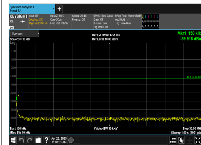
Band2-1.4MHz-16QAM-19193-6RB#0-0.15~30-PASS
