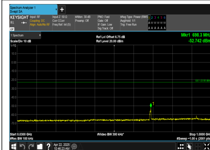
Band2-1.4MHz-16QAM-18607-1RB#5-30~1000-PASS
