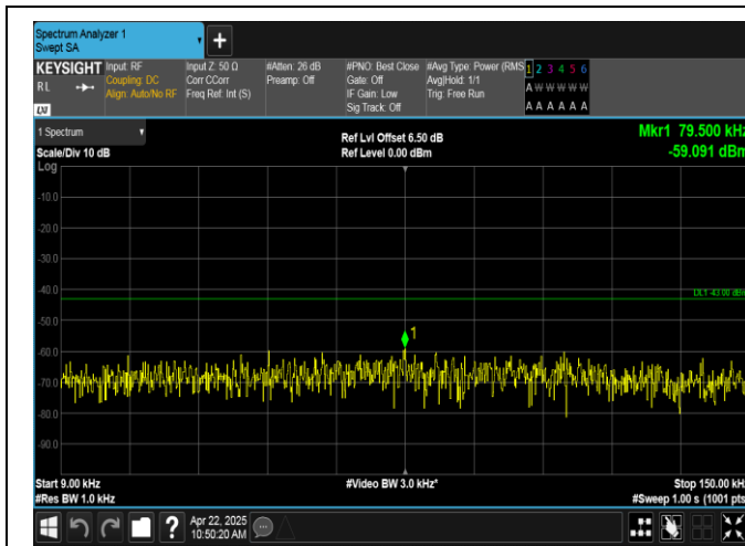
Band2-1.4MHz-16QAM-18900-1RB#0-0.009~0.15-PASS
