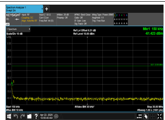
Band2-1.4MHz-QPSK-19193-1RB#0-0.15~30-PASS
