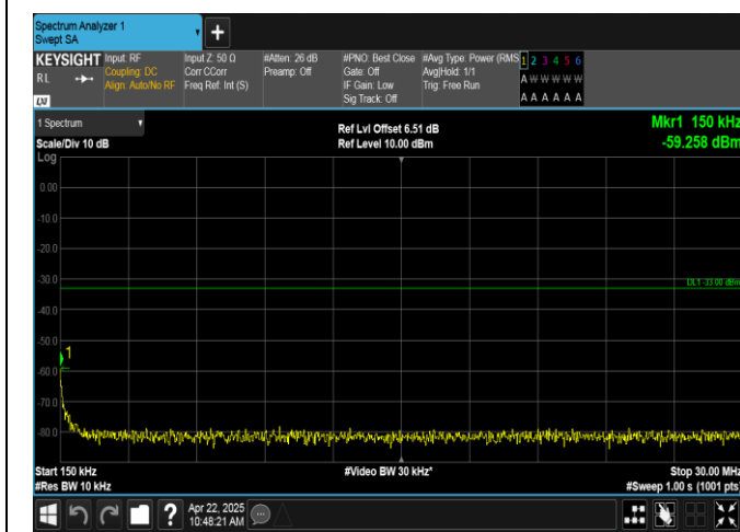
Band2-1.4MHz-16QAM-18607-6RB#0-0.15~30-PASS
