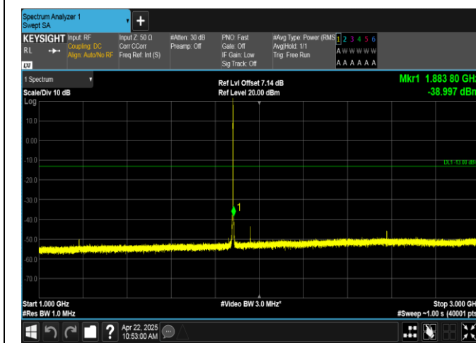
Band2-1.4MHz-16QAM-18900-1RB#5-1000~3000-PASS
