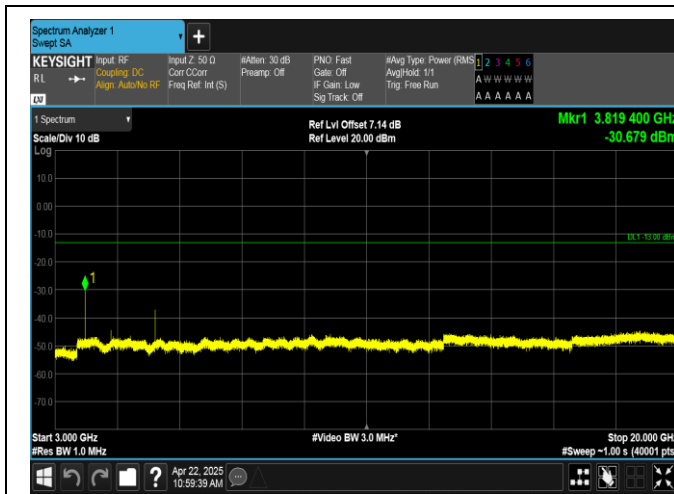
Band2-1.4MHz-16QAM-19193-1RB#5-3000~20000-PASS
