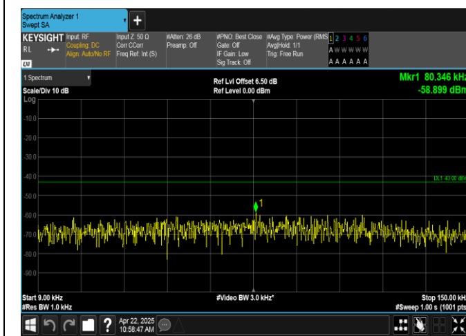
Band2-1.4MHz-16QAM-19193-1RB#5-0.009~0.15-PASS
