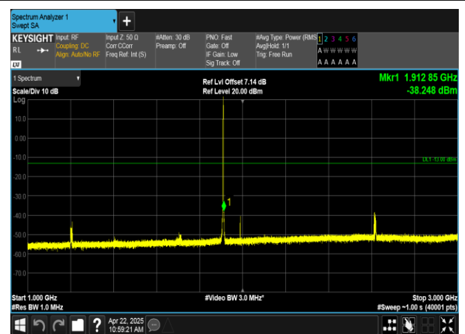
Band2-1.4MHz-16QAM-19193-1RB#5-1000~3000-PASS
