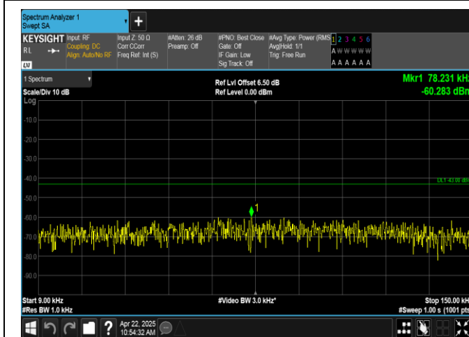
Band2-1.4MHz-16QAM-18900-6RB#0-0.009~0.15-PASS
