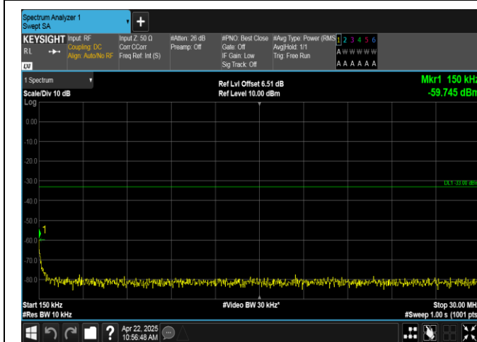
Band2-1.4MHz-16QAM-19193-1RB#0-0.15~30-PASS
