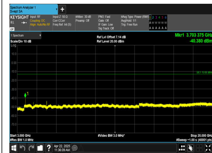
Band2-3MHz-QPSK-18615-15RB#0-3000~20000-PASS
