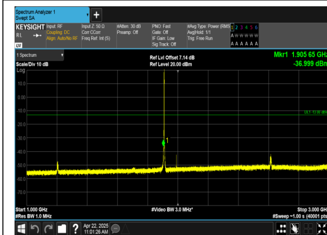
Band2-1.4MHz-16QAM-19193-6RB#0-1000~3000-PASS
