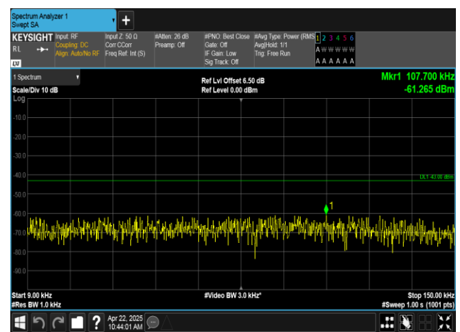
Band2-1.4MHz-16QAM-18607-1RB#0-0.009~0.15-PASS
