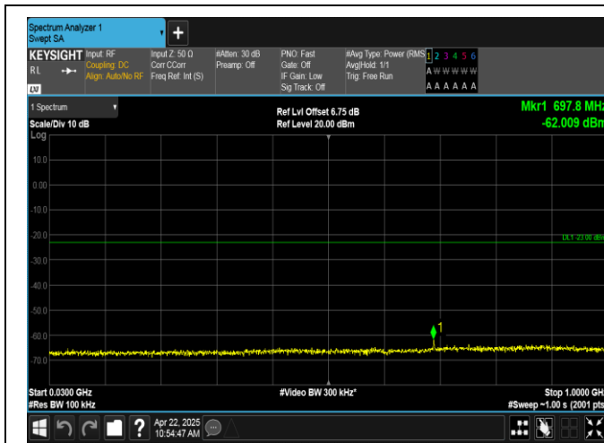
Band2-1.4MHz-16QAM-18900-6RB#0-30~1000-PASS
