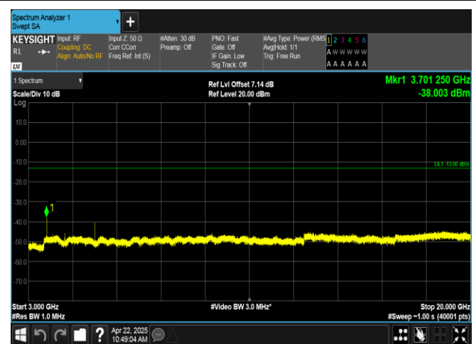
Band2-1.4MHz-16QAM-18607-6RB#0-3000~20000-PASS
