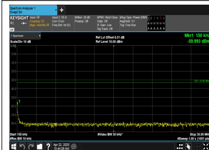
Band2-1.4MHz-16QAM-18607-1RB#0-0.15~30-PASS
