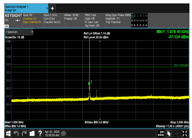
Band2-1.4MHz-16QAM-18900-1RB#0-1000~3000-PASS
