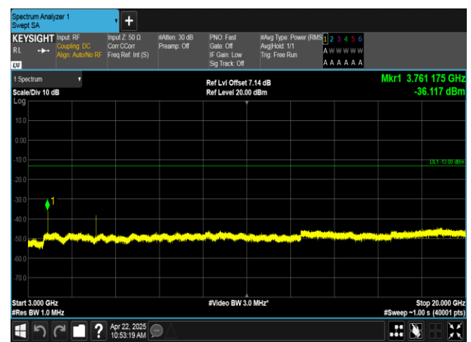
Band2-1.4MHz-16QAM-18900-1RB#5-3000~20000-PASS
