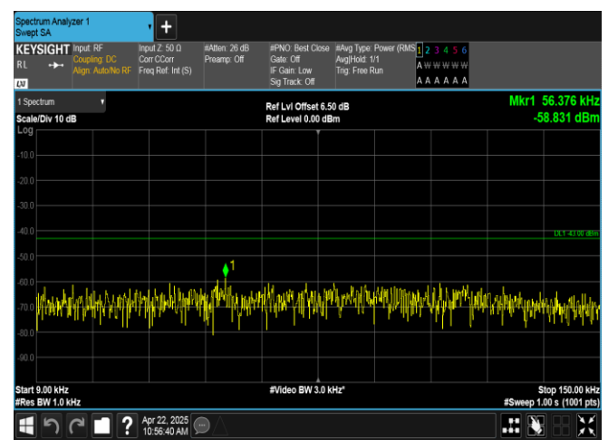
Band2-1.4MHz-16QAM-19193-1RB#0-0.009~0.15-PASS
