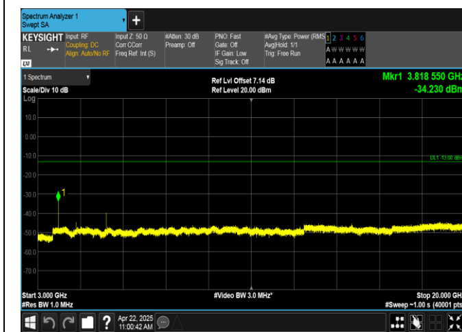
Band2-1.4MHz-QPSK-19193-6RB#0-3000~20000-PASS
