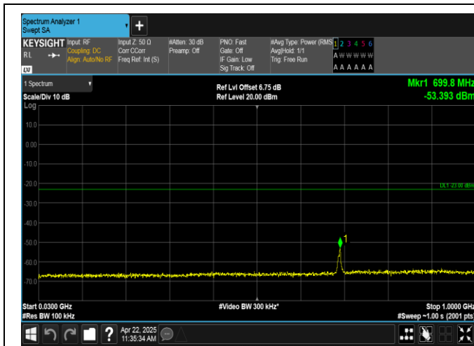
Band2-3MHz-QPSK-18615-15RB#0-30~1000-PASS
