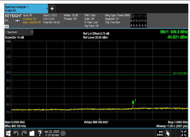
Band2-3MHz-QPSK-18900-1RB#0-30~1000-PASS
