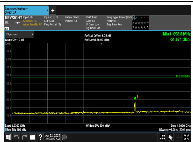
Band2-3MHz-QPSK-18615-1RB#14-30~1000-PASS
