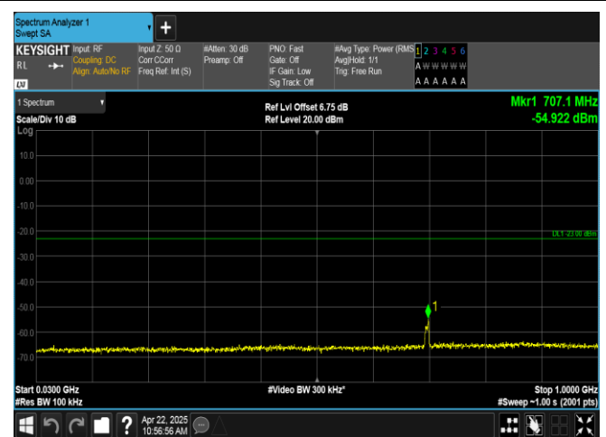
Band2-1.4MHz-16QAM-19193-1RB#0-30~1000-PASS
