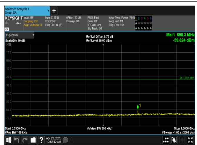
Band2-1.4MHz-16QAM-18900-1RB#5-30~1000-PASS
