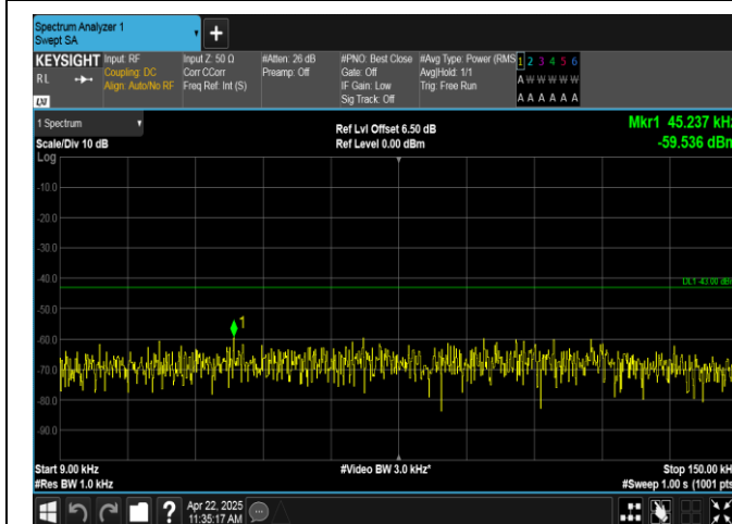
Band2-3MHz-QPSK-18615-15RB#0-0.009~0.15-PASS
