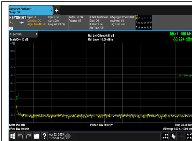
Band2-1.4MHz-16QAM-18900-1RB#5-0.15~30-PASS
