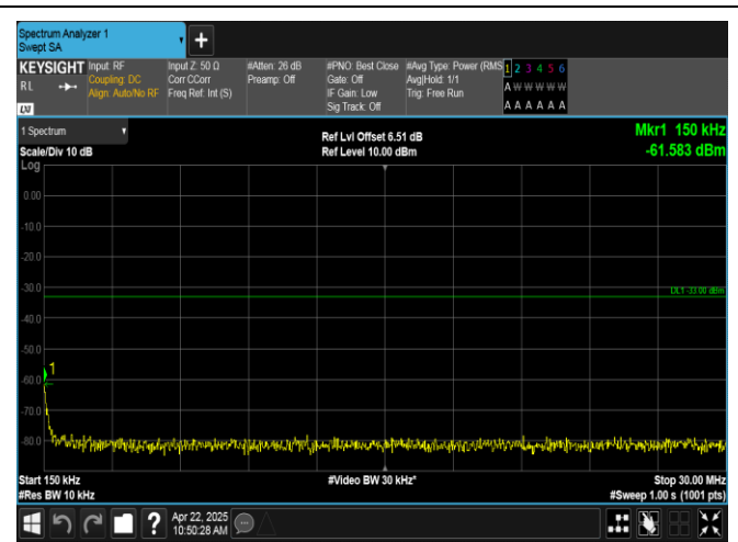
Band2-1.4MHz-16QAM-18900-1RB#0-0.15~30-PASS
