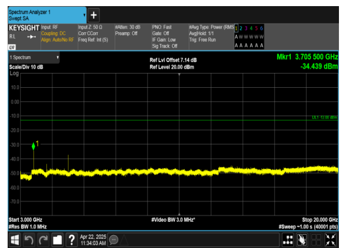
Band2-3MHz-QPSK-18615-1RB#14-3000~20000-PASS
