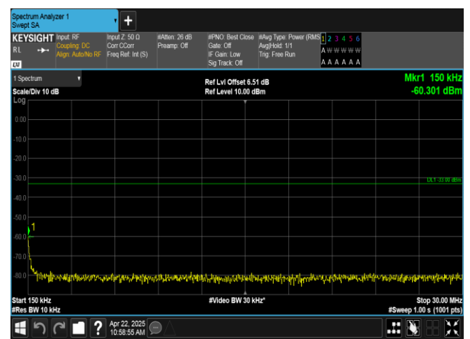
Band2-1.4MHz-16QAM-19193-1RB#5-0.15~30-PASS
