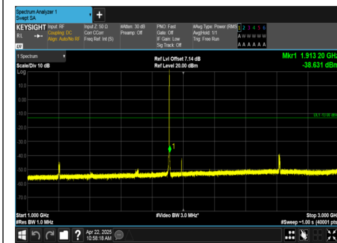
Band2-1.4MHz-QPSK-19193-1RB#5-1000~3000-PASS
