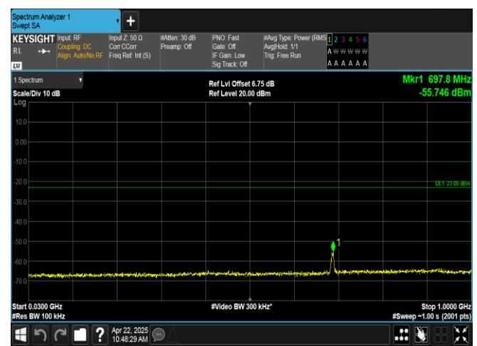
Band2-1.4MHz-16QAM-18607-6RB#0-30~1000-PASS
