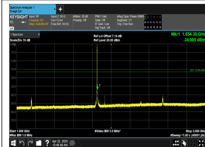
Band2-1.4MHz-16QAM-18607-6RB#0-1000~3000-PASS
