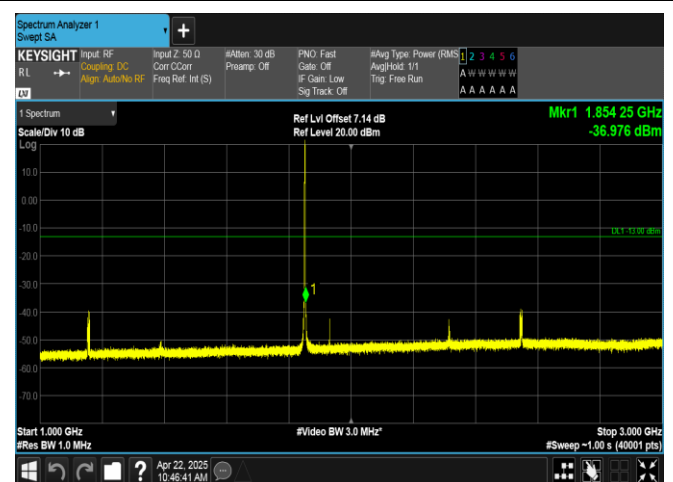
Band2-1.4MHz-16QAM-18607-1RB#5-1000~3000-PASS
