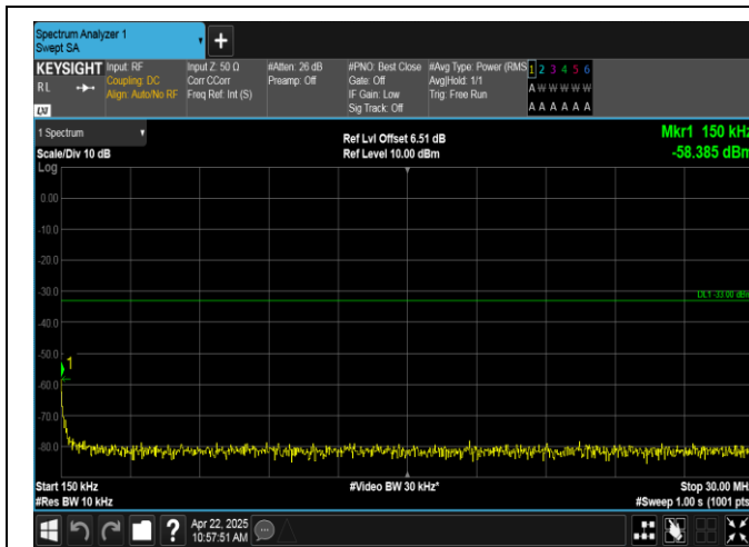
Band2-1.4MHz-QPSK-19193-1RB#5-0.15~30-PASS
