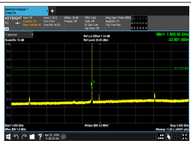
Band2-1.4MHz-QPSK-19193-6RB#0-1000~3000-PASS
