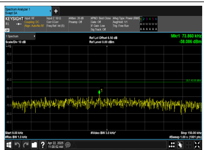
Band2-1.4MHz-16QAM-19193-6RB#0-0.009~0.15-PASS
