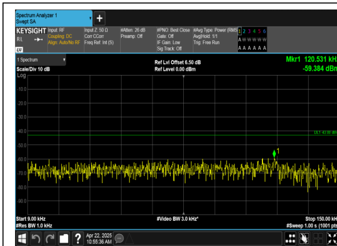
Band2-1.4MHz-QPSK-19193-1RB#0-0.009~0.15-PASS
