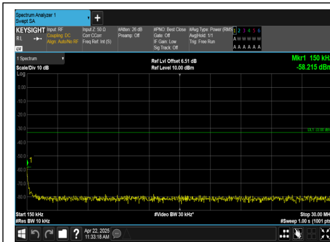
Band2-3MHz-QPSK-18615-1RB#14-0.15~30-PASS
