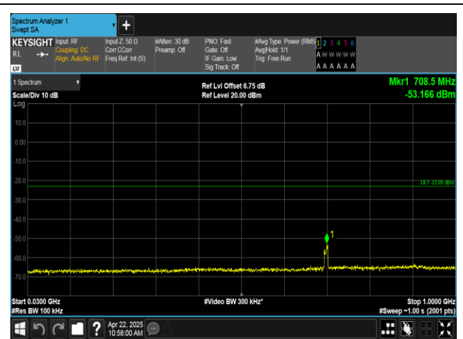
Band2-1.4MHz-QPSK-19193-1RB#5-30~1000-PASS
