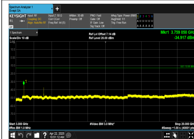
Band2-1.4MHz-16QAM-18900-1RB#0-3000~20000-PASS
