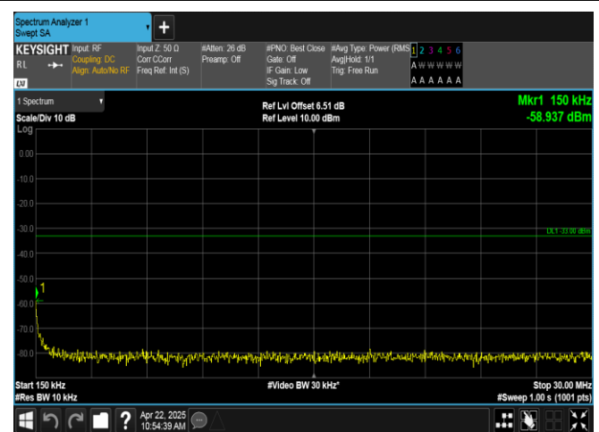
Band2-1.4MHz-16QAM-18900-6RB#0-0.15~30-PASS
