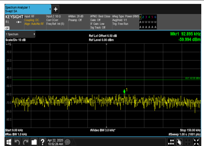
Band2-1.4MHz-16QAM-18900-1RB#5-0.009~0.15-PASS
