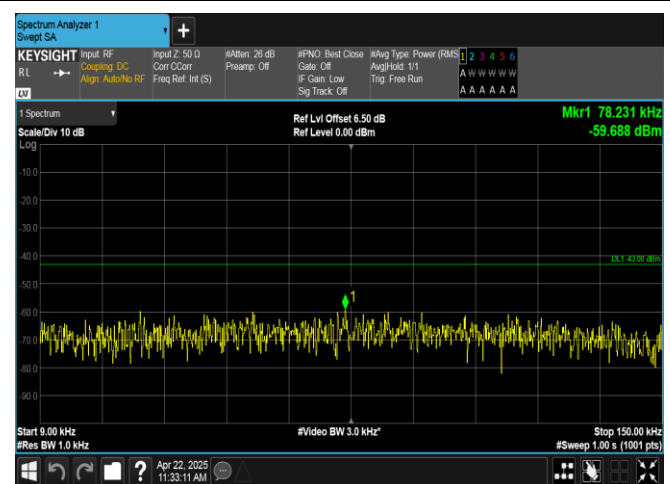
Band2-3MHz-QPSK-18615-1RB#14-0.009~0.15-PASS
