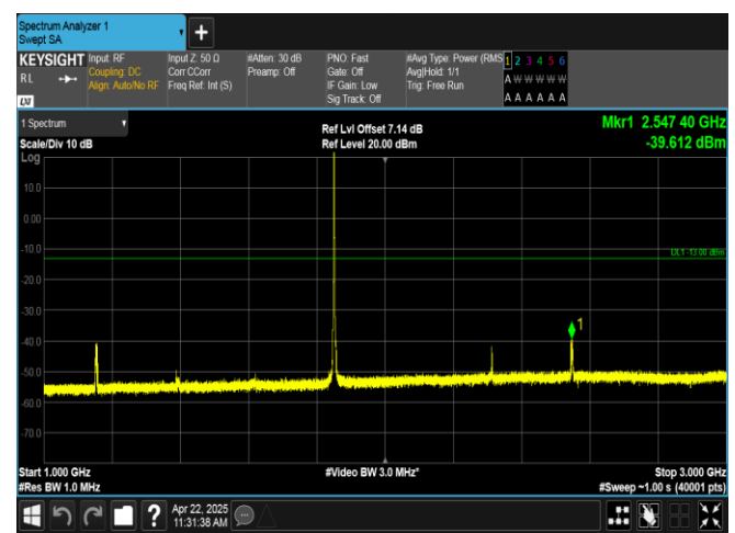
Band2-3MHz-QPSK-18615-1RB#0-1000~3000-PASS
