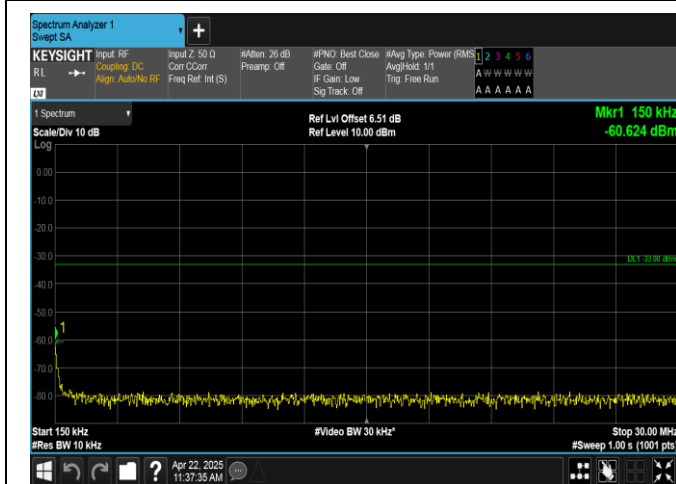
Band2-3MHz-QPSK-18900-1RB#0-0.15~30-PASS
