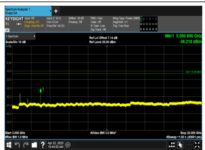
Band2-1.4MHz-16QAM-18607-1RB#0-3000~20000-PASS
