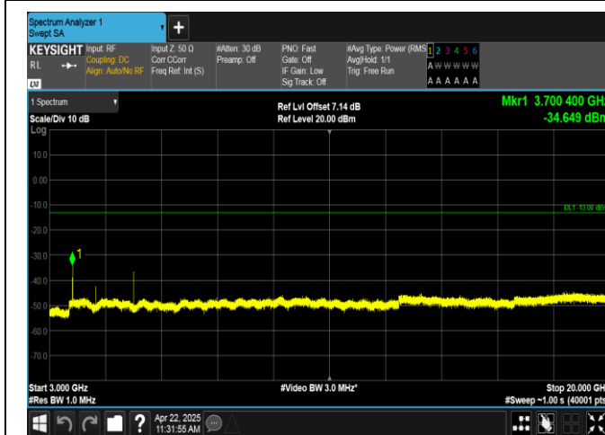
Band2-3MHz-QPSK-18615-1RB#0-3000~20000-PASS
