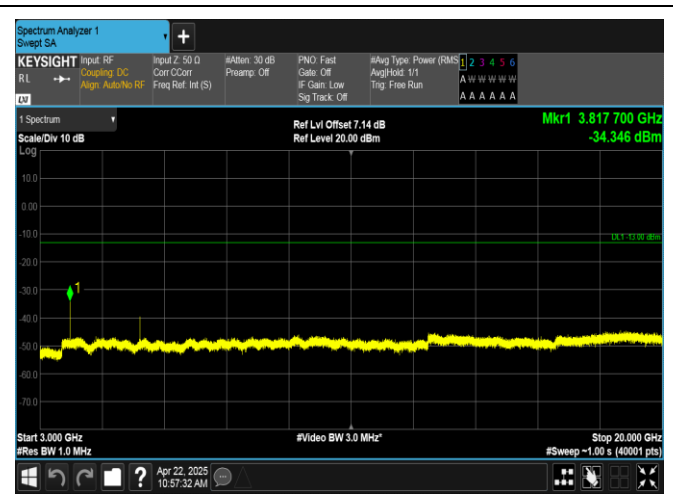
Band2-1.4MHz-16QAM-19193-1RB#0-3000~20000-PASS
