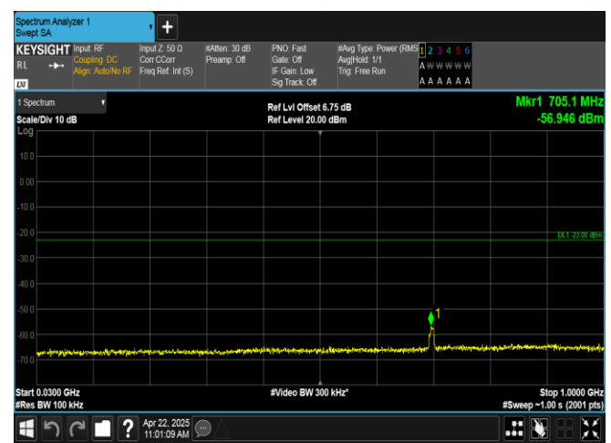
Band2-1.4MHz-16QAM-19193-6RB#0-30~1000-PASS
