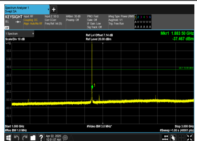
Band2-1.4MHz-QPSK-18900-1RB#5-1000~3000-PASS
