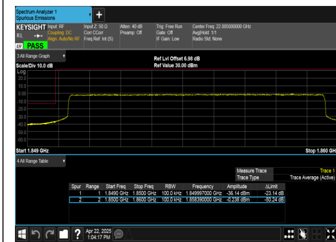
Band2-10MHz-16QAM-18650-50RB#0-PASS
