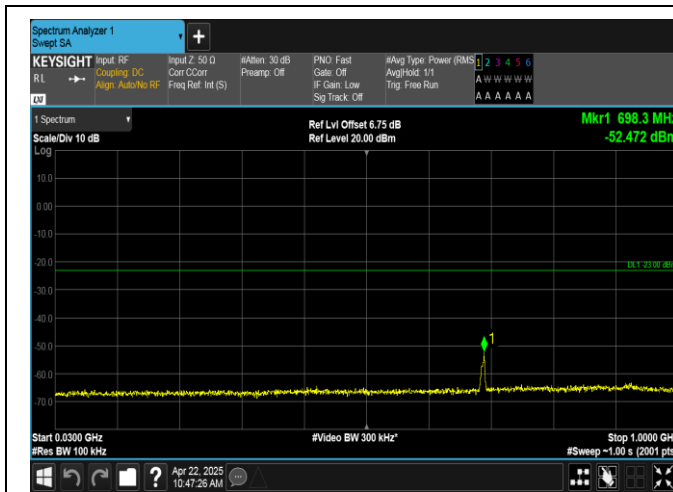
Band2-1.4MHz-QPSK-18607-6RB#0-30~1000-PASS
