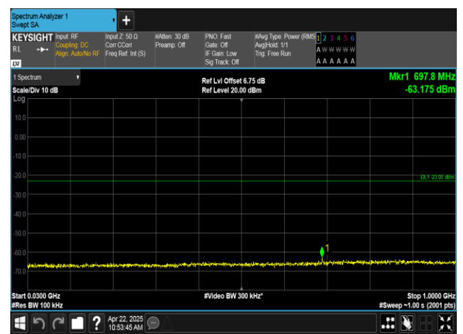
Band2-1.4MHz-QPSK-18900-6RB#0-30~1000-PASS
