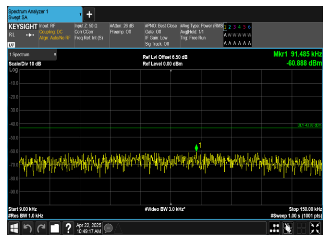
Band2-1.4MHz-QPSK-18900-1RB#0-0.009~0.15-PASS
