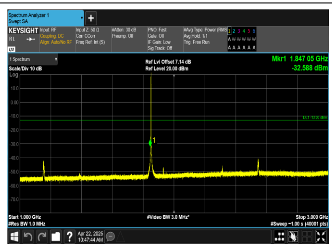
Band2-1.4MHz-QPSK-18607-6RB#0-1000~3000-PASS
