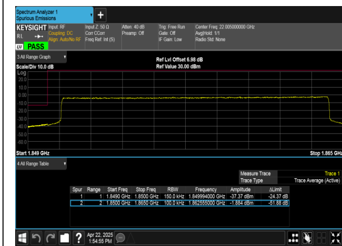
Band2-15MHz-16QAM-18675-75RB#0-PASS
