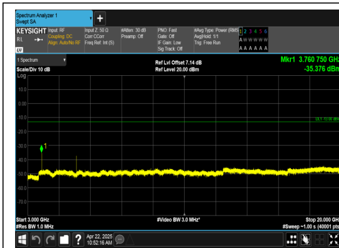
Band2-1.4MHz-QPSK-18900-1RB#5-3000~20000-PASS
