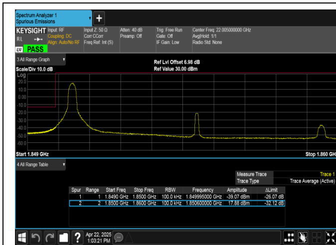
Band2-10MHz-16QAM-18650-1RB#0-PASS
