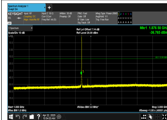
Band2-1.4MHz-QPSK-18900-6RB#0-1000~3000-PASS
