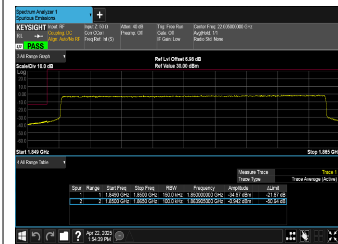
Band2-15MHz-QPSK-18675-75RB#0-PASS
