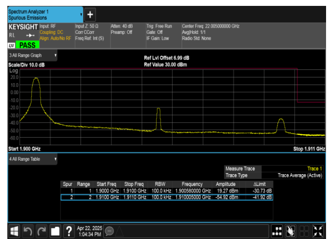
Band2-10MHz-QPSK-19150-1RB#0-PASS
