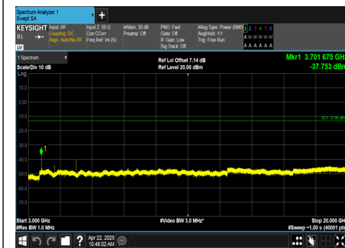
Band2-1.4MHz-QPSK-18607-6RB#0-3000~20000-PASS
