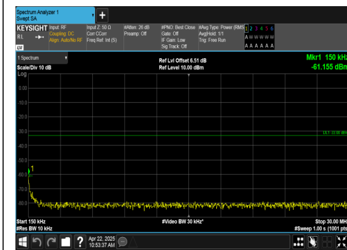
Band2-1.4MHz-QPSK-18900-6RB#0-0.15~30-PASS
