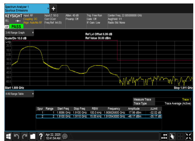
Band2-1.4MHz-16QAM-19193-1RB#0-PASS
