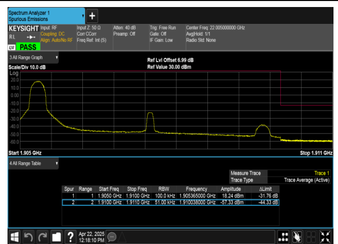
Band2-5MHz-16QAM-19175-1RB#0-PASS
