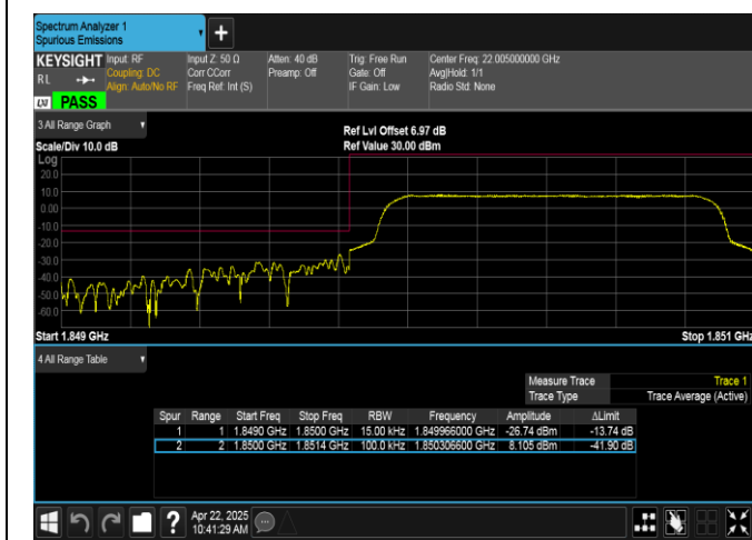
Band2-1.4MHz-16QAM-18607-6RB#0-PASS
