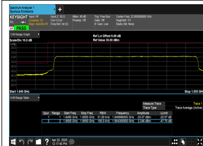
Band2-5MHz-16QAM-18625-25RB#0-PASS
