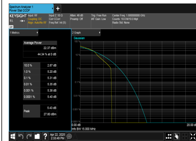
Band2-15MHz-16QAM-18900-1RB#0-PASS
