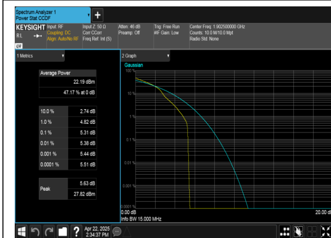
Band2-15MHz-16QAM-19125-1RB#0-PASS
