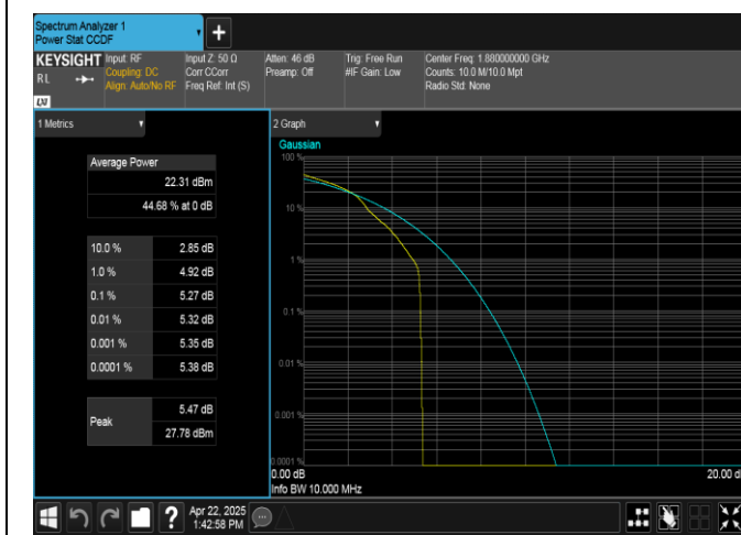
Band2-10MHz-16QAM-18900-1RB#0-PASS
