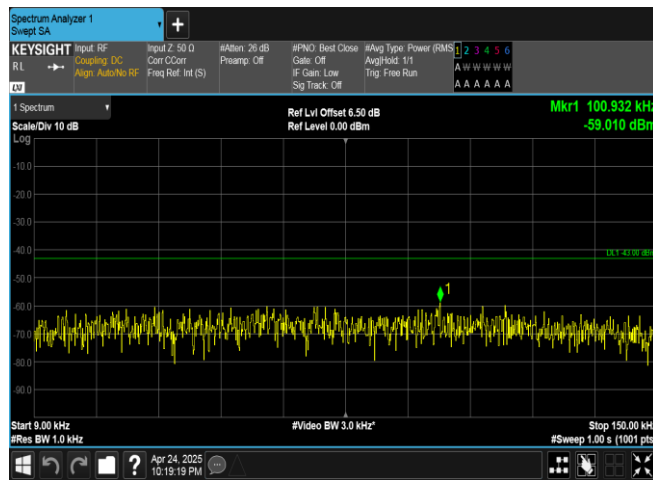
Band4-1413-2-0.009~0.15MHz-PASS
