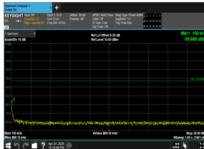
Band4-1413-1-0.15~30MHz-PASS
