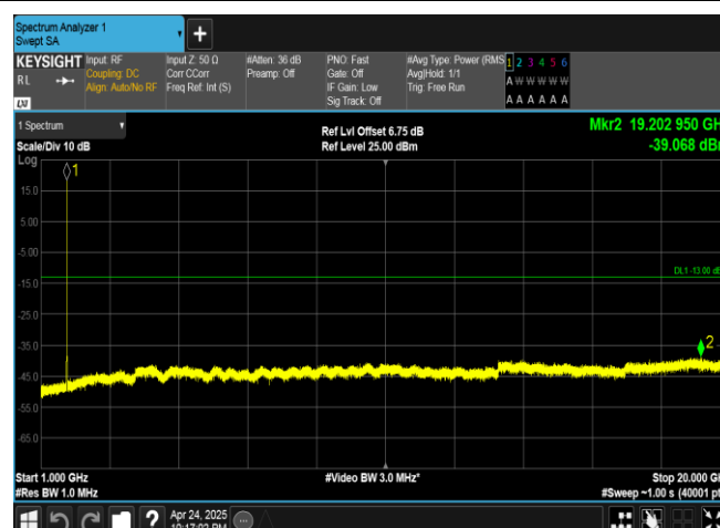
Band4-1413-1-1000~20000MHz-PASS
