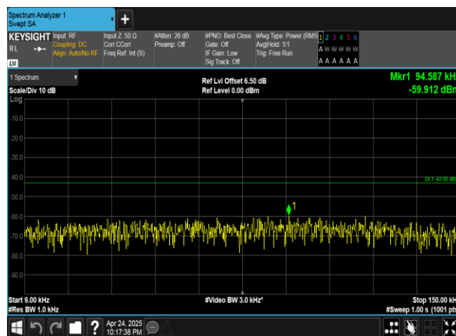
Band4-1513-1-0.009~0.15MHz-PASS
