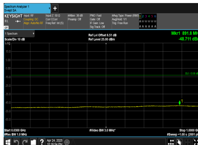
Band4-1413-1-30~1000MHz-PASS
