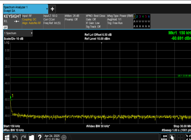
Band4-1413-3-0.15~30MHz-PASS
