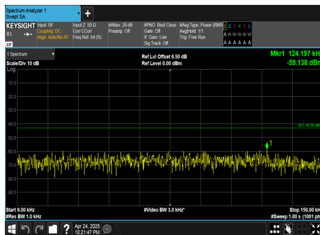
Band4-1413-3-0.009~0.15MHz-PASS
