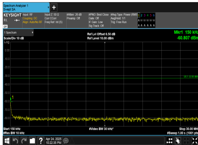
Band4-1513-3-0.15~30MHz-PASS
