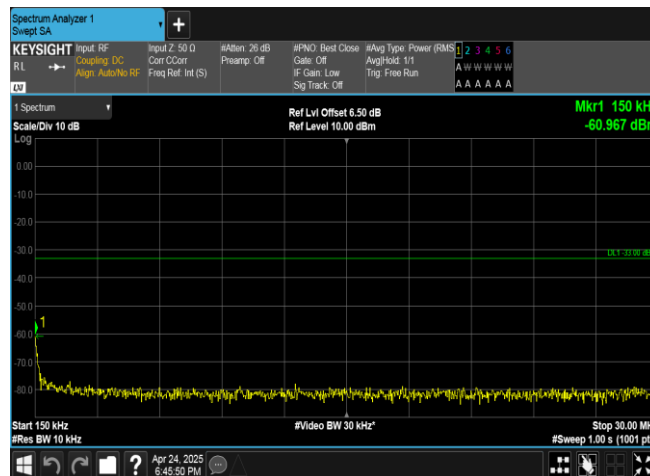
Band2-9400-1-0.15~30MHz-PASS
