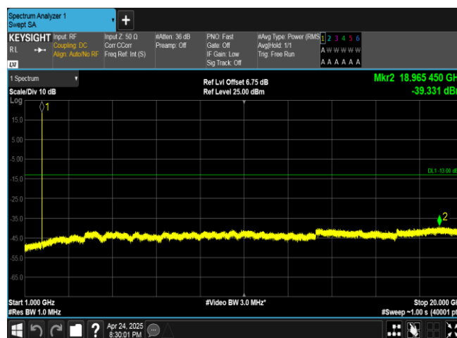
Band4-1513-1-1000~20000MHz-PASS
