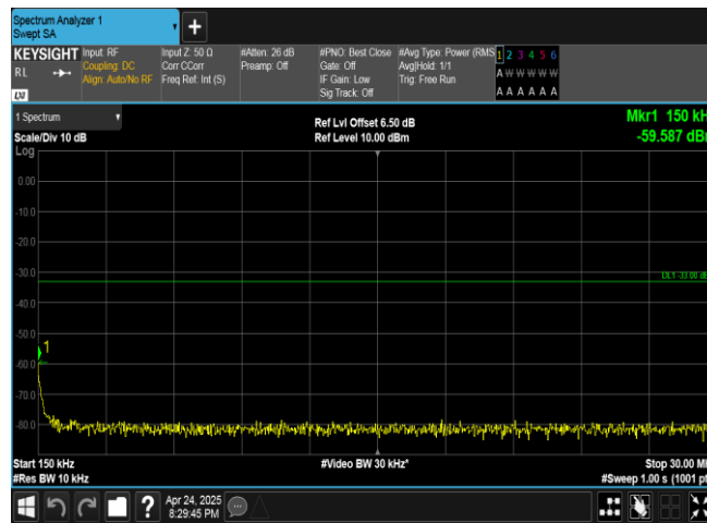
Band4-1513-1-0.15~30MHz-PASS
