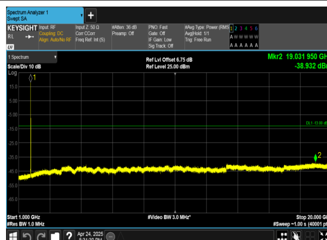
Band4-1413-2-1000~20000MHz-PASS
