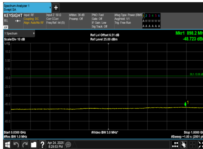
Band4-1513-1-30~1000MHz-PASS
