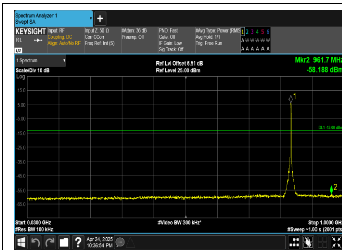
Band5-4182-30~1000MHz-PASS
