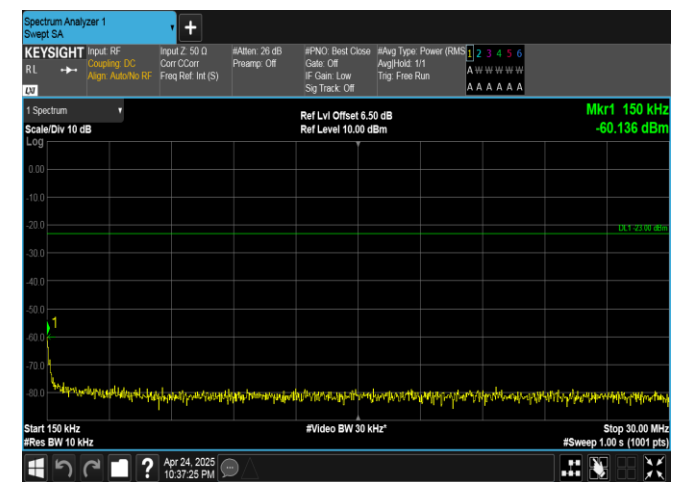
Band5-4233-0.15~30MHz-PASS
