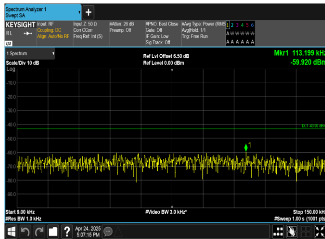
Band2-9400-3-0.009~0.15MHz-PASS
