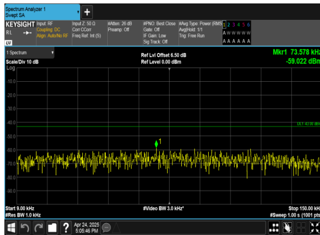
Band2-9538-2-0.009~0.15MHz-PASS
