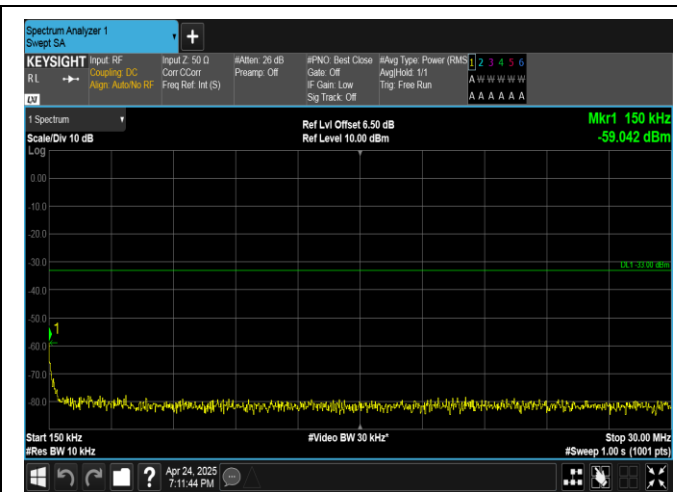
Band4-1312-0.15~30MHz-PASS
