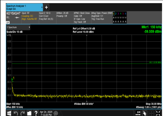
Band4-1413-0.15~30MHz-PASS
