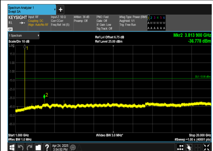
Band2-9538-1000~20000MHz-PASS
