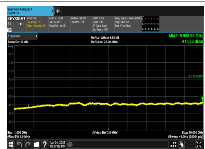
Band5-4182-1000~10000MHz-PASS
