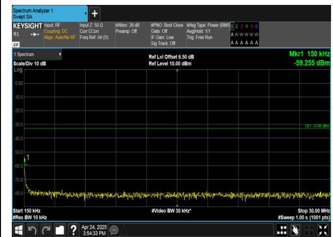
Band2-9538-0.15~30MHz-PASS
