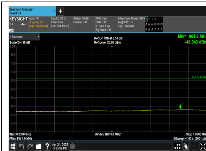
Band2-9400-30~1000MHz-PASS
