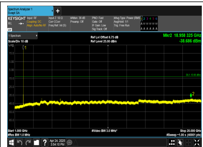
Band2-9400-1000~20000MHz-PASS
