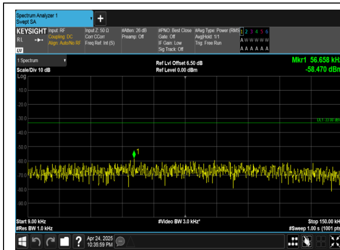
Band5-4132-0.009~0.15MHz-PASS
