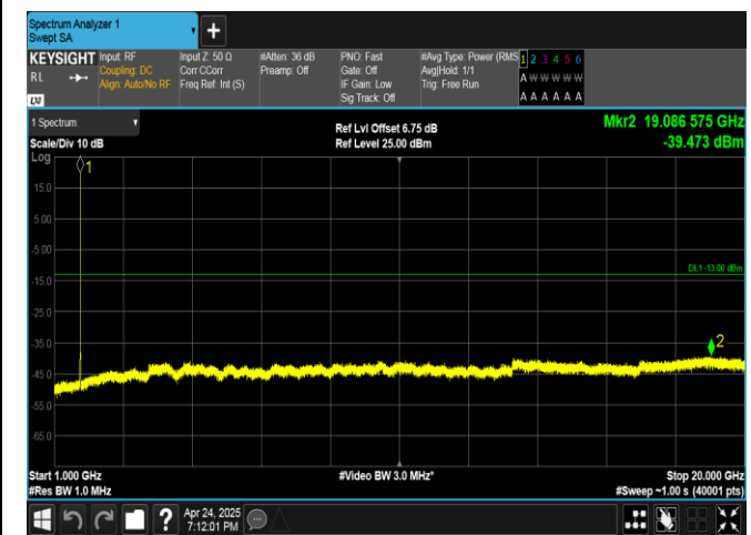
Band4-1312-1000~20000MHz-PASS
