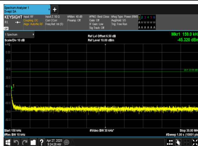
EGPRS850-251-8-0.15~30MHz-PASS
