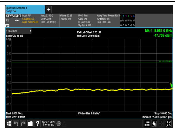
EGPRS850-128-8-1000~10000MHz-PASS
