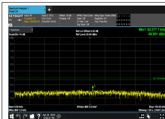
GPRS1900-512-0-0.009~0.15MHz-PASS
