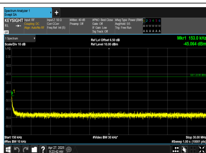
EGPRS850-190-8-0.15~30MHz-PASS
