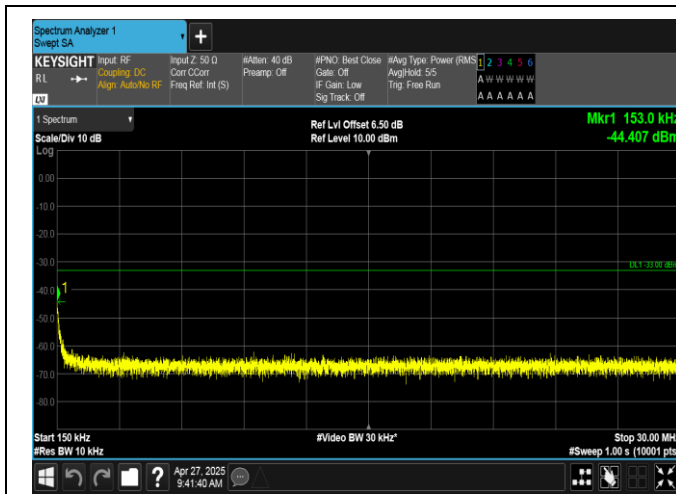
EGPRS1900-512-2-0.15~30MHz-PASS
