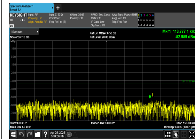
GPRS850-190-5-0.009~0.15MHz-PASS
