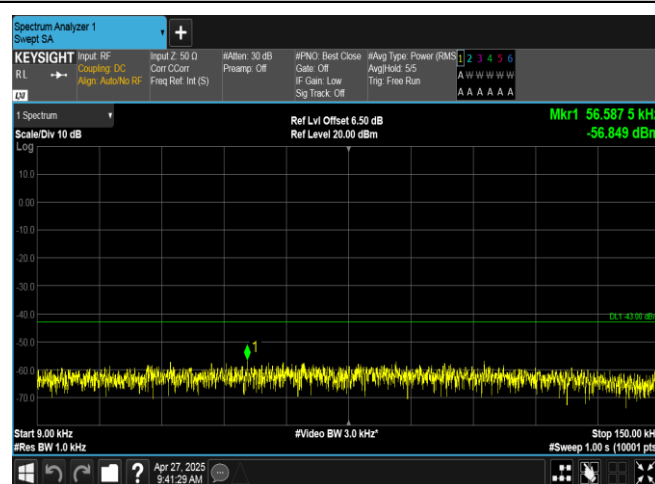
EGPRS1900-512-2-0.009~0.15MHz-PASS
