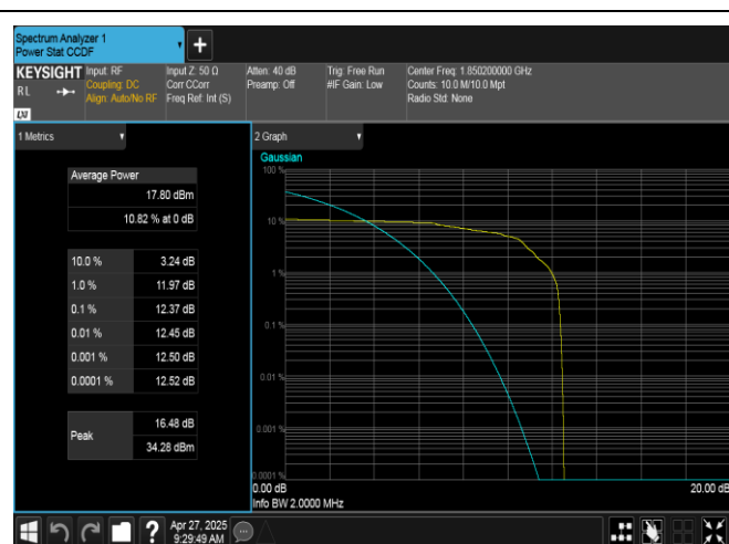
EGPRS1900-512-2-PASS
