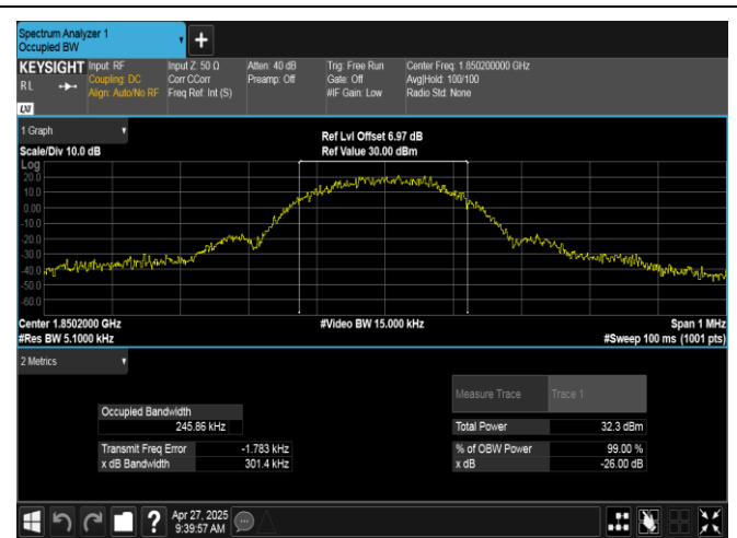
EGPRS1900-512-2-PASS
