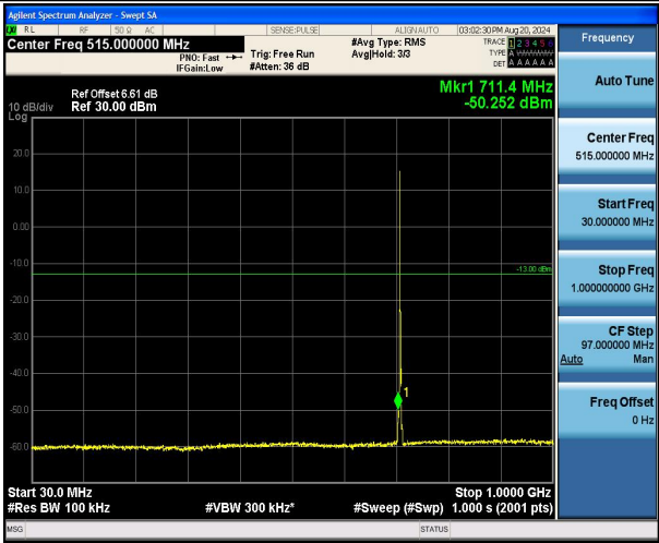
Band12_1.4MHz_16QAM_23173_1RB#0_30~1000_30~1000
