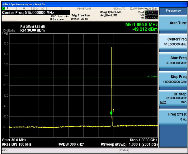
Band12_1.4MHz_QPSK_23017_1RB#0_30~1000_30~1000
