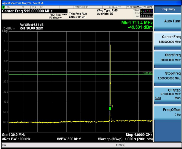
Band12_1.4MHz_QPSK_23173_1RB#0_30~1000_30~1000
