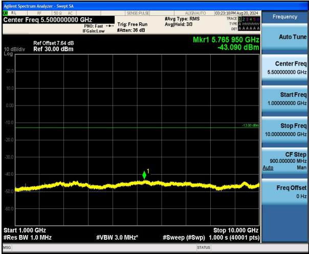
Band12_3MHz_QPSK_23025_1RB#0_1000~10000_1000~10000
