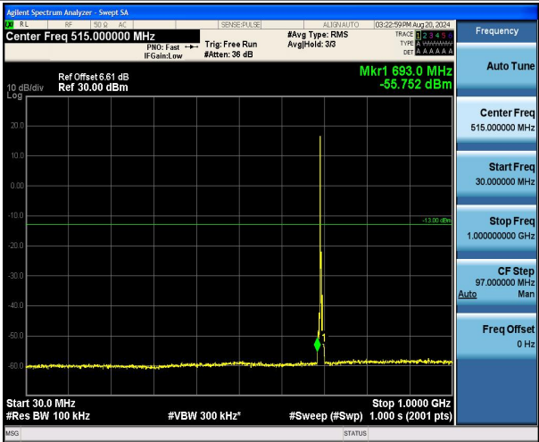
Band12_3MHz_QPSK_23025_1RB#0_30~1000_30~1000
