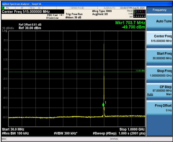
Band12_1.4MHz_QPSK_23095_1RB#0_30~1000_30~1000
