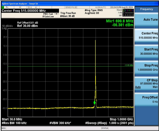
Band12_3MHz_QPSK_23095_1RB#0_30~1000_30~1000
