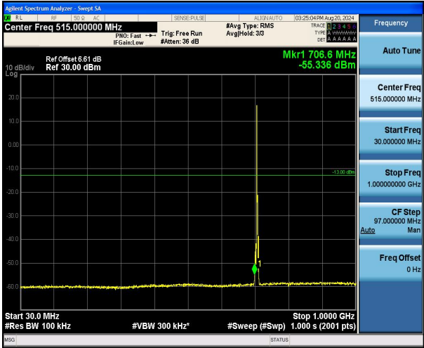
Band12_3MHz_QPSK_23165_1RB#0_30~1000_30~1000
