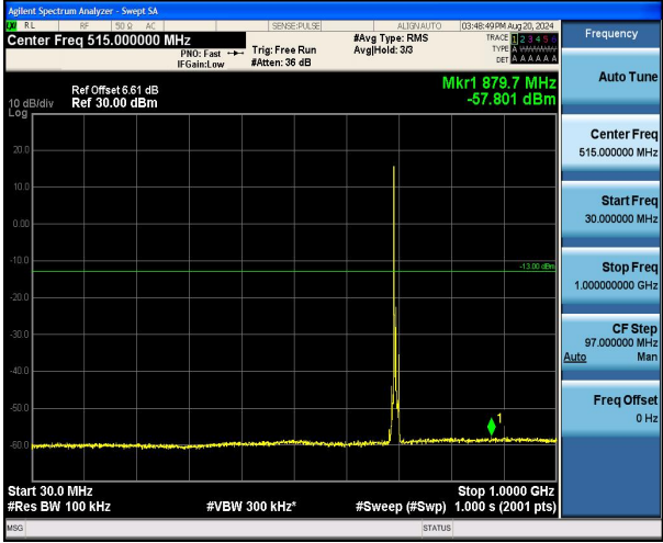
Band12_5MHz_16QAM_23035_1RB#0_30~1000_30~1000
