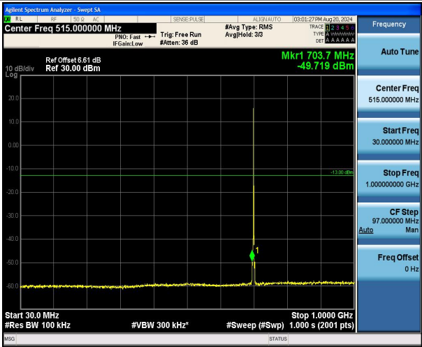
Band12_1.4MHz_16QAM_23095_1RB#0_30~1000_30~1000
