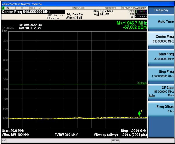
Band7_20MHz_16QAM_21350_1RB#0_30~1000_30~1000
