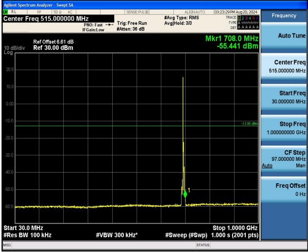
Band12_3MHz_16QAM_23025_1RB#0_30~1000_30~1000
