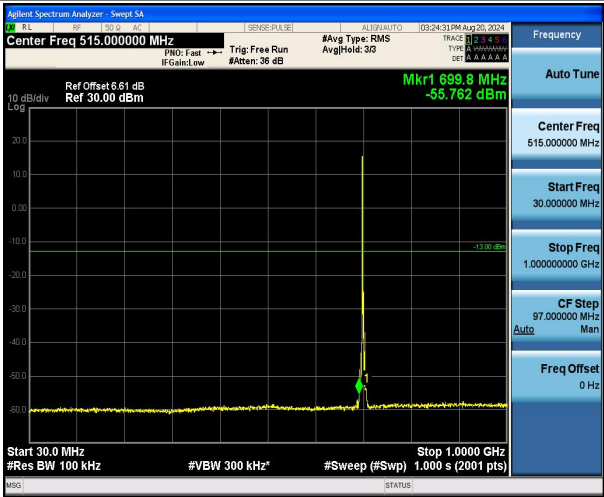
Band12_3MHz_16QAM_23095_1RB#0_30~1000_30~1000
