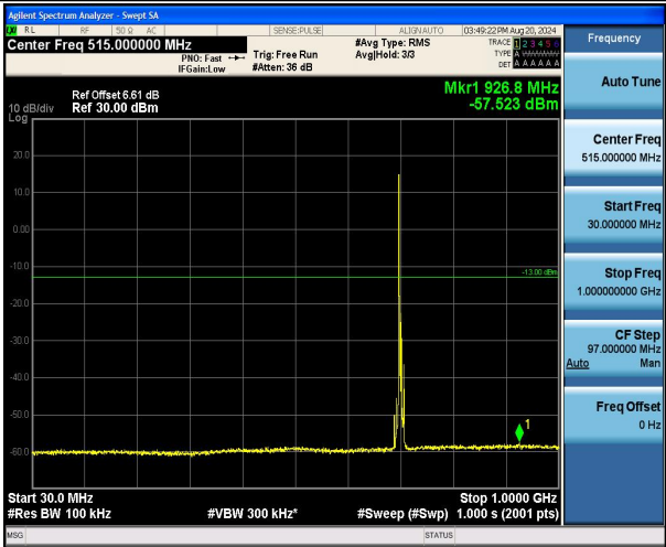
Band12_5MHz_QPSK_23095_1RB#0_30~1000_30~1000
