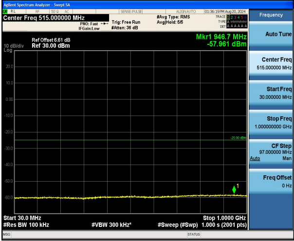
Band7_5MHz_QPSK_21425_1RB#0_30~1000_30~1000
