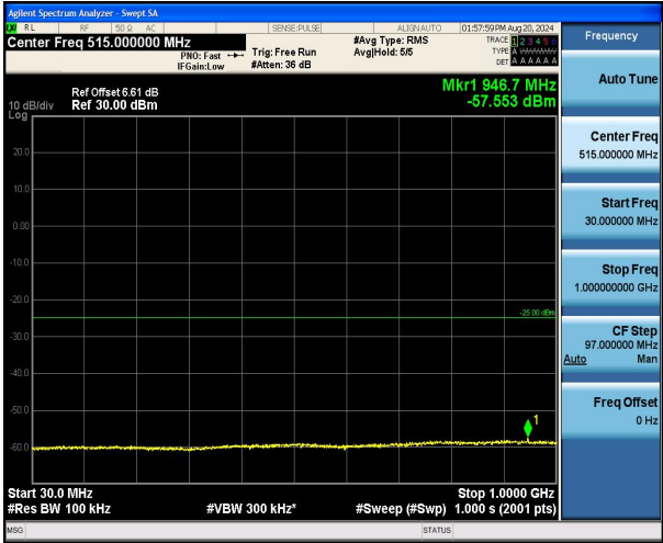
Band7_10MHz_QPSK_21400_1RB#0_30~1000_30~1000
