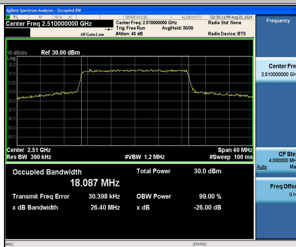
Band7-20MHz-16QAM-20850-100RB#0-PASS
