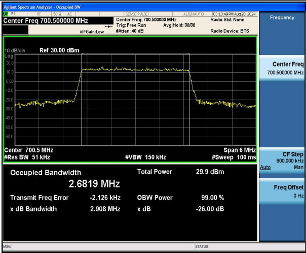
Band12-3MHz-16QAM-23025-15RB#0-PASS
