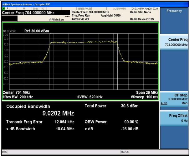
Band12-10MHz-16QAM-23060-50RB#0-PASS
