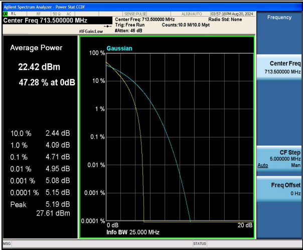
Band12-5MHz-QPSK-23155-25RB#0-PASS
