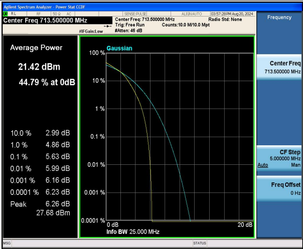
Band12-5MHz-16QAM-23155-25RB#0-PASS
