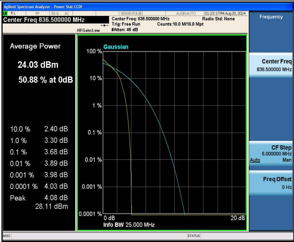
Band5-10MHz-QPSK-20525-1RB#0-PASS
