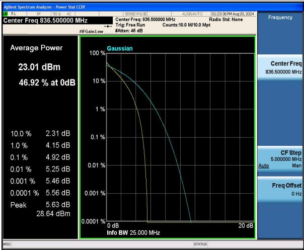
Band5-10MHz-QPSK-20525-50RB#0-PASS
