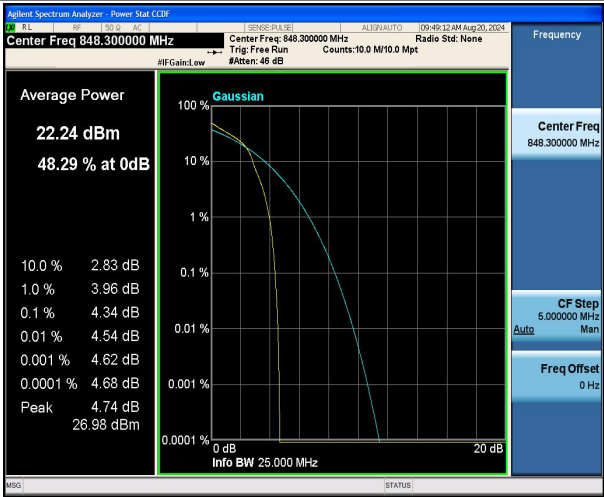
Band5-1.4MHz-16QAM-20643-1RB#0-PASS
