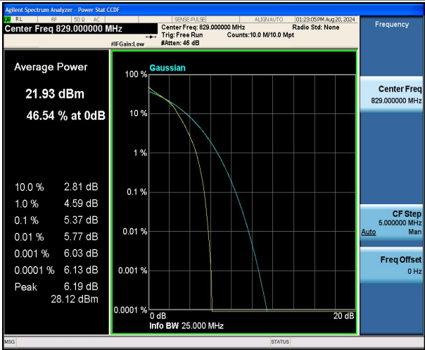
Band5-10MHz-16QAM-20450-50RB#0-PASS
