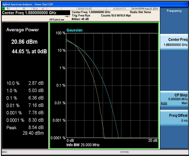
Band2-20MHz-16QAM-18900-100RB#0-PASS
