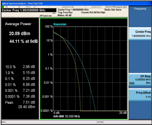
Band2-15MHz-16QAM-19125-75RB#0-PASS
