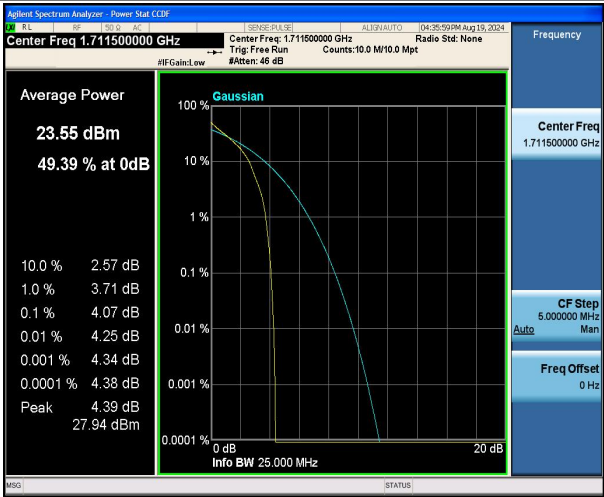
Band4-3MHz-QPSK-19965-1RB#0-PASS
