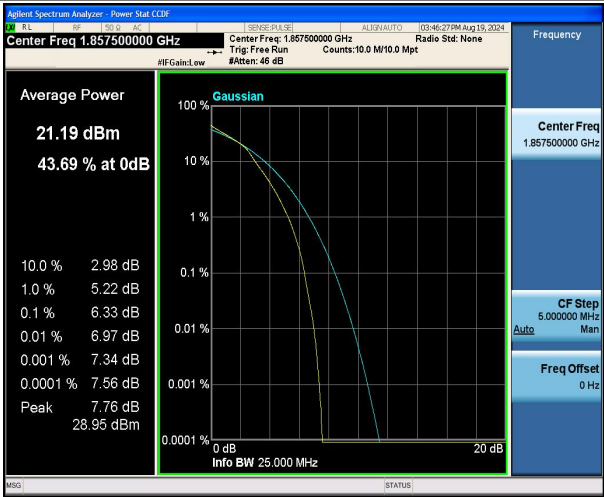
Band2-15MHz-16QAM-18675-75RB#0-PASS
