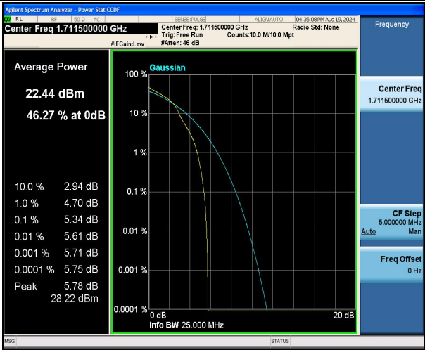
Band4-3MHz-16QAM-19965-1RB#0-PASS
