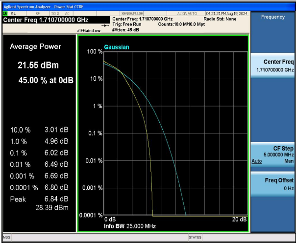
Band4-1.4MHz-16QAM-19957-6RB#0-PASS
