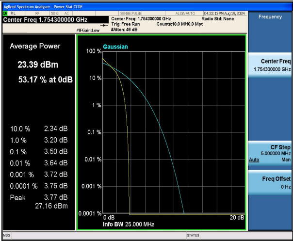
Band4-1.4MHz-QPSK-20393-1RB#0-PASS
