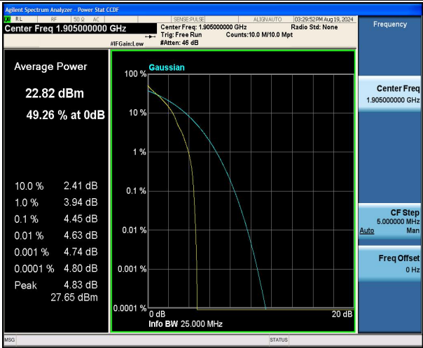
Band2-10MHz-QPSK-19150-1RB#0-PASS
