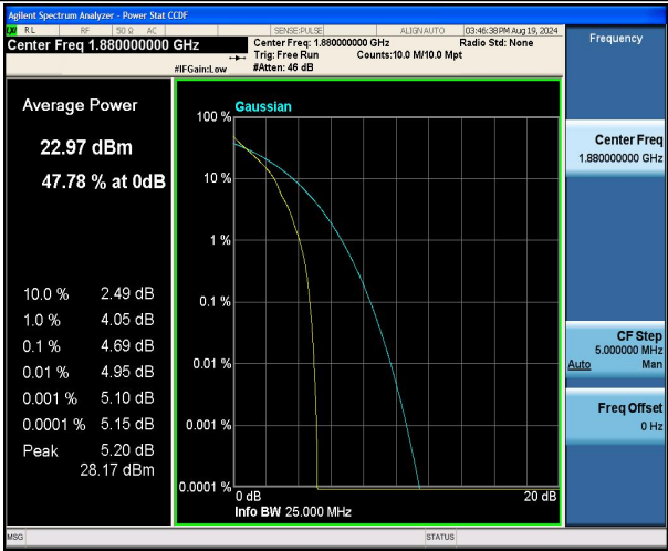
Band2-15MHz-QPSK-18900-1RB#0-PASS
