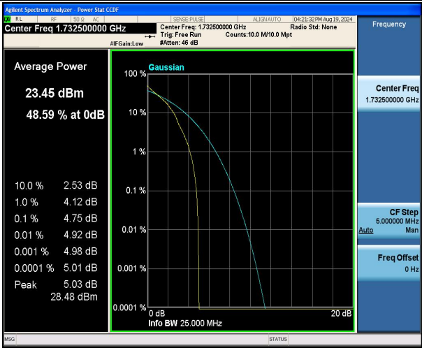
Band4-1.4MHz-QPSK-20175-1RB#0-PASS
