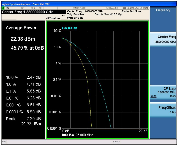
Band2-15MHz-QPSK-18900-75RB#0-PASS
