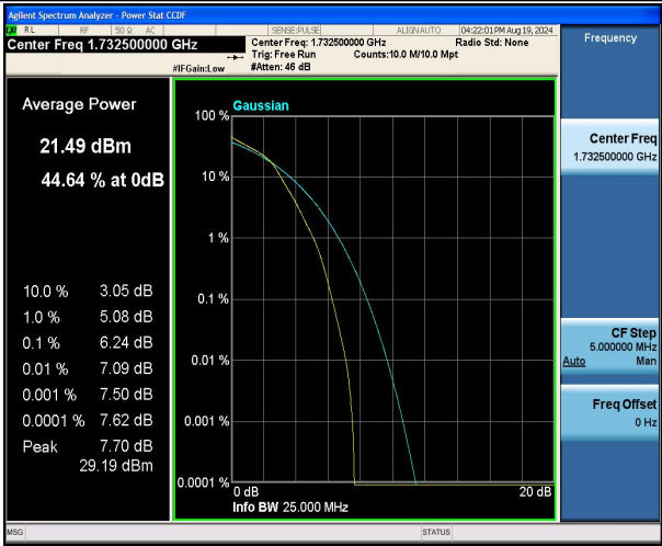
Band4-1.4MHz-16QAM-20175-6RB#0-PASS
