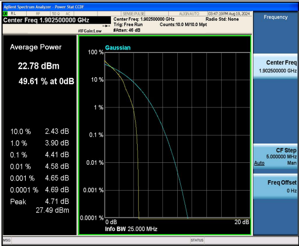
Band2-15MHz-QPSK-19125-1RB#0-PASS
