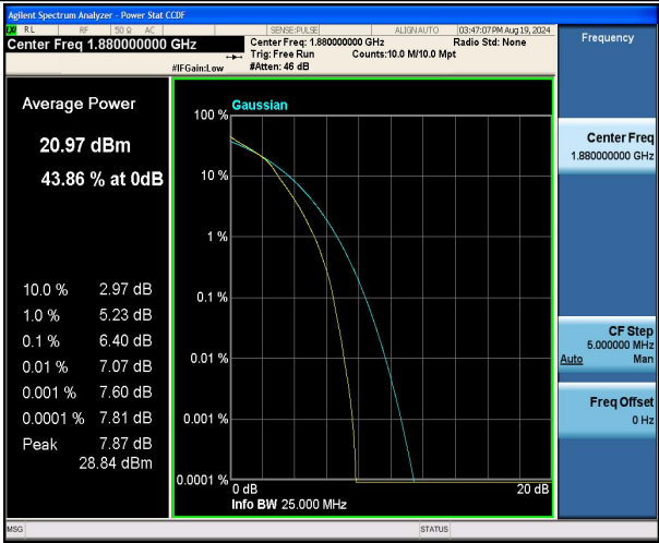
Band2-15MHz-16QAM-18900-75RB#0-PASS
