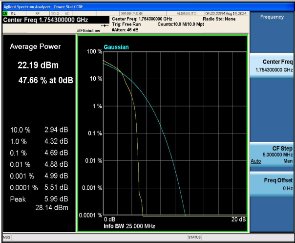
Band4-1.4MHz-16QAM-20393-1RB#0-PASS
