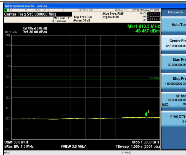
Band2-9262-30~1000MHz-PASS
