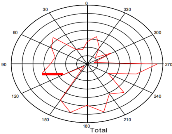
Gain: (dBi)
