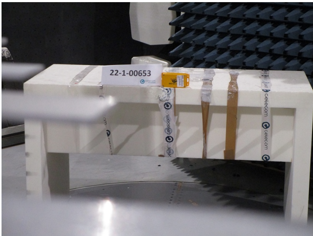
Fig. Mea.: 2 : Measurement in the semi anechoic chamber
