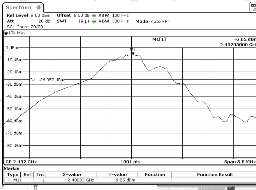
1_Reference_Level_NVNT_ANT1_1Mbps_2402
