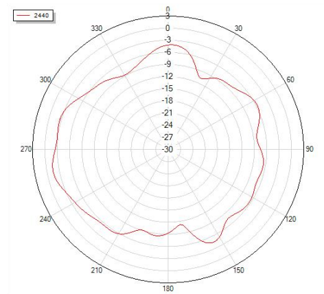
Phi=0 freq=2440MHz
