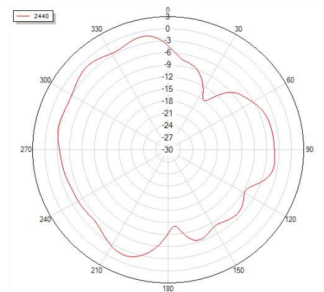
Phi=90 freq=2440MHz
