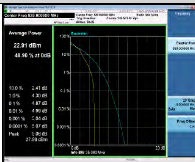
N5-20MHz-QPSK-167800-100RB#0
