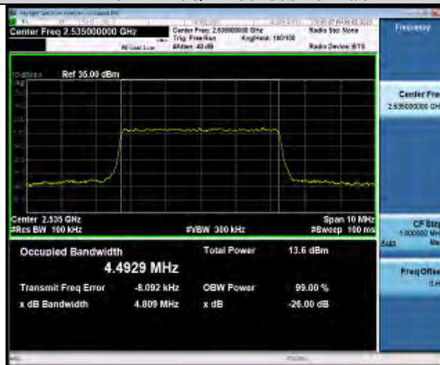
N7-5MHz-64QAM-507000-25RB#0
