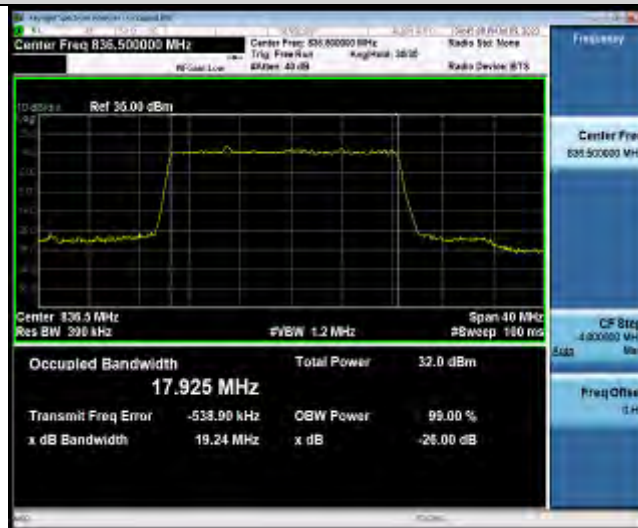
N5-20MHz-256QAM-167300-100RB#0
