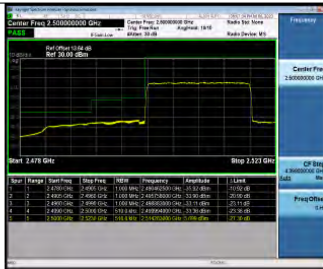
N7-20MHz-QPSK-512000-1RB#99
