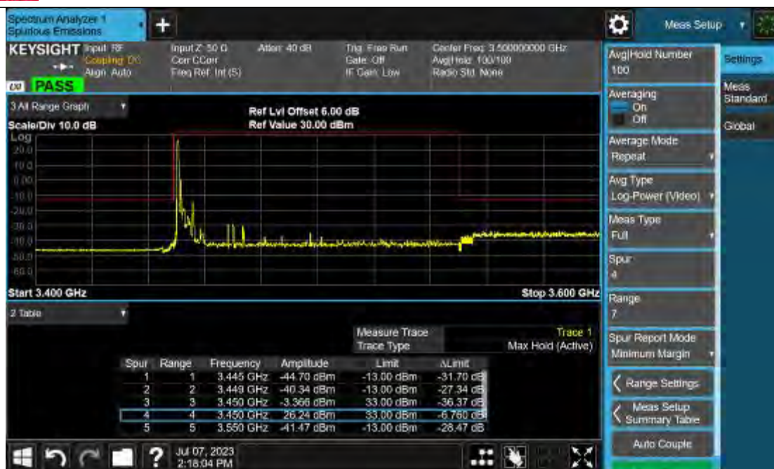
Band42-5MHz-16QAM-42115-25RB#0
