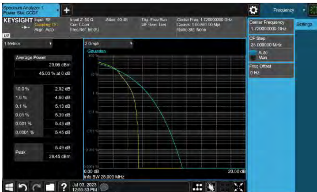
Band66-20MHz-16QAM-132072-100RB#0
