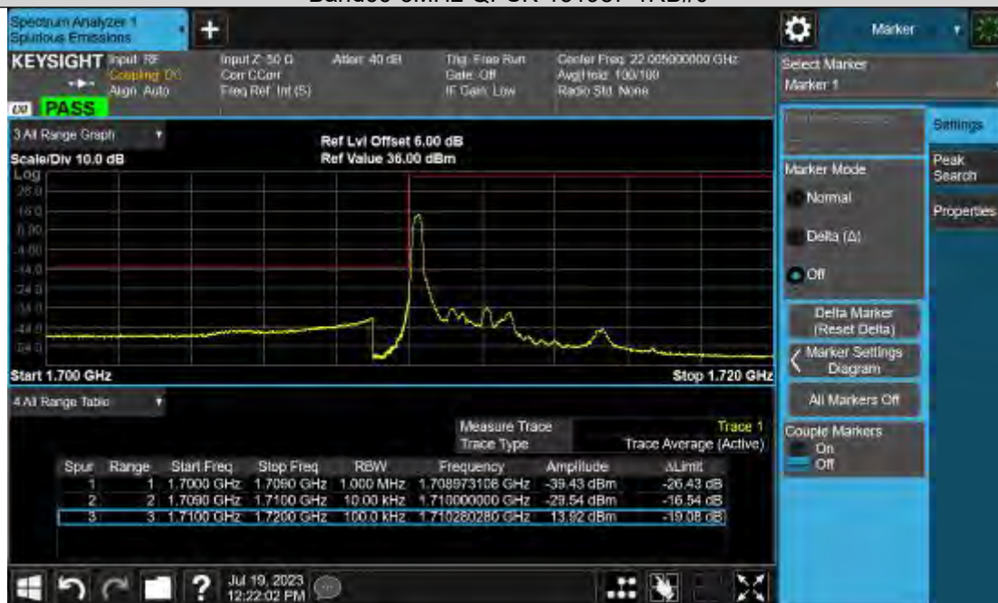
Band66-3MHz-QPSK-131987-15RB#0
