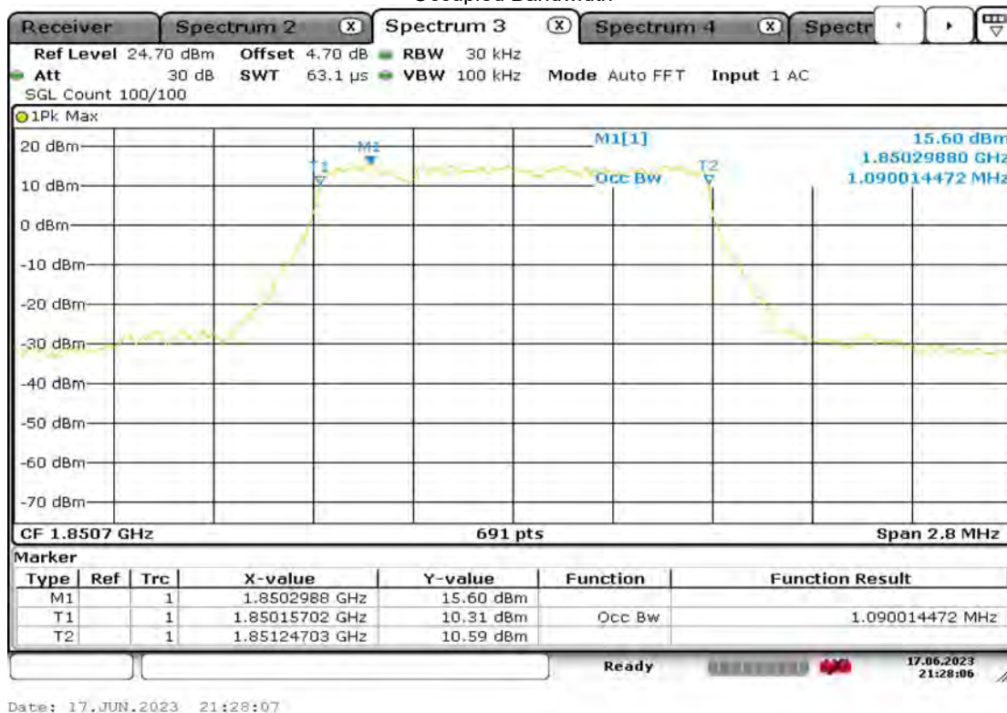
Band25-1.4MHz-QPSK-26047-6RB#0
