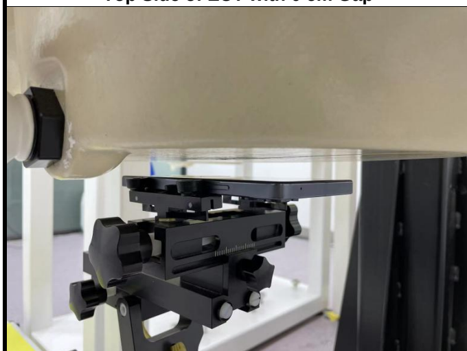
Front Face of EUT with 1.4 cm Gap
