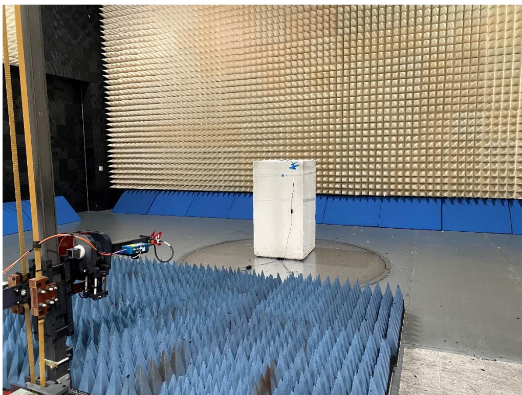
Figure 6: FCC 15.247 RSE, 1GHz – 18GHz
