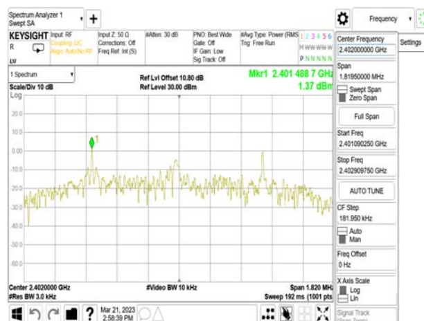
PSD_BLE 2M_LowCH00-2402MHz
