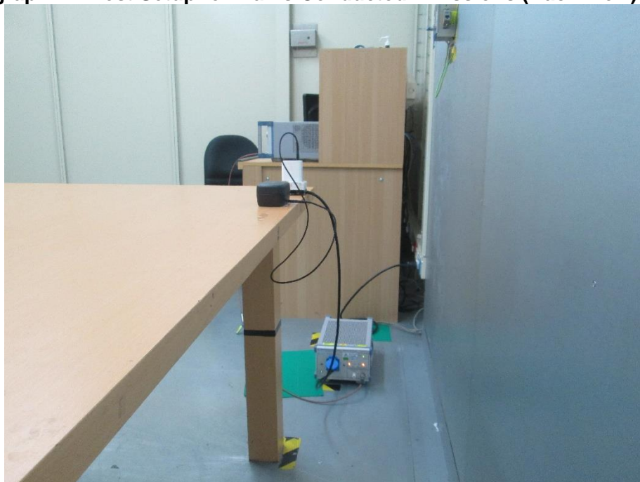
Photograph 11: Test Setup for Mains Conducted Emissions (Back View)
