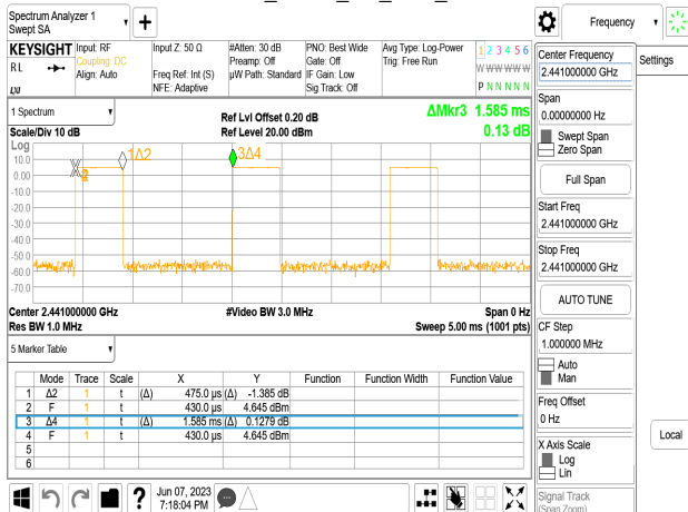
Dwell Time_GFSK_1M_DH3_2441MHz
