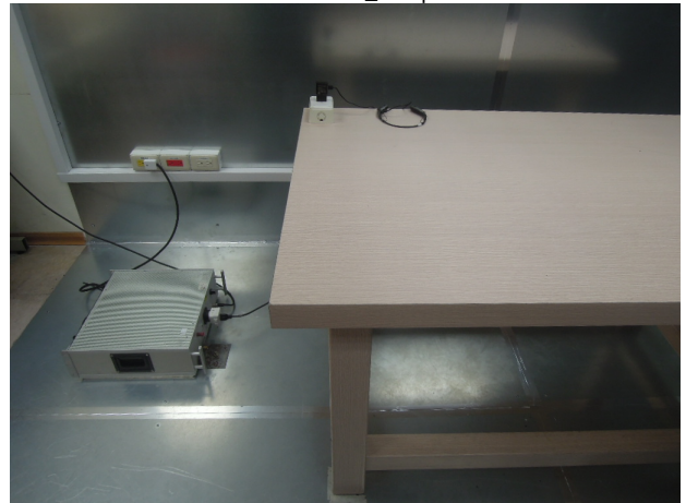
Conduction_Setup
