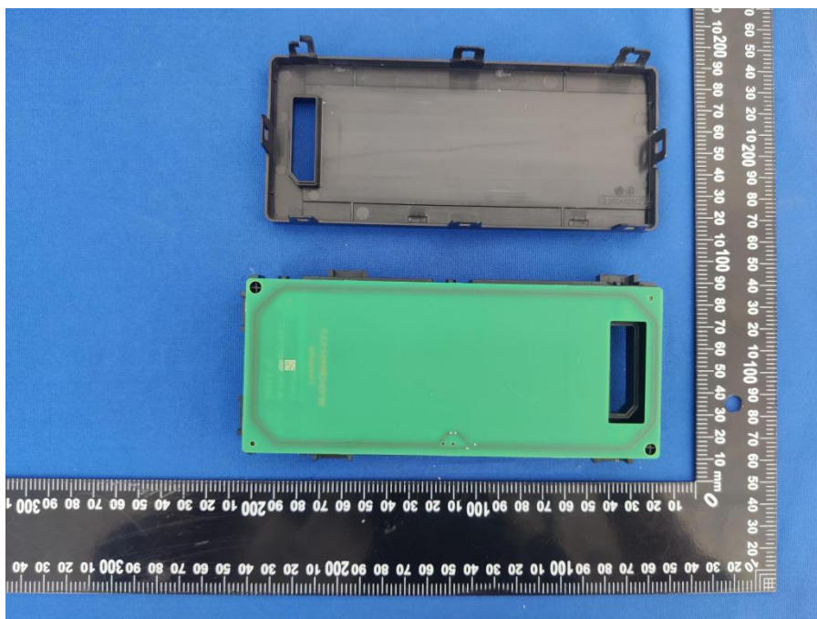
EUT UNCOVER VIEW 1_WCM_NFC_Int(fanless)
