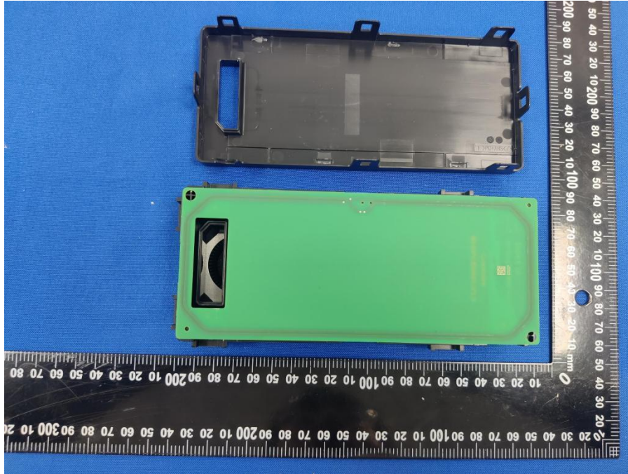
EUT UNCOVER VIEW 1_WCM_NFC_Int(Have a fan)
