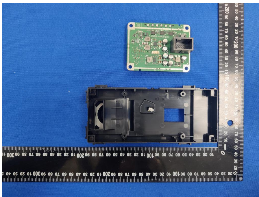
EUT UNCOVER VIEW 4_WCM_NFC_Int(Have a fan)
