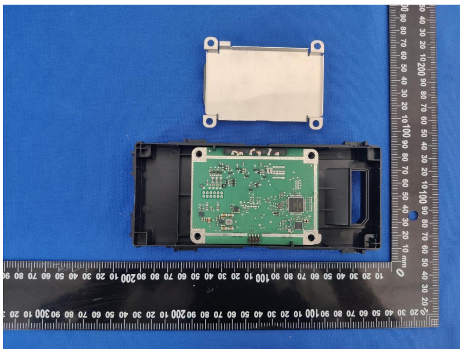
EUT UNCOVER VIEW 3_WCM_NFC_Int(fanless)
