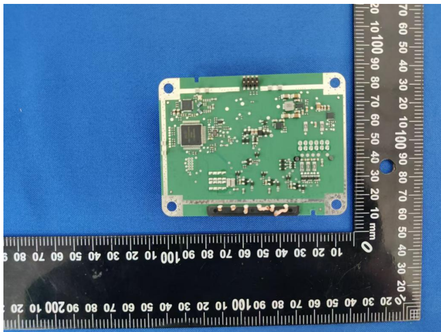
MAIN BOARD REAR VIEW_WCM_NFC_Int(Have a fan)
