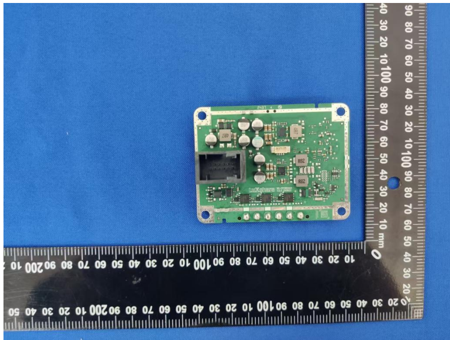
MAIN BOARD TOP VIEW_WCM_NFC_Int(Have a fan)
