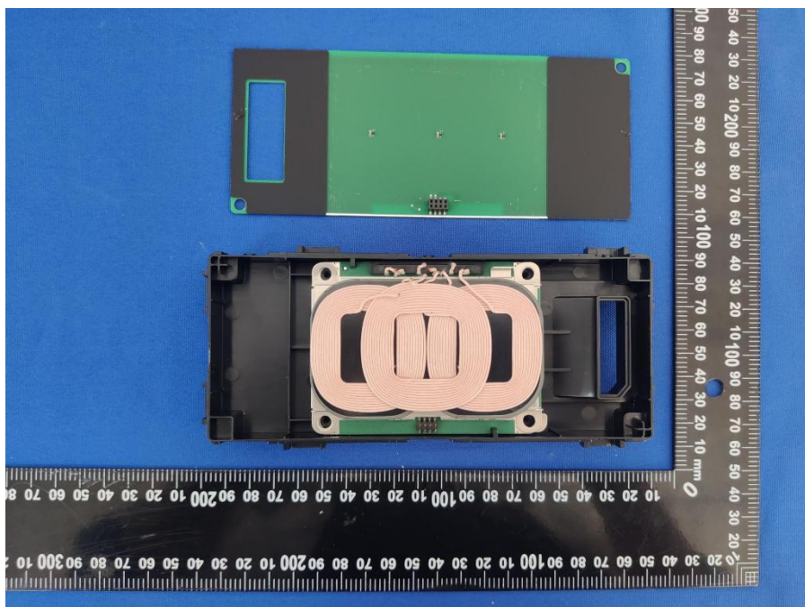
EUT UNCOVER VIEW 2_WCM_NFC_Int(fanless)
