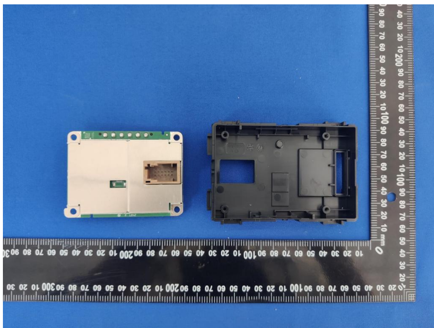
EUT UNCOVER VIEW 4_WCM(fanless)
