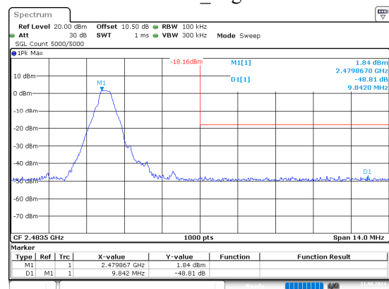
GFSK_High
