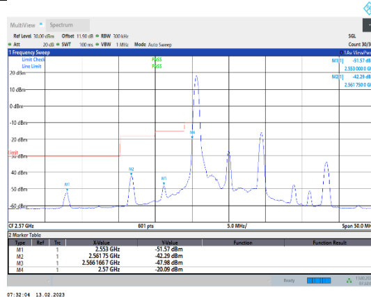
Band38-10MHz-16QAM-37800-1RB#0
