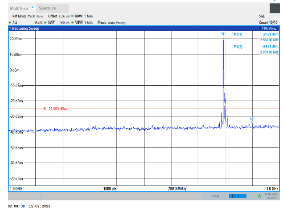
Band41-15MHz-64QAM-40620-1RB#0-Range2:1000~3000MHz
