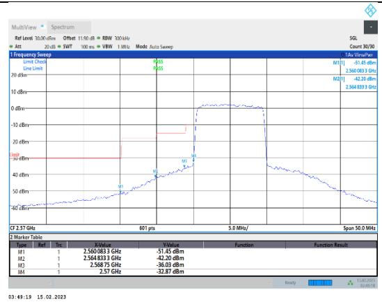
Band38-10MHz-64QAM-37800-50RB#0
