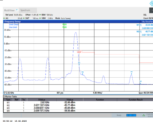
Band38-20MHz-64QAM-38150-1RB#99
