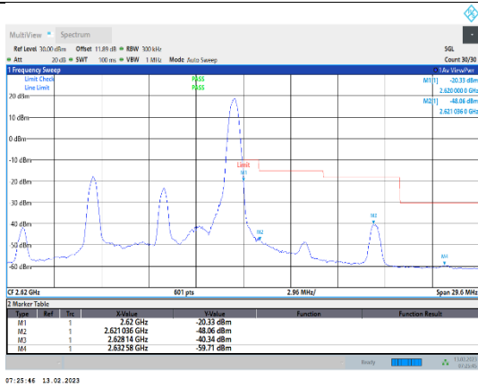
Band38-10MHz-16QAM-38200-1RB#49
