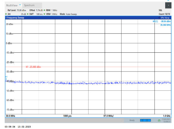
Band41-20MHz-16QAM-40620-1RB#0-Range1:30~1000MHz
