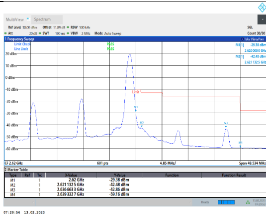
Band38-20MHz-16QAM-38150-1RB#99
