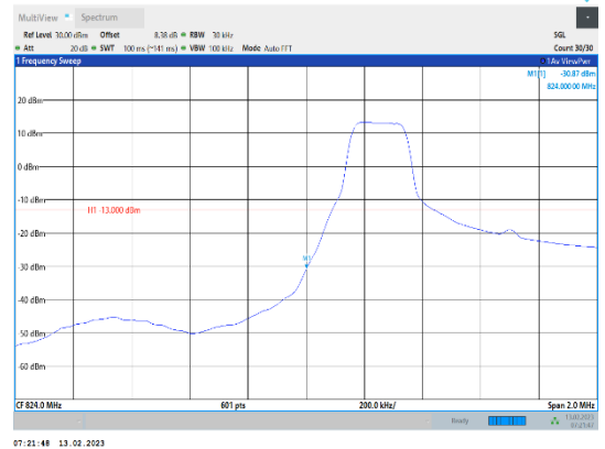
Band5-1.4MHz-16QAM-20407-1RB#0
