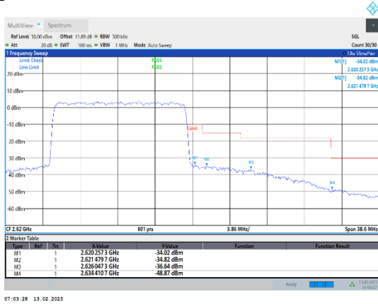
Band38-15MHz-16QAM-38175-75RB#0
