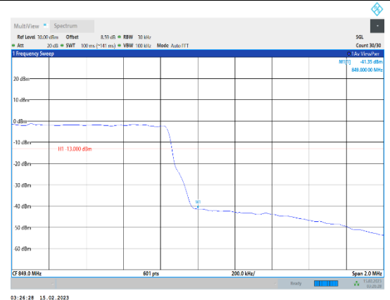
Band5-1.4MHz-64QAM-20643-6RB#0
