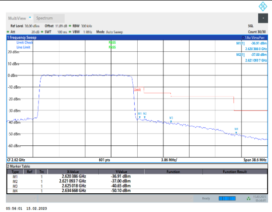
Band38-15MHz-64QAM-38175-75RB#0
