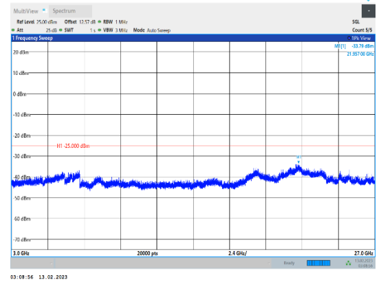
Band41-20MHz-16QAM-40620-1RB#0-Range3:3000~27000MHz
