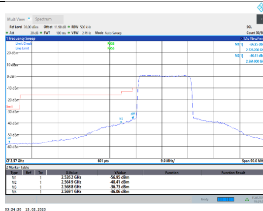
Band38-20MHz-64QAM-37850-100RB#0
