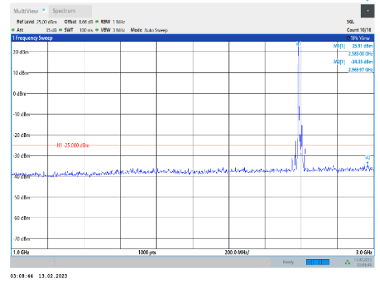
Band41-20MHz-16QAM-40620-1RB#0-Range2:1000~3000MHz
