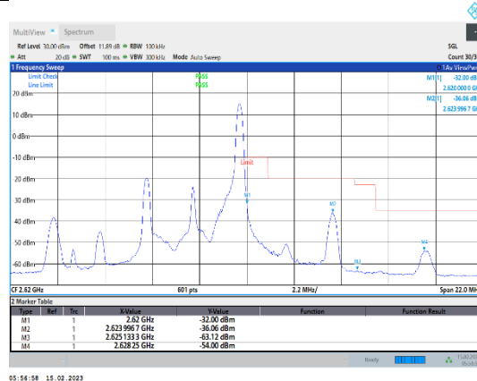
Band38-5MHz-64QAM-38225-1RB#24
