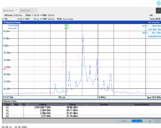
Band38-5MHz-64QAM-37775-1RB#0
