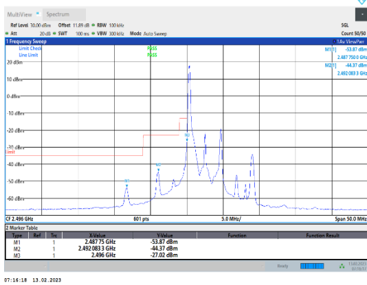
Band41-5MHz-QPSK-39675-1RB#0
