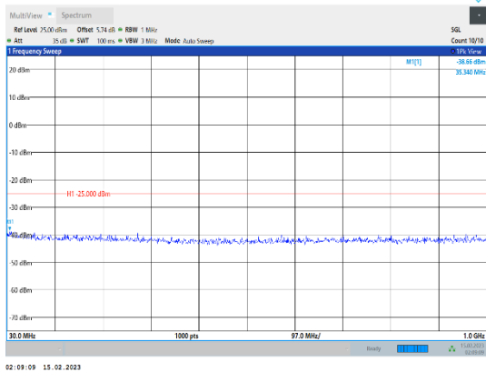
Band41-15MHz-64QAM-41515-1RB#0-Range1:30~1000MHz
