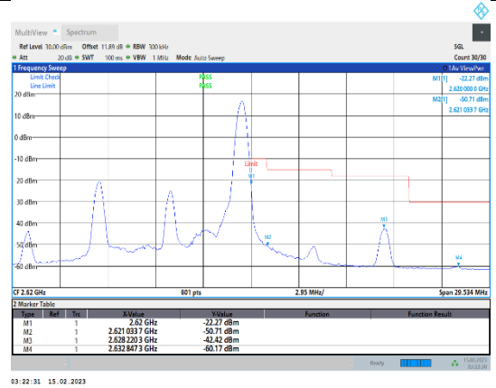
Band38-10MHz-64QAM-38200-1RB#49
