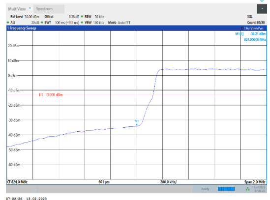
Band5-1.4MHz-16QAM-20407-6RB#0
