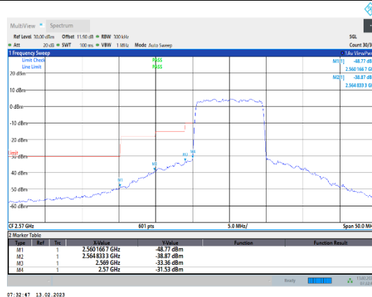
Band38-10MHz-16QAM-37800-50RB#0
