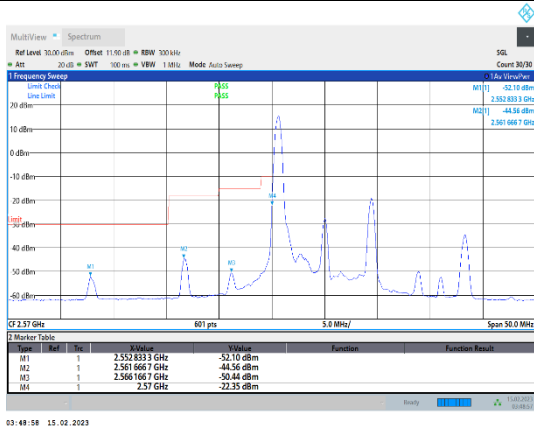
Band38-10MHz-64QAM-37800-1RB#0
