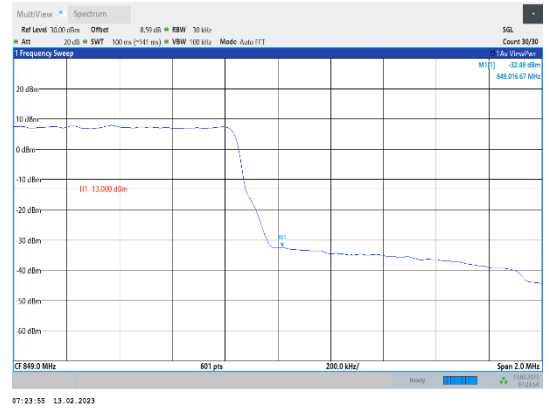
Band5-1.4MHz-QPSK-20643-6RB#0
