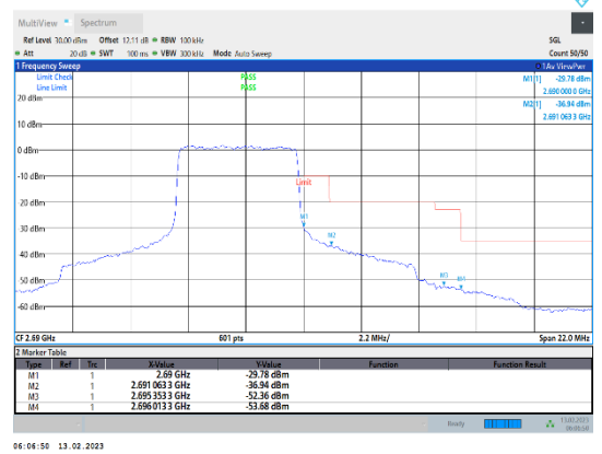
Band41-5MHz-QPSK-41565-25RB#0
