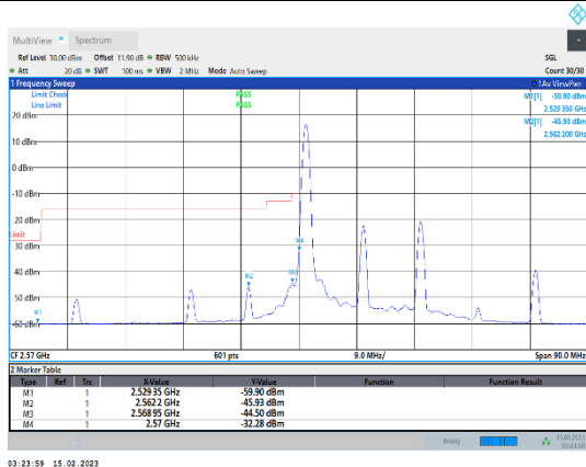
Band38-20MHz-64QAM-37850-1RB#0
