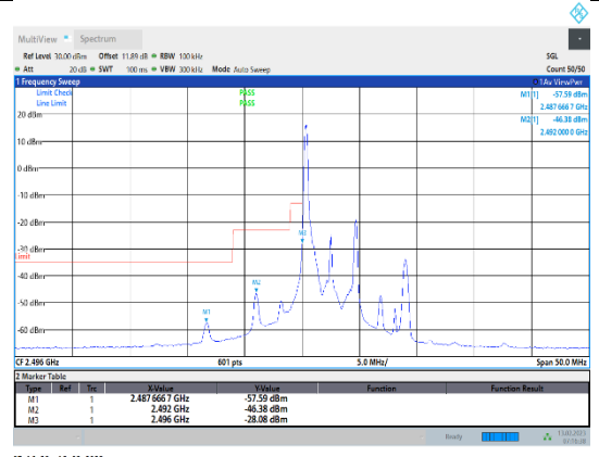
Band41-5MHz-16QAM-39675-1RB#0
