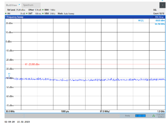
Band41-15MHz-64QAM-40620-1RB#0-Range1:30~1000MHz
