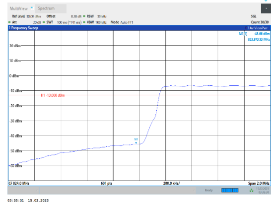
Band5-1.4MHz-64QAM-20407-6RB#0
