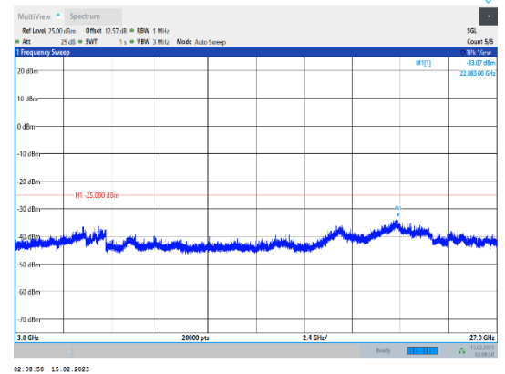
Band41-15MHz-64QAM-40620-1RB#0-Range3:3000~27000MHz
