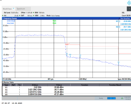
Band38-20MHz-16QAM-38150-100RB#0
