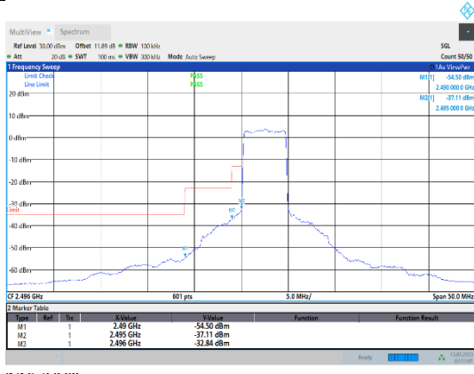
Band41-5MHz-QPSK-39675-25RB#0
