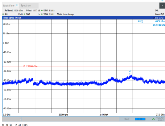
Band41-15MHz-64QAM-41515-1RB#0-Range3:3000~27000MHz
