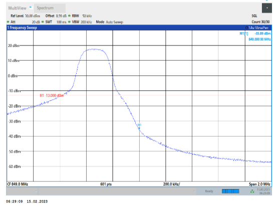
Band5-5MHz-64QAM-20625-1RB#24
