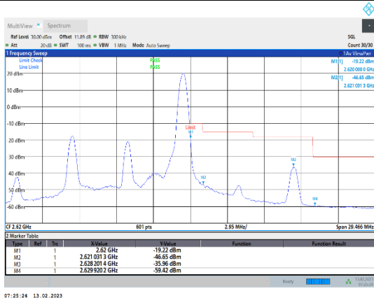
Band38-10MHz-QPSK-38200-1RB#49
