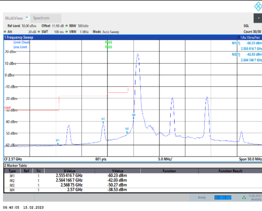
Band38-15MHz-64QAM-37825-1RB#0
