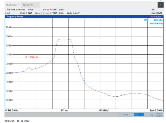
Band5-1.4MHz-64QAM-20643-1RB#5
