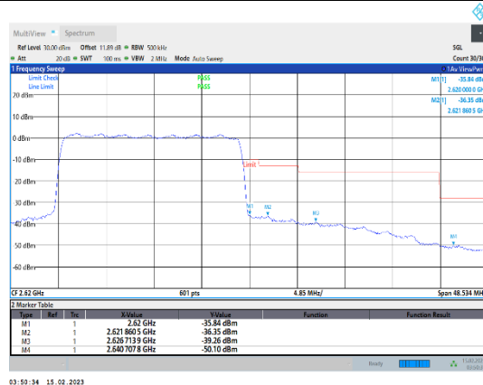
Band38-20MHz-64QAM-38150-100RB#0
