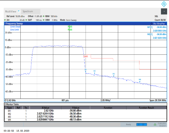
Band38-10MHz-64QAM-38200-50RB#0
