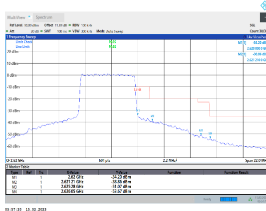
Band38-5MHz-64QAM-38225-25RB#0
