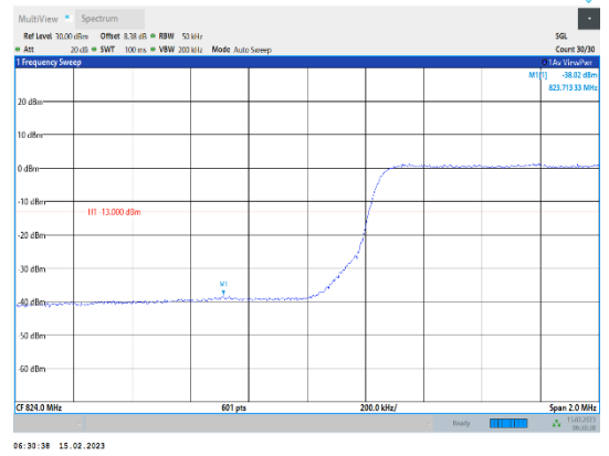
Band5-5MHz-64QAM-20425-25RB#0
