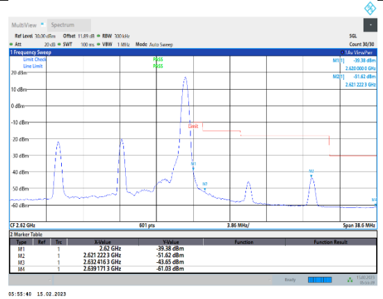
Band38-15MHz-64QAM-38175-1RB#74
