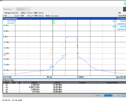
Band38-5MHz-64QAM-37775-25RB#0
