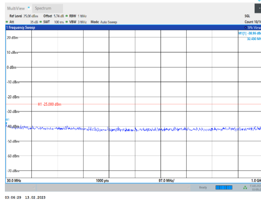
Band41-20MHz-QPSK-39750-1RB#0-Range1:30~1000MHz
