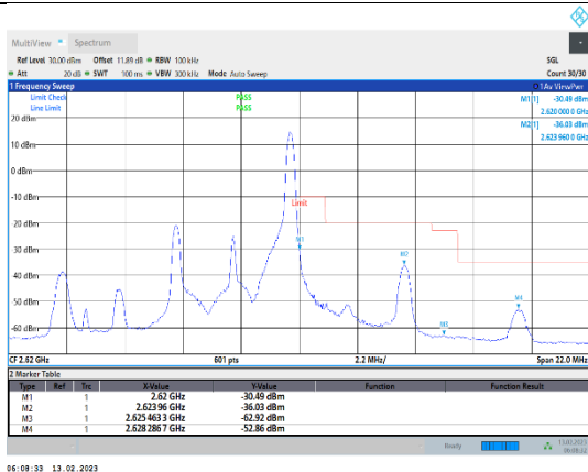
Band38-5MHz-16QAM-38225-1RB#24
