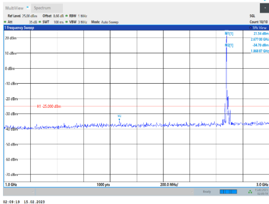
Band41-15MHz-64QAM-41515-1RB#0-Range2:1000~3000MHz
