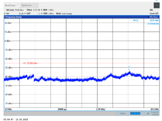
Band38-20MHz-64QAM-37850-1RB#0-Range3:3000~26500MHz
