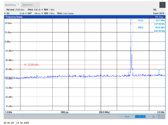
Band38-15MHz-16QAM-37825-1RB#0-Range2:1000~3000MHz
