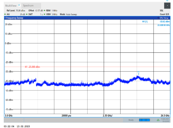
Band38-15MHz-16QAM-37825-1RB#0-Range3:3000~26500MHz
