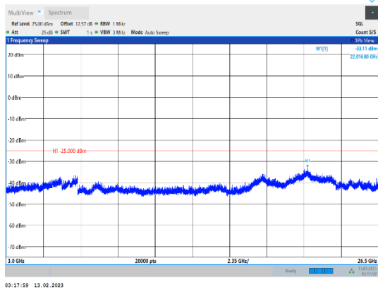
Band38-20MHz-QPSK-38000-1RB#0-Range3:3000~26500MHz
