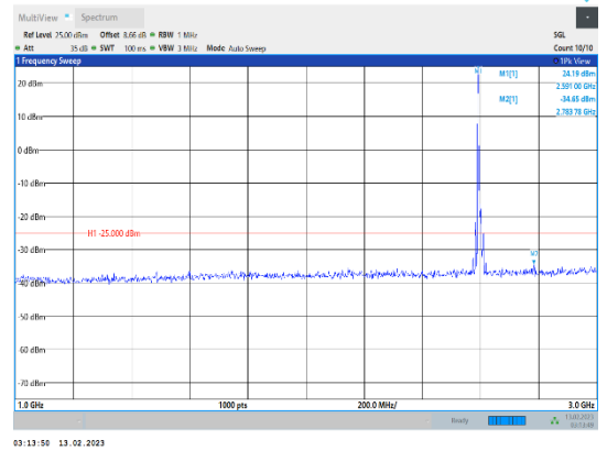
Band38-10MHz-16QAM-38000-1RB#0-Range2:1000~3000MHz
