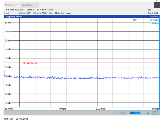
Band38-20MHz-64QAM-37850-1RB#0-Range1:30~1000MHz
