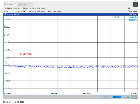
Band41-15MHz-QPSK-40620-1RB#0-Range1:30~1000MHz
