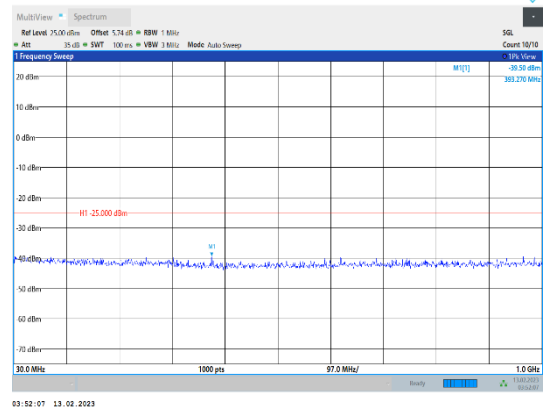
Band41-10MHz-QPSK-41540-1RB#0-Range1:30~1000MHz
