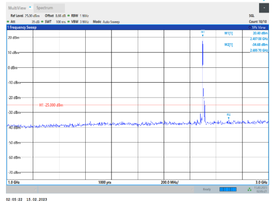
Band41-10MHz-64QAM-39700-1RB#0-Range2:1000~3000MHz
