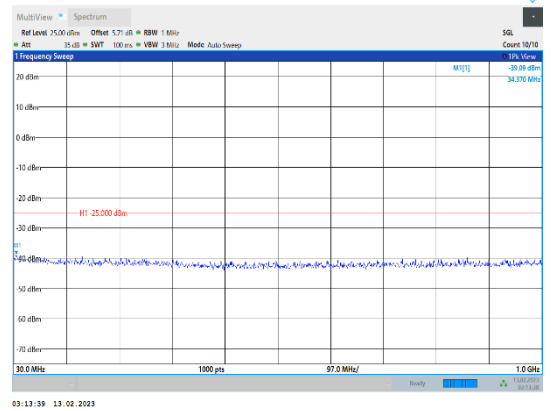
Band38-10MHz-16QAM-38000-1RB#0-Range1:30~1000MHz
