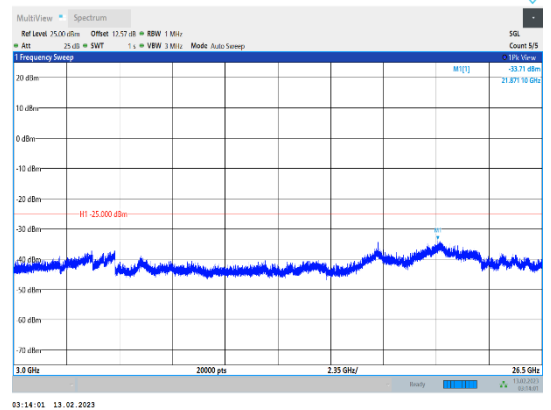
Band38-10MHz-16QAM-38000-1RB#0-Range3:3000~26500MHz
