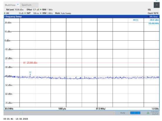
Band38-15MHz-16QAM-37825-1RB#0-Range1:30~1000MHz
