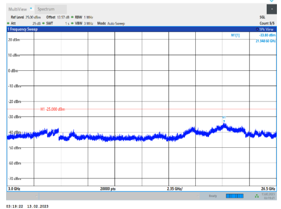
Band38-20MHz-QPSK-38150-1RB#0-Range3:3000~26500MHz
