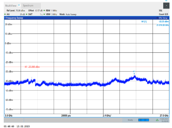
Band41-15MHz-QPSK-40620-1RB#0-Range3:3000~27000MHz
