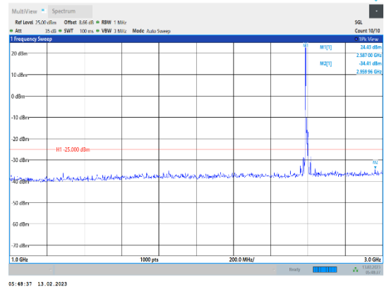
Band41-15MHz-QPSK-40620-1RB#0-Range2:1000~3000MHz
