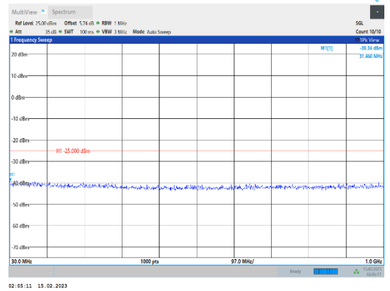
Band41-10MHz-64QAM-39700-1RB#0-Range1:30~1000MHz
