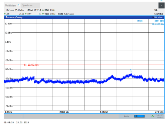
Band41-10MHz-64QAM-39700-1RB#0-Range3:3000~27000MHz
