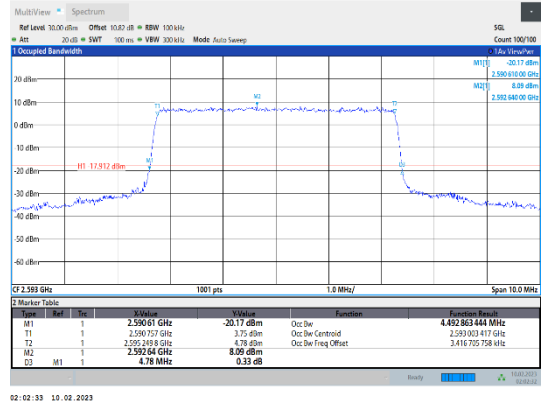
Band41-5MHz-QPSK-40620-25RB#0
