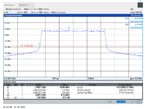
Band41-5MHz-16QAM-41565-25RB#0
