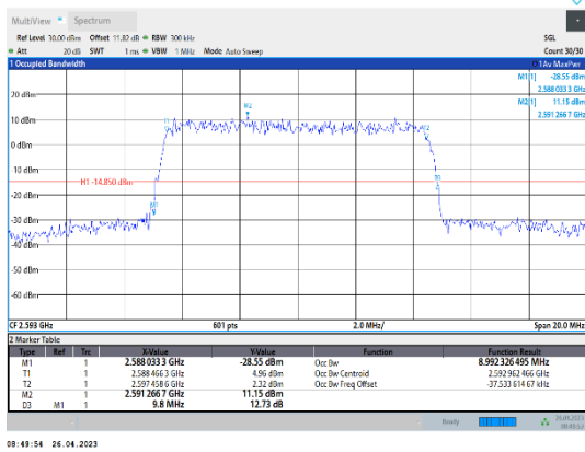
Band41-10MHz-16QAM-40620-50RB#0
