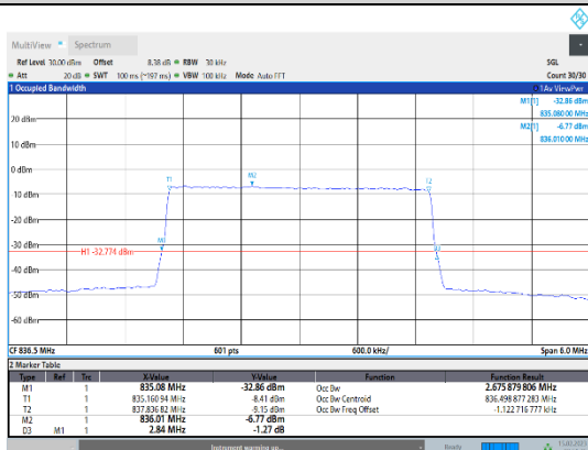
Band5-3MHz-64QAM-20525-15RB#0
