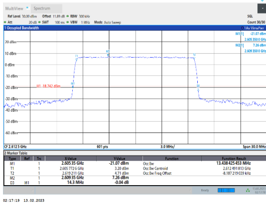
Band38-15MHz-QPSK-38175-75RB#0
