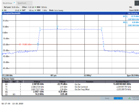
Band38-15MHz-16QAM-38000-75RB#0
