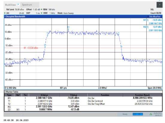
Band41-10MHz-QPSK-40620-50RB#0
