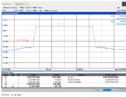
Band41-10MHz-QPSK-40090-50RB#0
