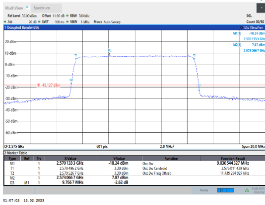
Band38-10MHz-64QAM-37800-50RB#0
