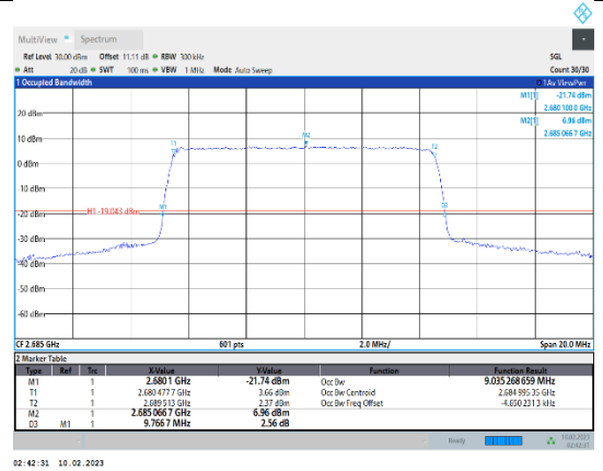
Band41-10MHz-16QAM-41540-50RB#0
