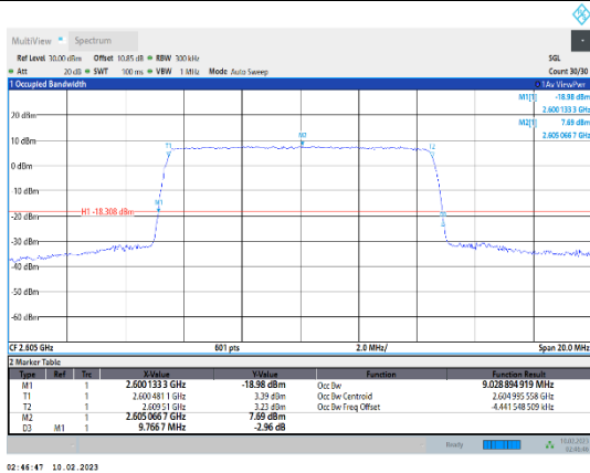
Band41-10MHz-16QAM-40740-50RB#0
