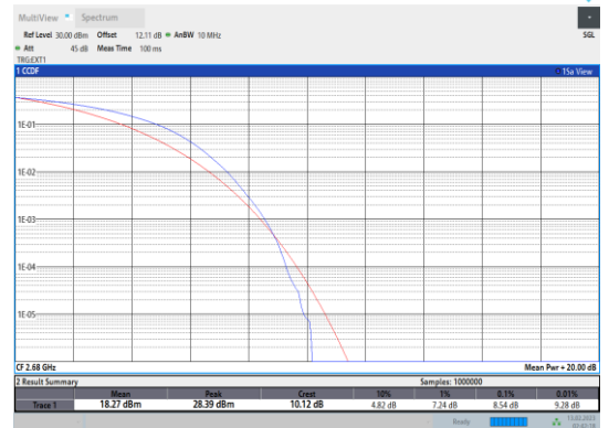
Band41-20MHz-16QAM-41490-100RB#0
