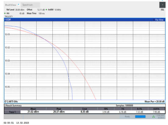
Band41-5MHz-QPSK-41565-25RB#0
