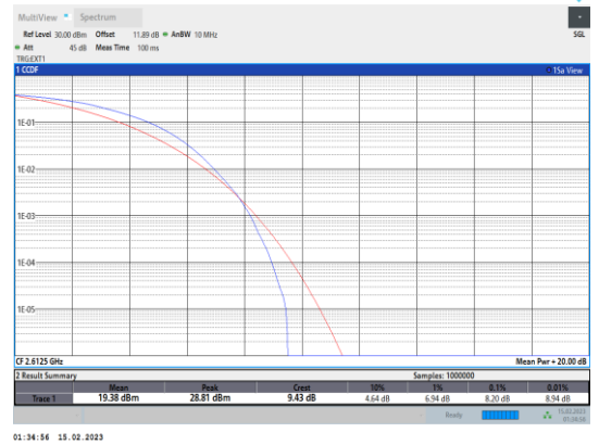
Band38-15MHz-64QAM-38175-75RB#0
