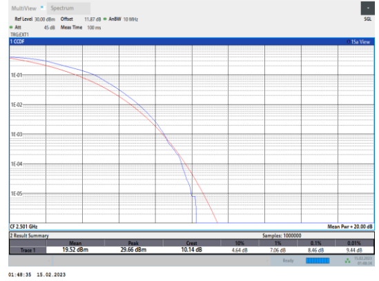
Band41-10MHz-64QAM-39700-50RB#0
