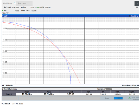
Band38-10MHz-64QAM-38200-50RB#0
