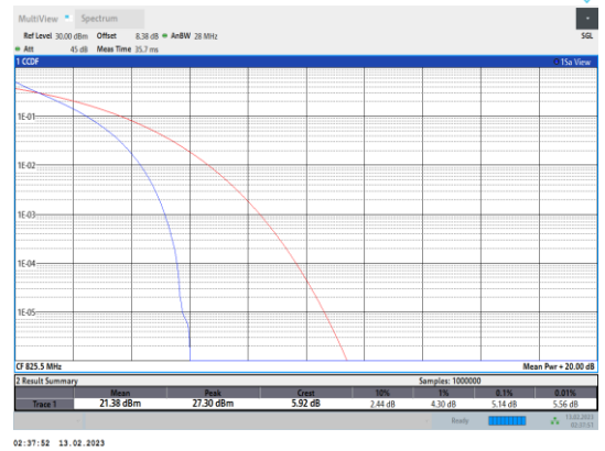
Band5-3MHz-QPSK-20415-15RB#0
