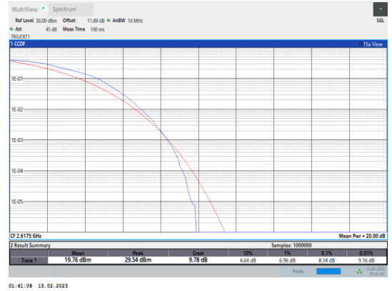
Band38-5MHz-64QAM-38225-25RB#0
