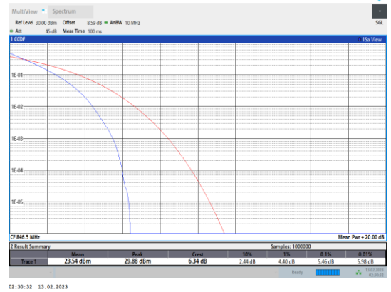
Band5-5MHz-QPSK-20625-25RB#0
