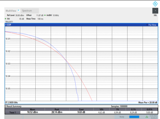
Band41-15MHz-16QAM-39725-75RB#0
