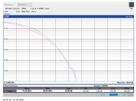
Band41-5MHz-16QAM-39675-25RB#0
