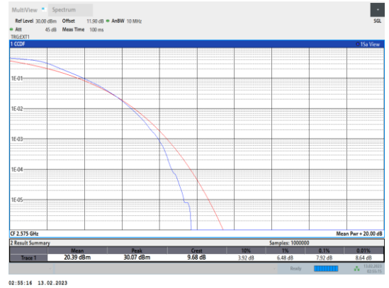
Band38-10MHz-QPSK-37800-50RB#0
