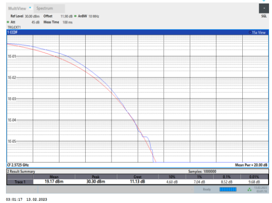
Band38-5MHz-16QAM-37775-25RB#0
