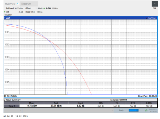
Band38-15MHz-QPSK-38175-75RB#0
