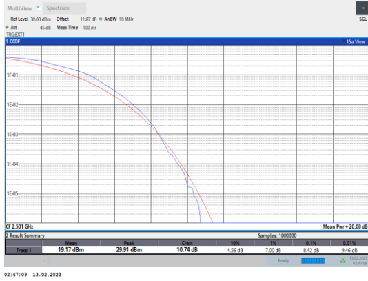
Band41-10MHz-16QAM-39700-50RB#0
