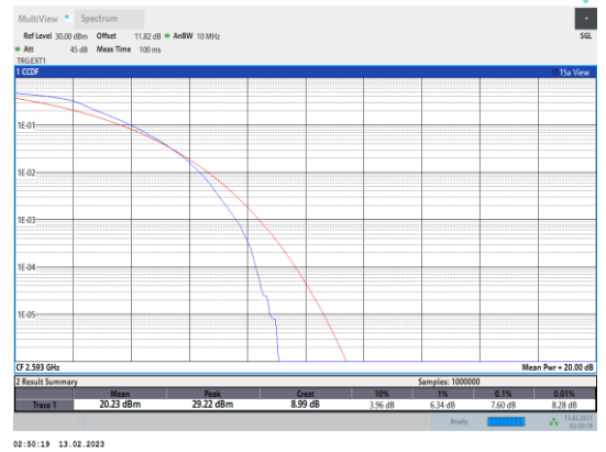
Band41-5MHz-QPSK-40620-25RB#0
