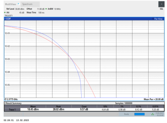
Band38-15MHz-16QAM-37825-75RB#0
