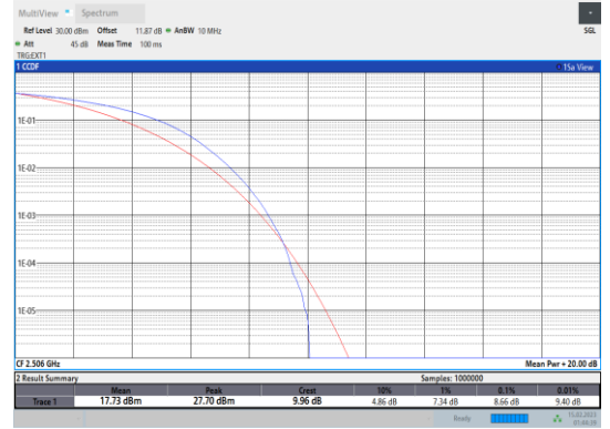
Band41-20MHz-64QAM-39750-100RB#0
