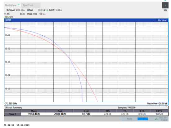
Band38-15MHz-64QAM-38000-75RB#0
