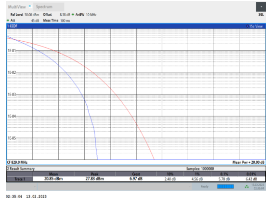
Band5-10MHz-QPSK-20450-50RB#0
