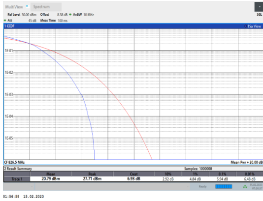
Band5-5MHz-64QAM-20425-25RB#0
