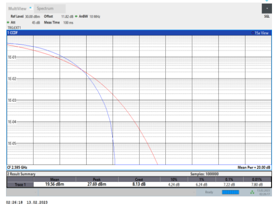
Band38-15MHz-QPSK-38000-75RB#0
