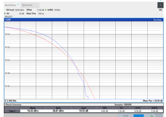
Band41-20MHz-16QAM-40620-100RB#0
