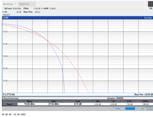
Band38-15MHz-QPSK-37825-75RB#0
