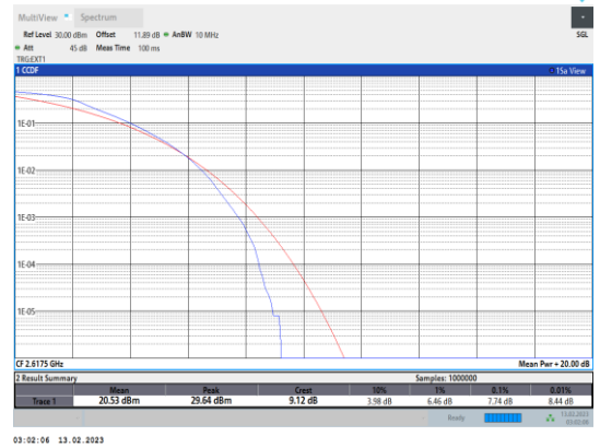
Band38-5MHz-QPSK-38225-25RB#0
