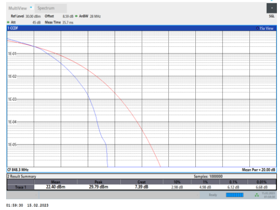
Band5-1.4MHz-64QAM-20643-6RB#0
