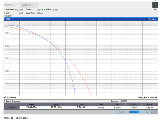
Band38-5MHz-QPSK-38000-25RB#0
