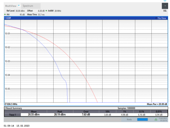
Band5-1.4MHz-64QAM-20525-6RB#0
