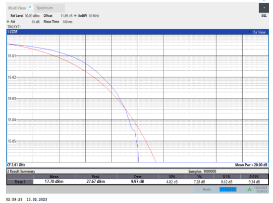
Band38-20MHz-16QAM-38150-100RB#0
