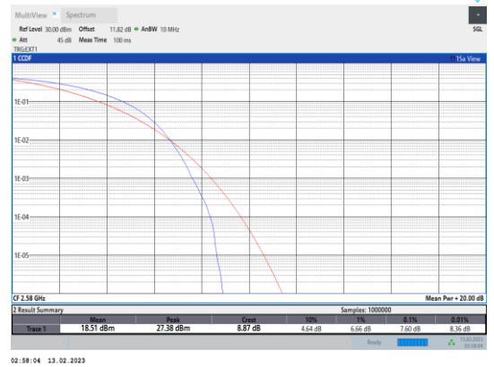
Band38-20MHz-QPSK-37850-100RB#0
