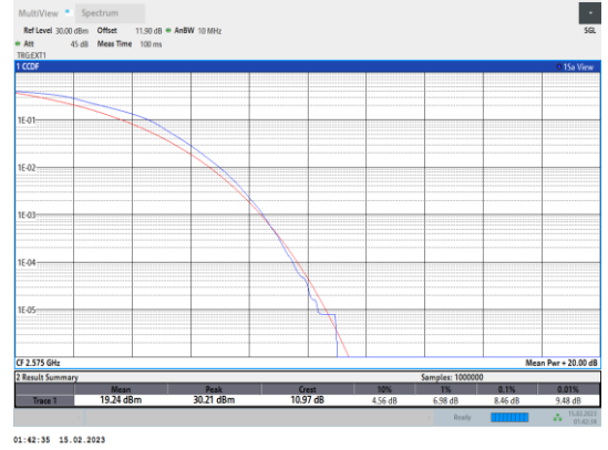
Band38-10MHz-64QAM-37800-50RB#0
