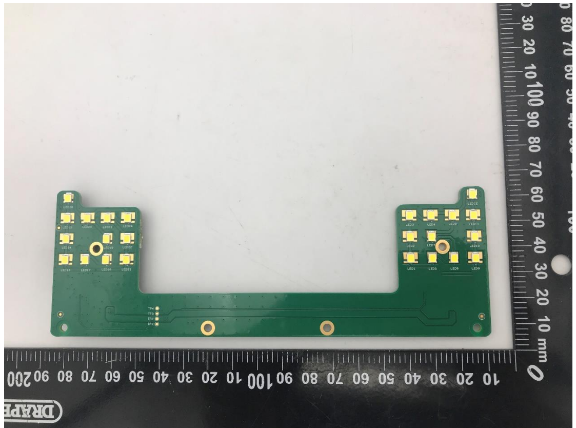
Photo 32 Inside of EUT
