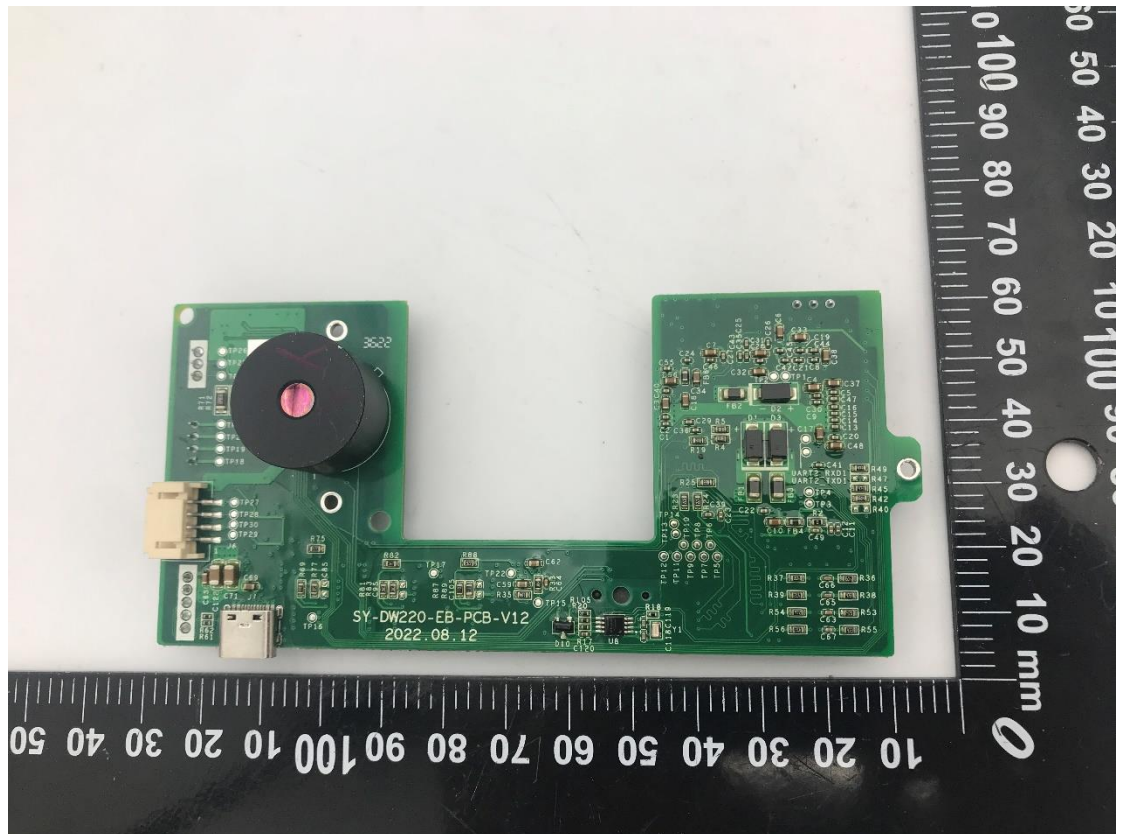
Photo 26 Inside of EUT
