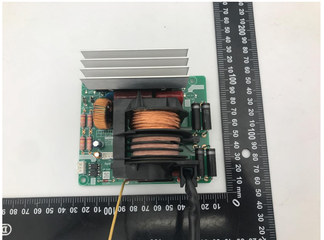
Photo 10 Inside of EUT
