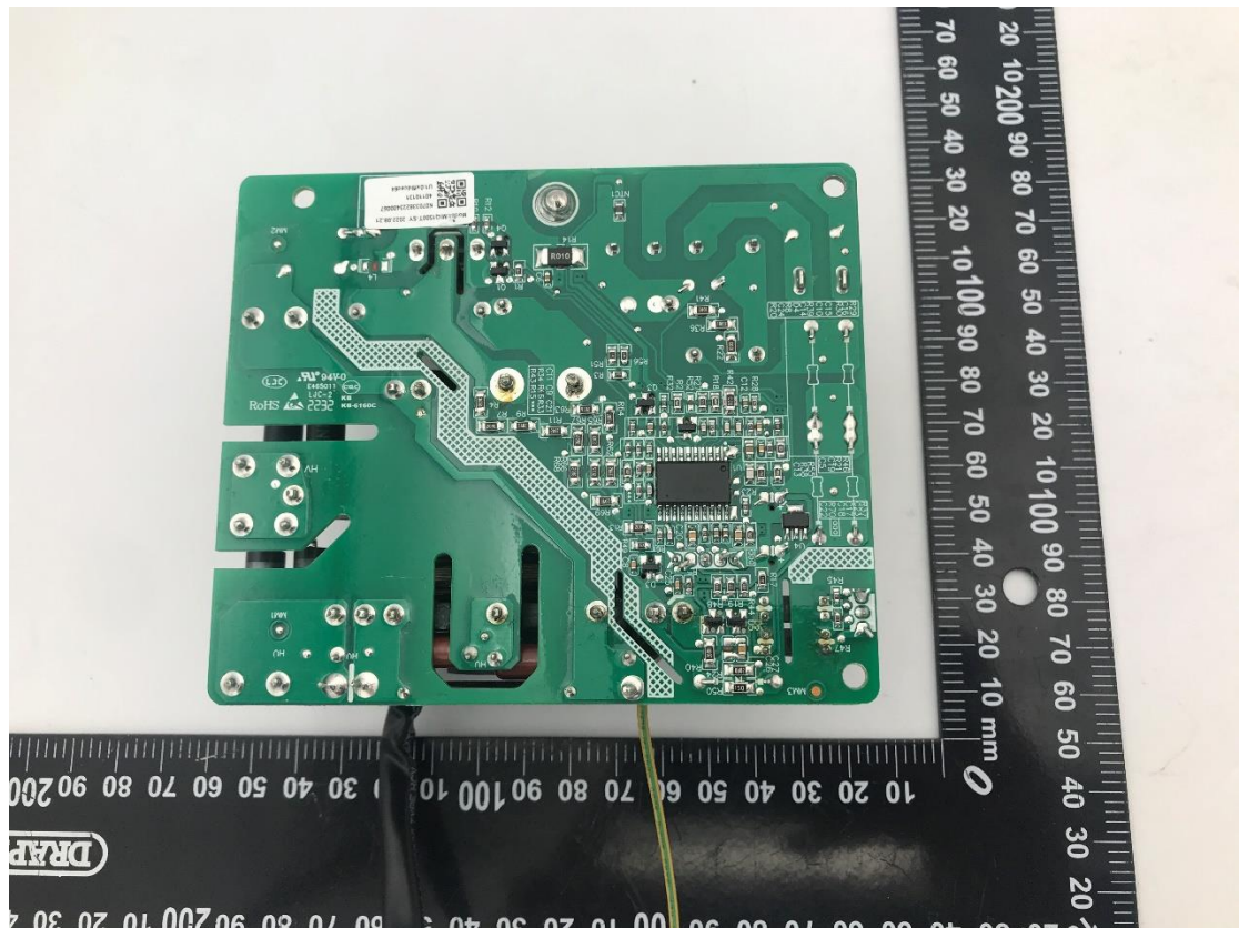
Photo 11 Inside of EUT
