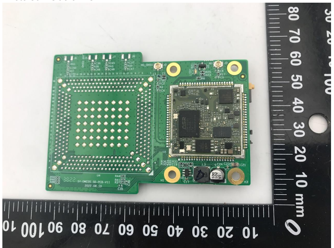
Photo 30 Inside of EUT
