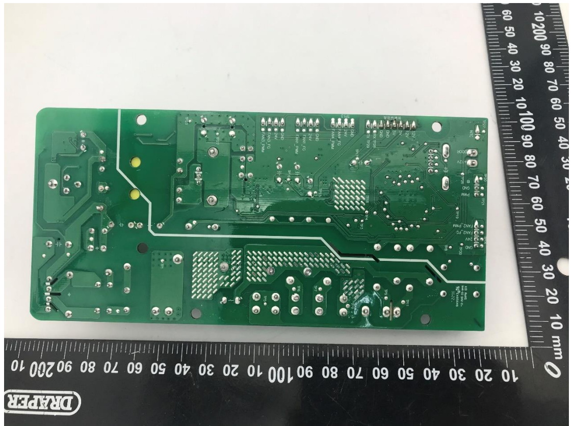
Photo 19 Inside of EUT
