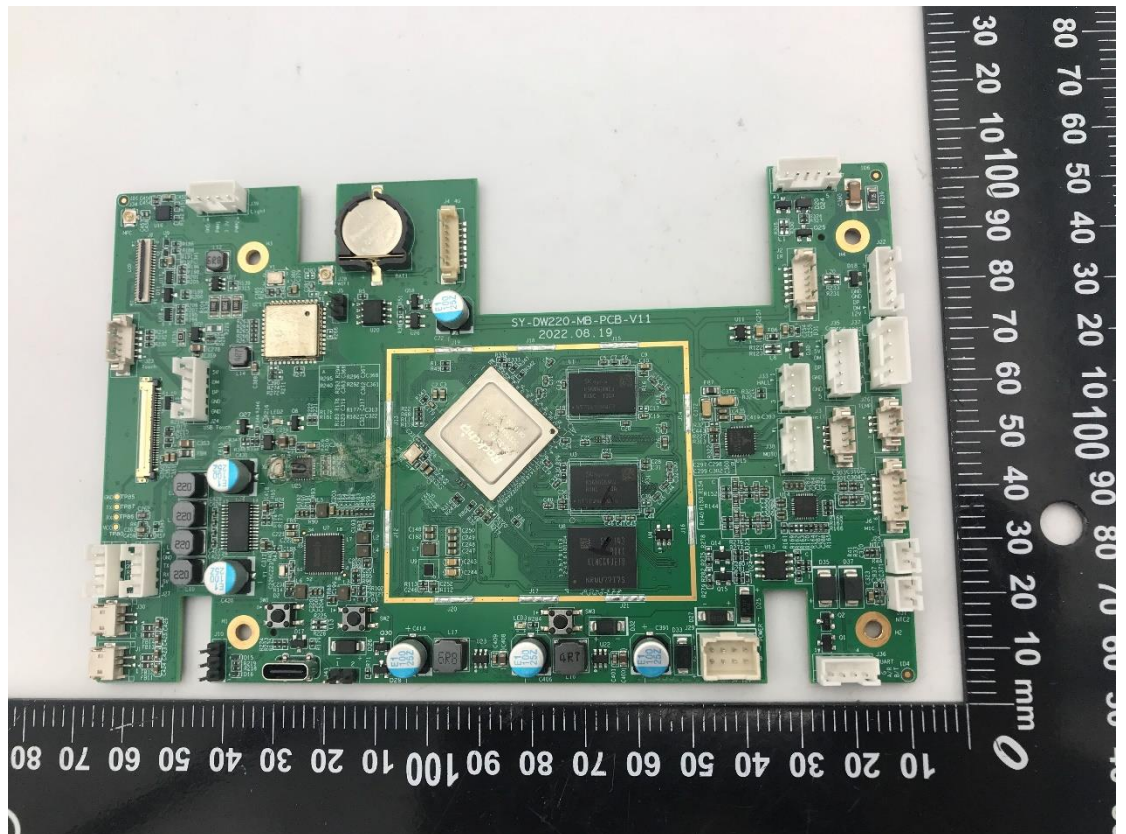
Photo 20 Inside of EUT
