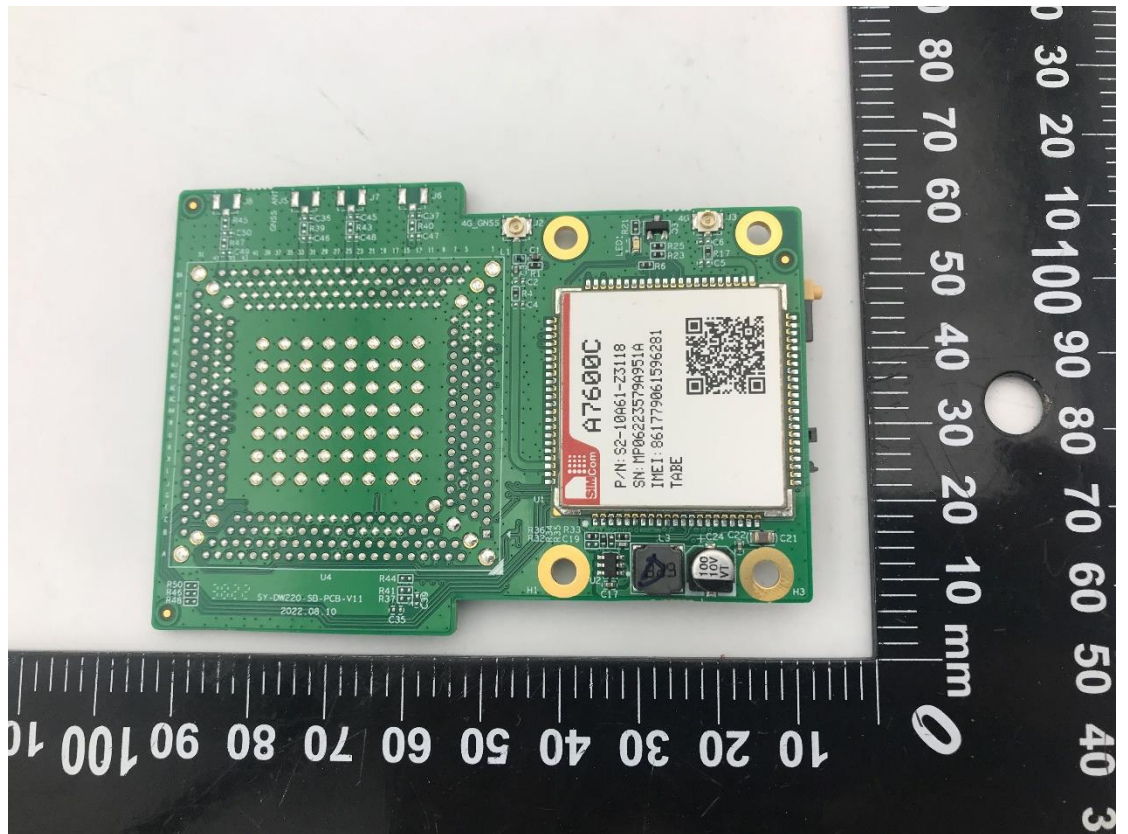
Photo 28 Inside of EUT
