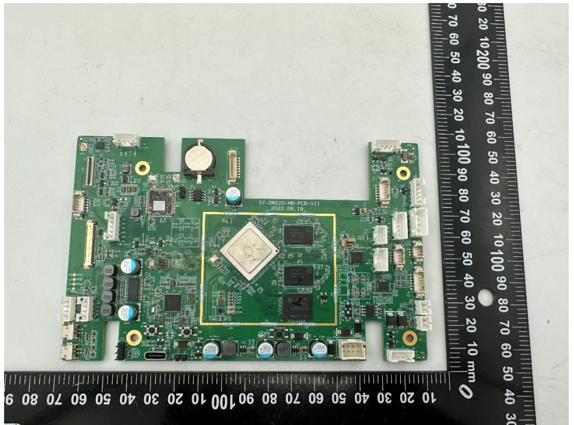
Photo 22 Inside of EUT
