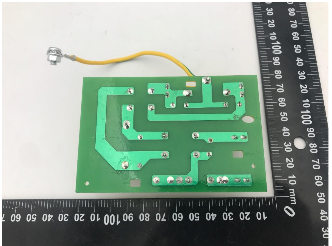
Photo 13 Inside of EUT
