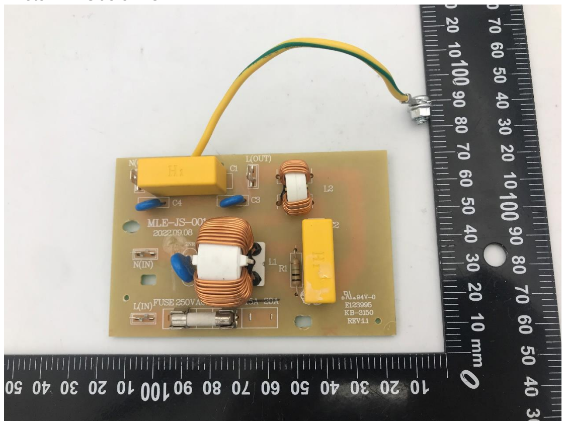
Photo 12 Inside of EUT
