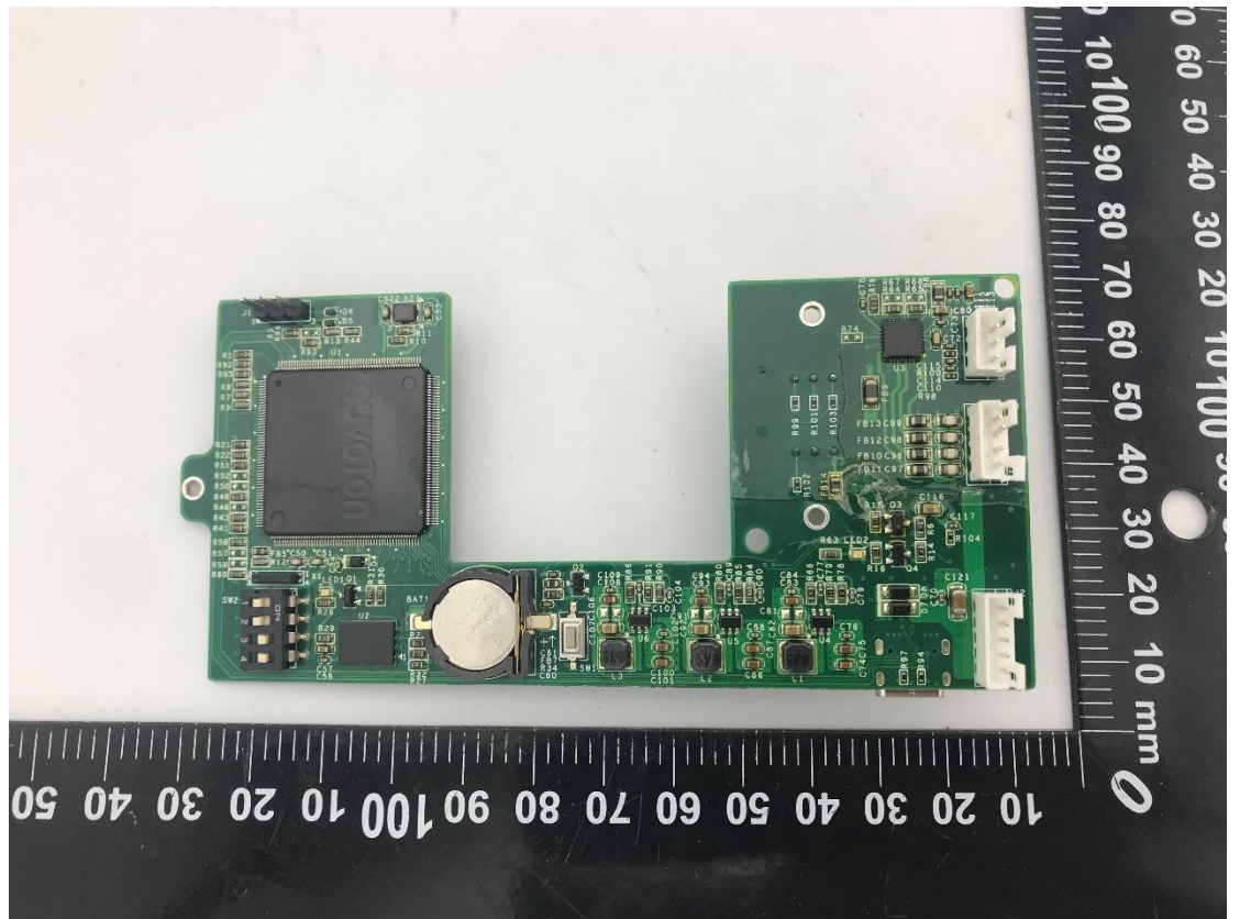
Photo 27 Inside of EUT
