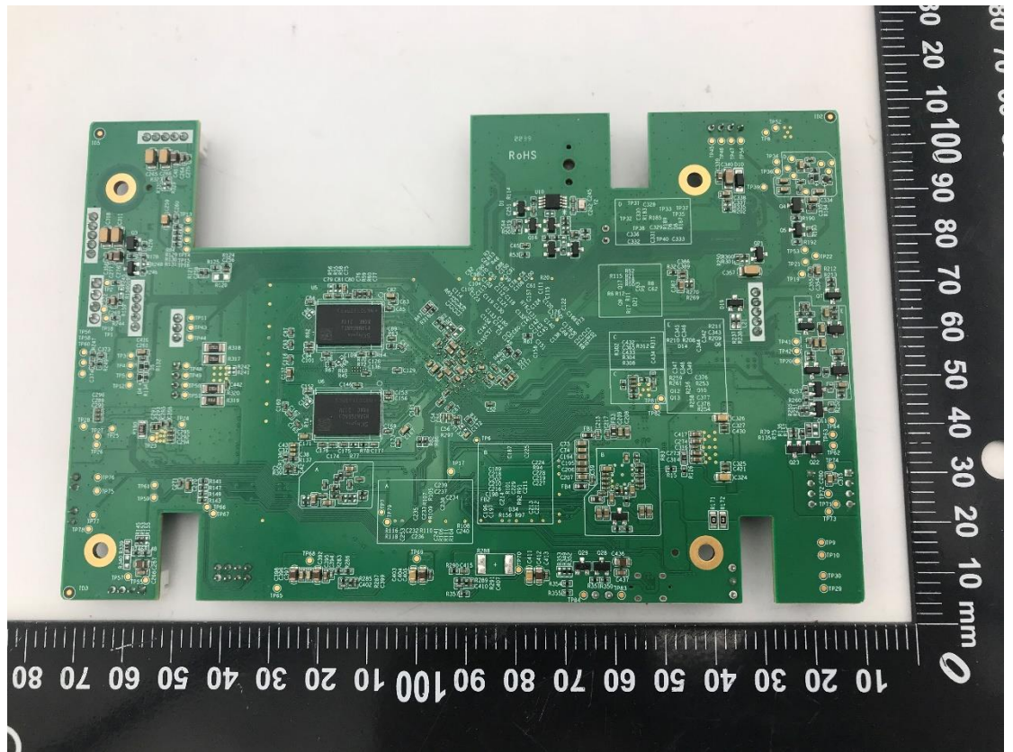
Photo 21 Inside of EUT
