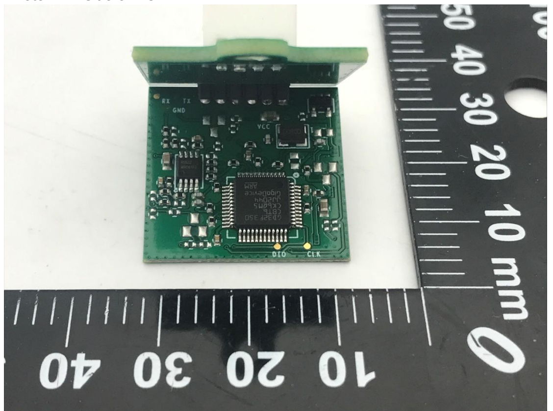
Photo 14 Inside of EUT
