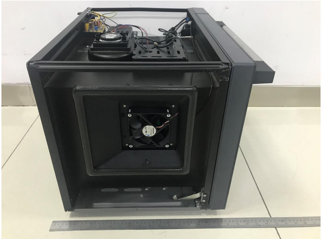
Photo 3 Inside of EUT
