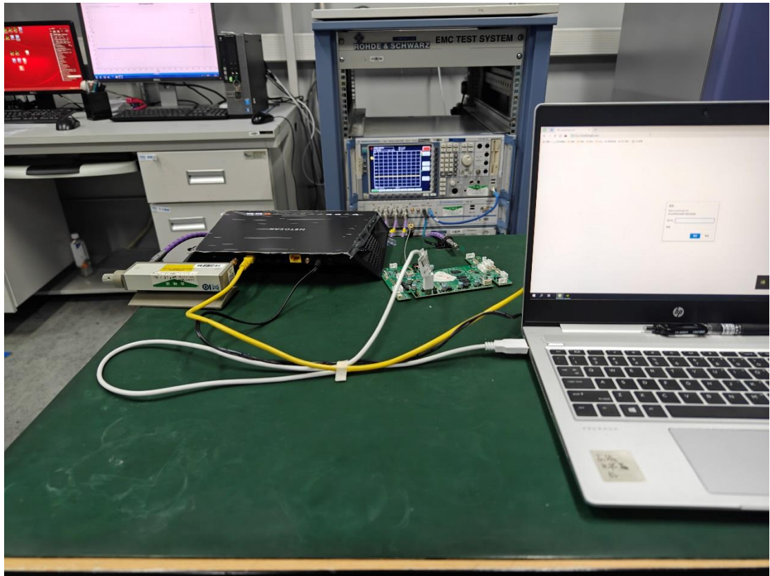
DFS Test Setup
