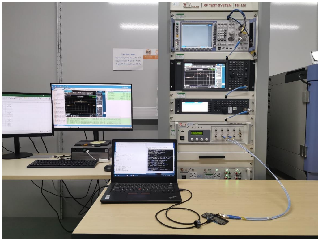
Photograph 3: Set-up photo for RF Conducted
