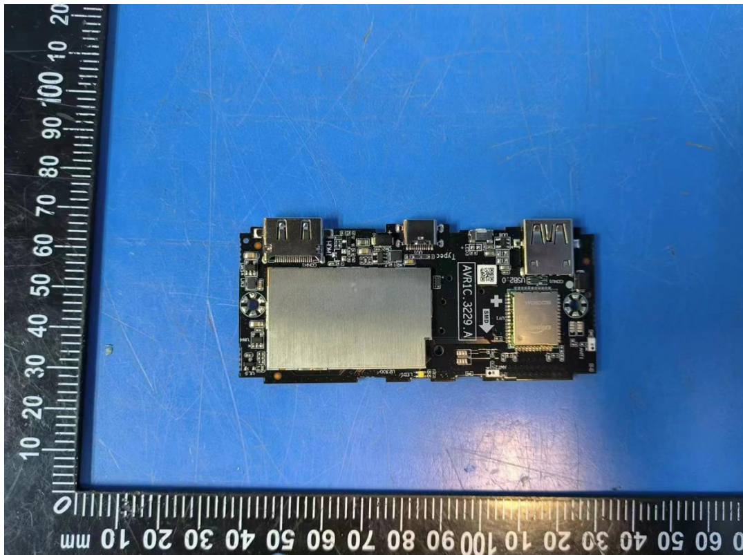
Figure 2 PCB overall view
