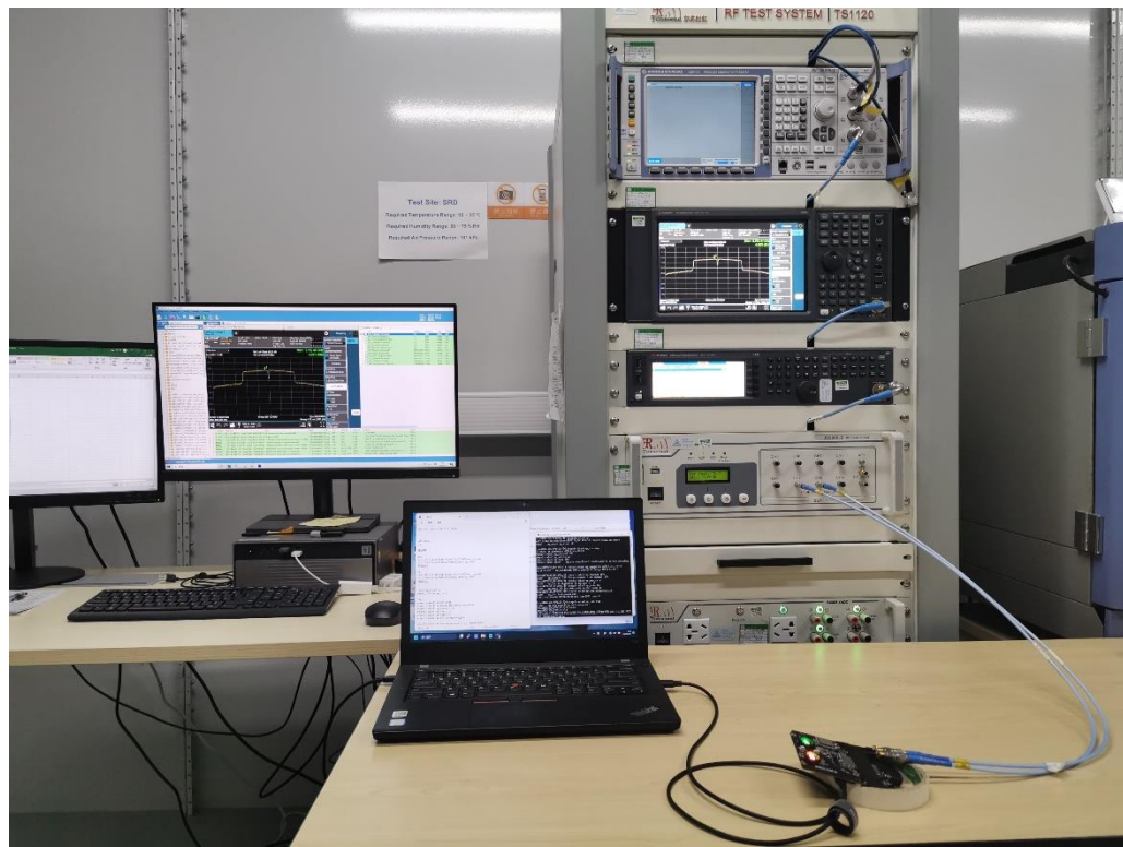
Photograph 3: Set-up photo for RF Conducted Test
