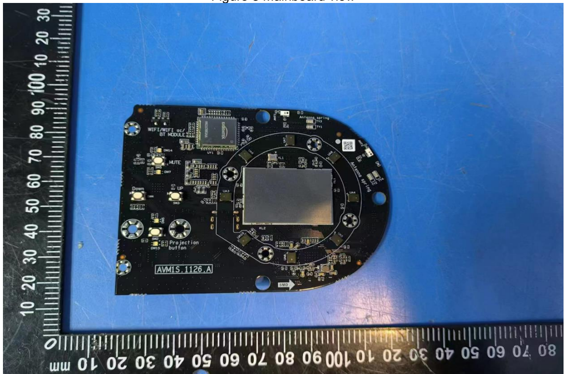
Figure 4 Mainboard view
