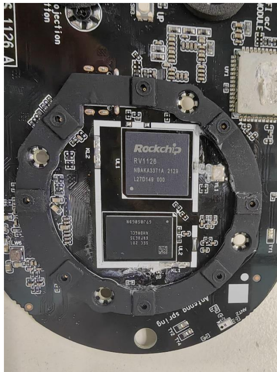
Figure 5 Shield-off view
