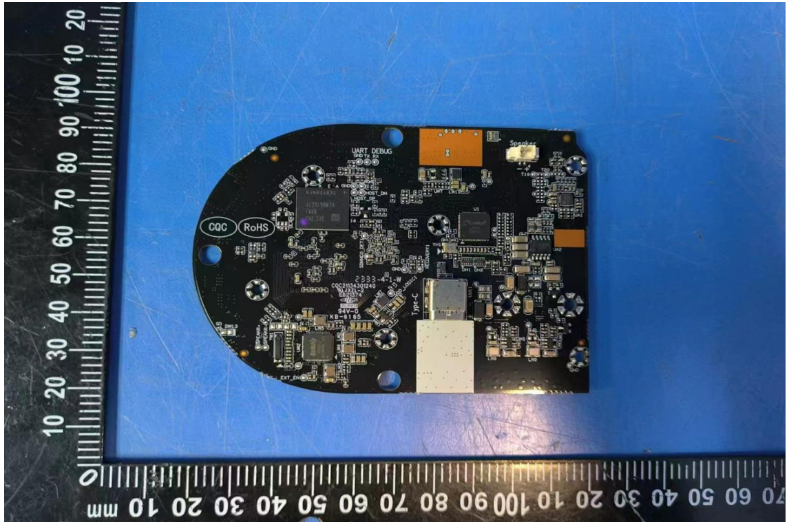
Figure 3 Mainboard view
