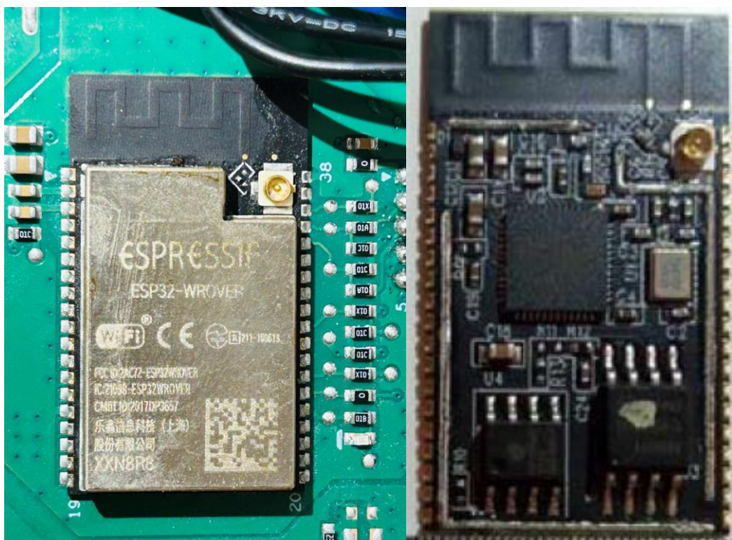
Figure 28 Wireless module
