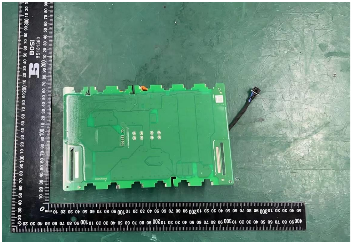
Figure 29 Bottom view of BMS board
