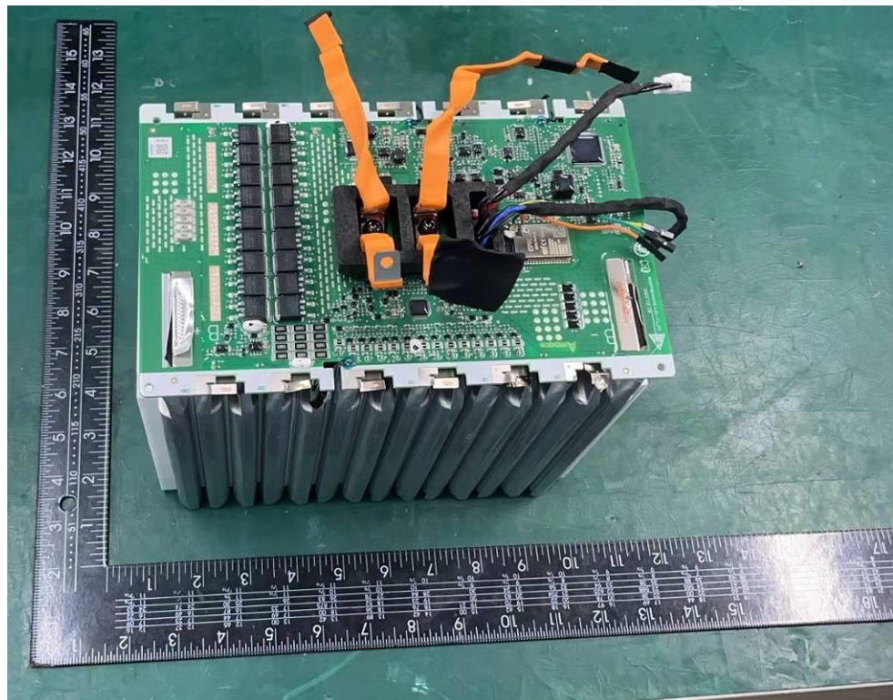
Figure 26 Internal view of battery module
