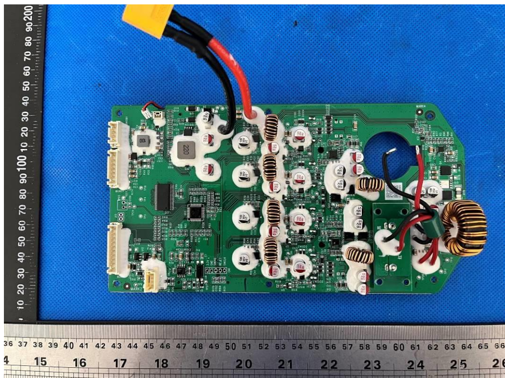
Figure 8 Top view of DC output board
