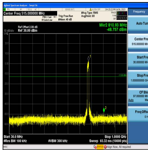
Band71-15MHz-16QAM-133297-75RB#0-Range1:30~1000MHz
