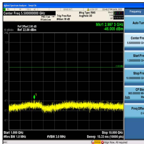
Band71-5MHz-16QAM-133447-25RB#0-Range2:1000~10000MHz
