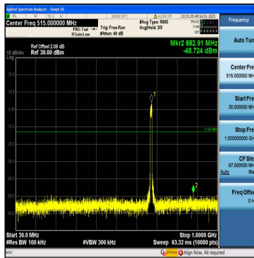
Band71-10MHz-16QAM-133297-50RB#0-Range1:30~1000MHz
