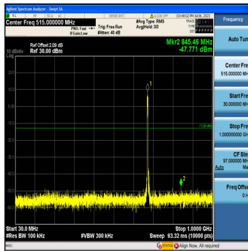
Band71-5MHz-16QAM-133297-25RB#0-Range1:30~1000MHz
