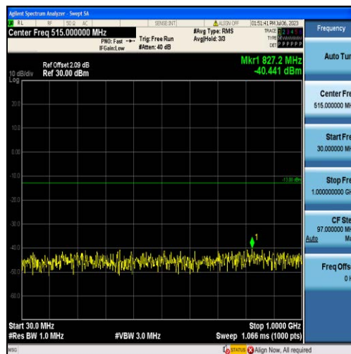
Band66-1.4MHz-16QAM-131979-6RB#0-Range1:30~1000MHz
