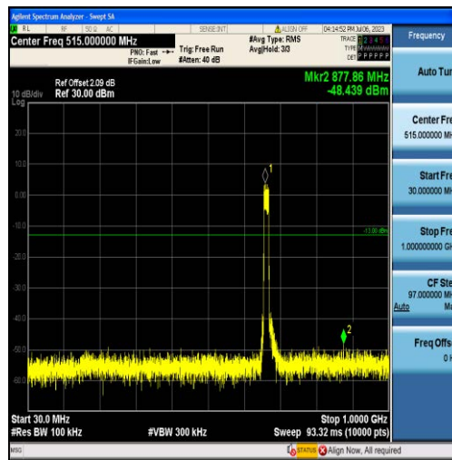
Band71-15MHz-QPSK-133197-75RB#0-Range1:30~1000MHz
