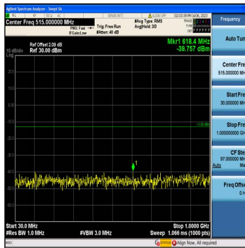
Band66-3MHz-QPSK-131987-15RB#0-Range1:30~1000MHz
