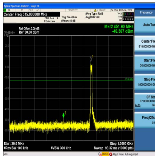
Band71-15MHz-16QAM-133197-75RB#0-Range1:30~1000MHz
