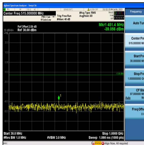
Band66-1.4MHz-QPSK-132665-6RB#0-Range1:30~1000MHz
