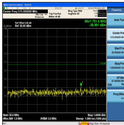
Band66-3MHz-16QAM-131987-15RB#0-Range1:30~1000MHz
