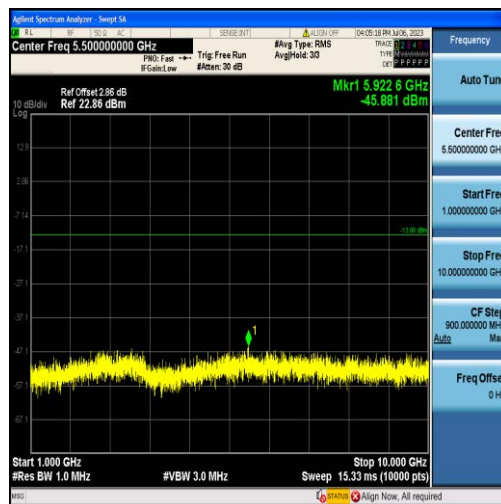
Band71-10MHz-16QAM-133422-50RB#0-Range2:1000~10000MHz
