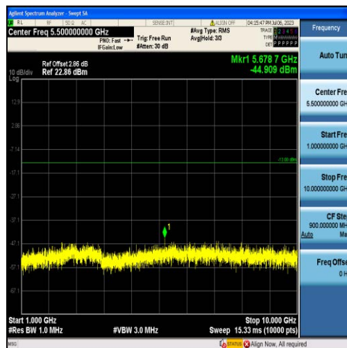
Band71-15MHz-16QAM-133397-75RB#0-Range2:1000~10000MHz
