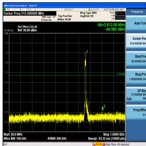
Band71-10MHz-16QAM-133172-50RB#0-Range1:30~1000MHz
