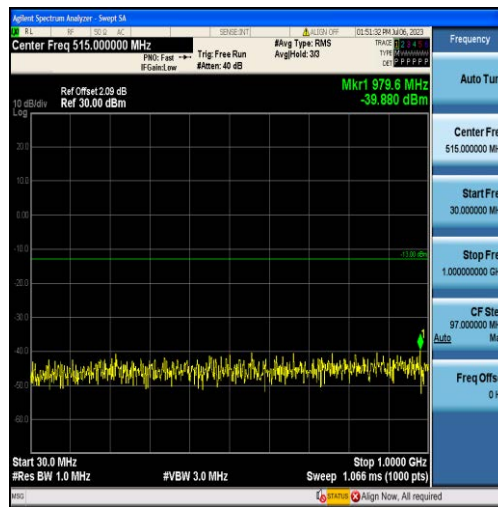
Band66-1.4MHz-QPSK-131979-6RB#0-Range1:30~1000MHz
