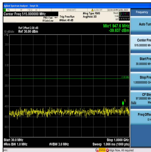
Band66-3MHz-QPSK-132657-15RB#0-Range1:30~1000MHz
