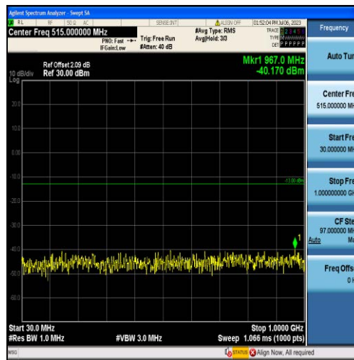
Band66-1.4MHz-16QAM-132322-6RB#0-Range1:30~1000MHz
