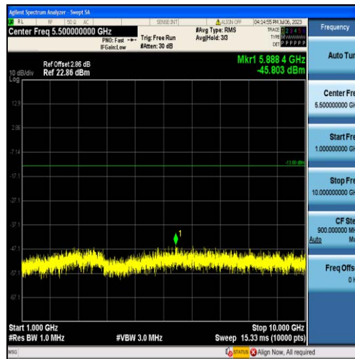
Band71-15MHz-QPSK-133197-75RB#0-Range2:1000~10000MHz
