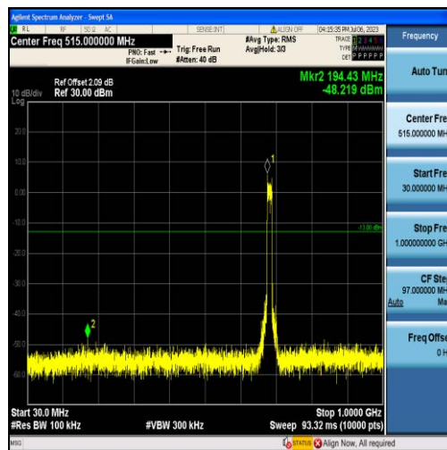
Band71-15MHz-QPSK-133397-75RB#0-Range1:30~1000MHz
