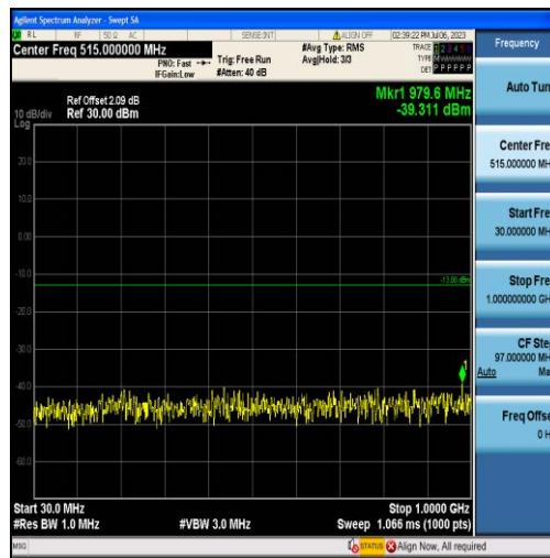
Band66-20MHz-16QAM-132322-100RB#0-Range1:30~1000MHz
