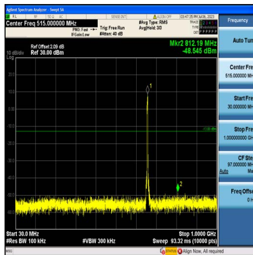
Band71-5MHz-16QAM-133147-25RB#0-Range1:30~1000MHz
