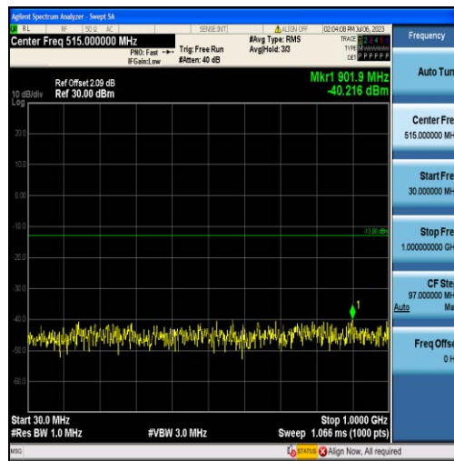
Band66-3MHz-16QAM-132322-15RB#0-Range1:30~1000MHz
