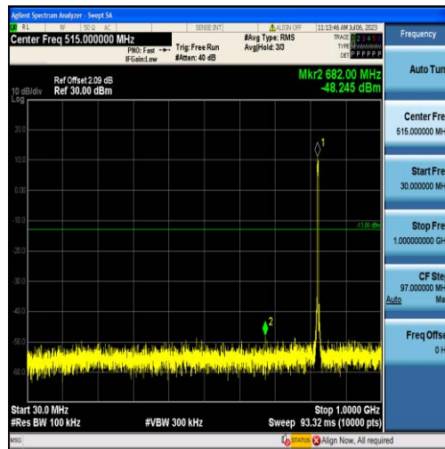
Band26-3MHz-QPSK-26805-15RB#0-Range1:30~1000MHz
