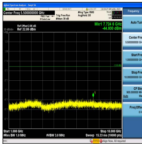
Band26-3MHz-16QAM-26775-15RB#0-Range2:1000~10000MHz
