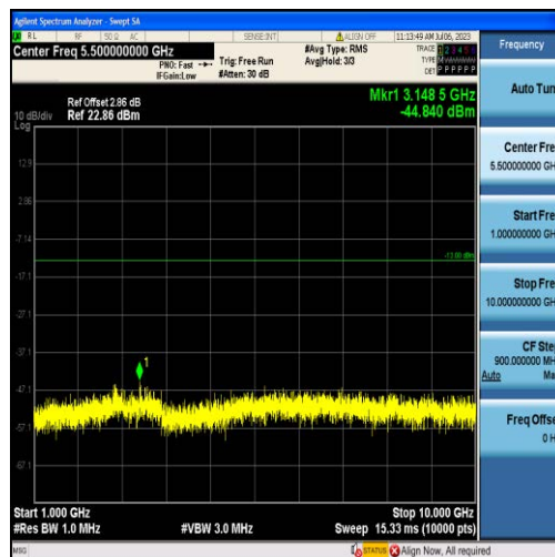
Band26-3MHz-QPSK-26805-15RB#0-Range2:1000~10000MHz
