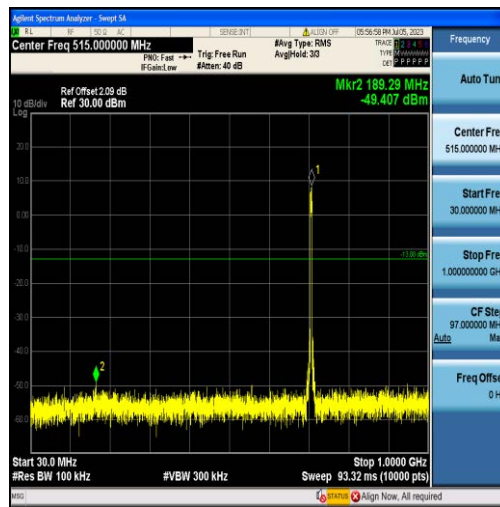
Band17-5MHz-QPSK-23825-25RB#0-Range1:30~1000MHz
