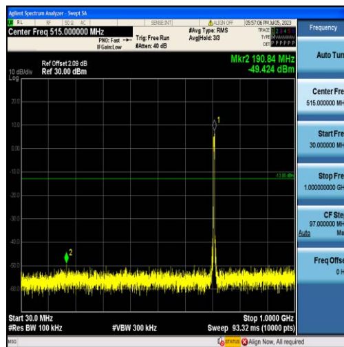
Band17-5MHz-16QAM-23825-25RB#0-Range1:30~1000MHz
