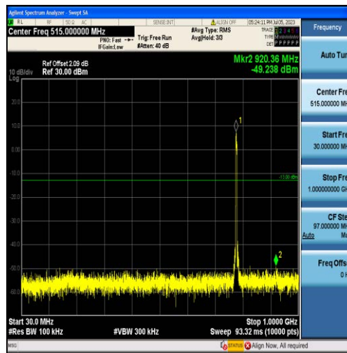
Band13-5MHz-16QAM-23230-25RB#0-Range1:30~1000MHz
