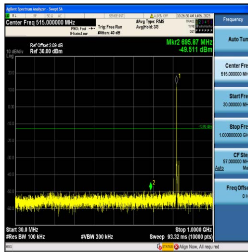
Band26-1.4MHz-QPSK-26783-6RB#0-Range1:30~1000MHz
