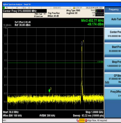
Band13-5MHz-QPSK-23205-25RB#0-Range1:30~1000MHz
