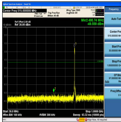
Band17-5MHz-QPSK-23755-25RB#0-Range1:30~1000MHz
