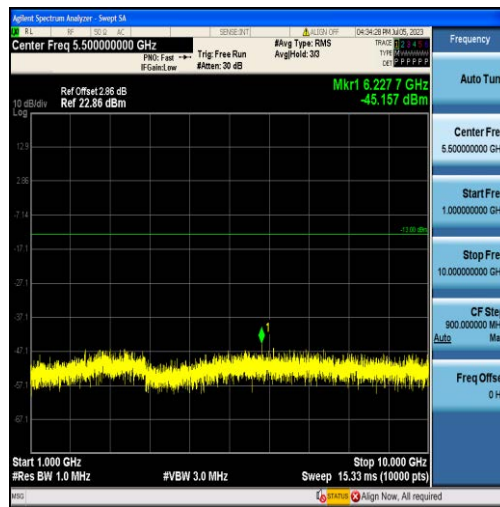
Band12-1.4MHz-QPSK-23173-6RB#0-Range2:1000~10000MHz
