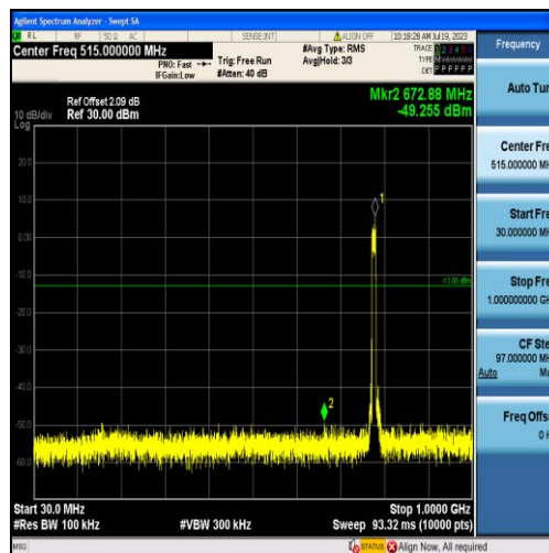
Band13-10MHz-16QAM-23230-50RB#0-Range1:30~1000MHz
