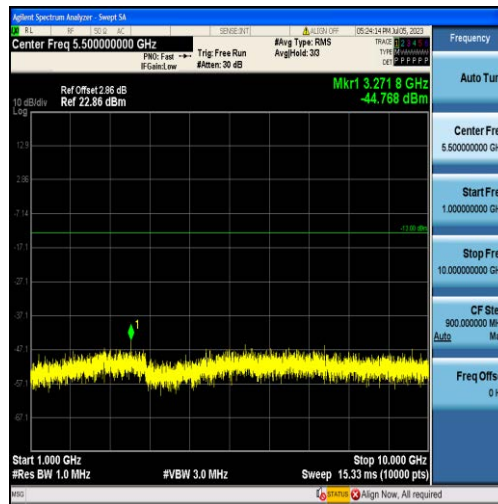
Band13-5MHz-16QAM-23230-25RB#0-Range2:1000~10000MHz
