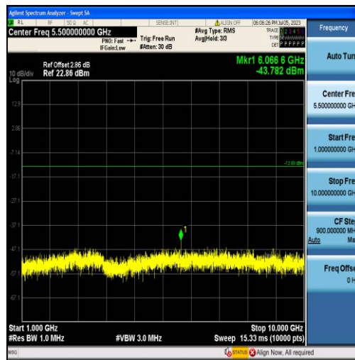
Band17-10MHz-QPSK-23790-50RB#0-Range2:1000~10000MHz
