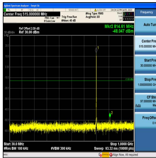
Band12-1.4MHz-16QAM-23095-6RB#0-Range1:30~1000MHz
