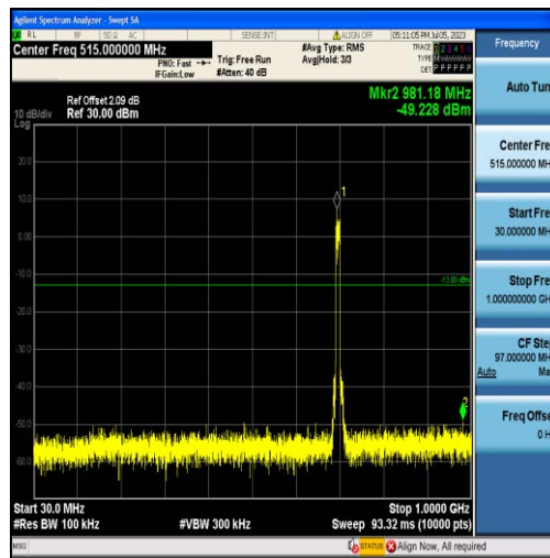
Band12-10MHz-QPSK-23060-50RB#0-Range1:30~1000MHz
