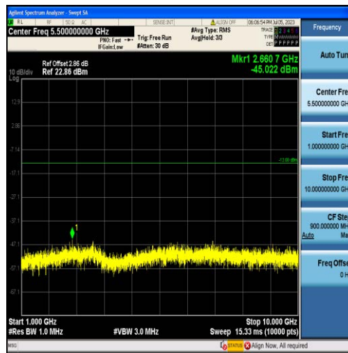
Band17-10MHz-16QAM-23800-50RB#0-Range2:1000~10000MHz
