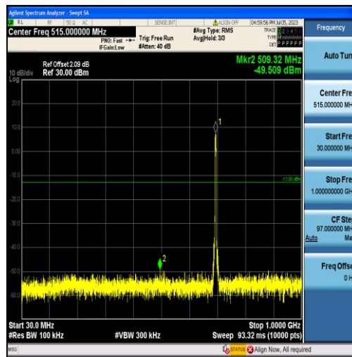
Band12-5MHz-QPSK-23035-25RB#0-Range1:30~1000MHz
