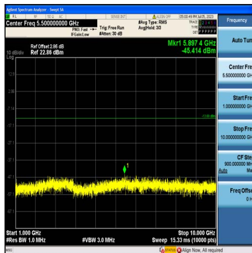
Band12-5MHz-16QAM-23155-25RB#0-Range2:1000~10000MHz
