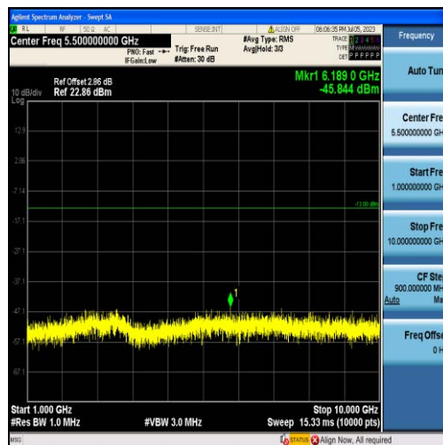
Band17-10MHz-16QAM-23790-50RB#0-Range2:1000~10000MHz
