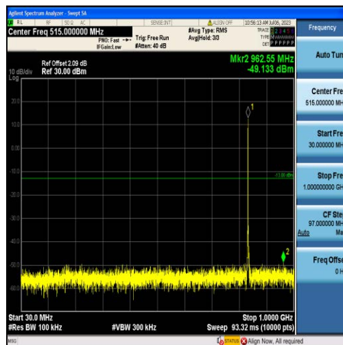
Band26-1.4MHz-QPSK-26915-6RB#0-Range1:30~1000MHz
