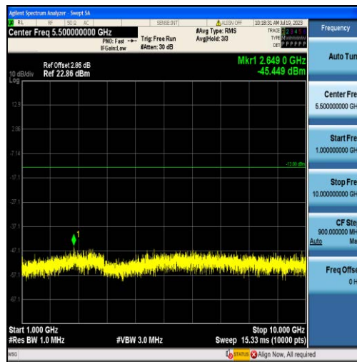
Band13-10MHz-16QAM-23230-50RB#0-Range2:1000~10000MHz
