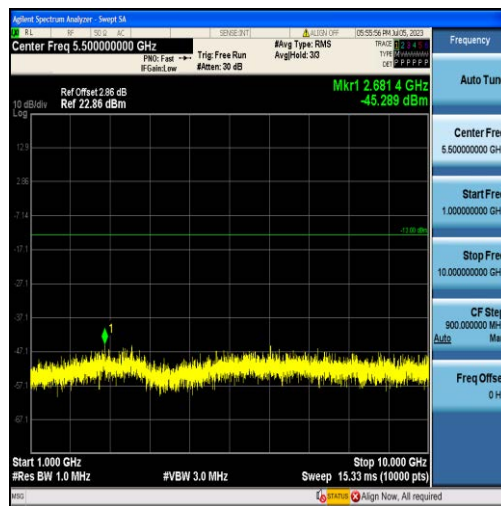
Band17-5MHz-16QAM-23755-25RB#0-Range2:1000~10000MHz
