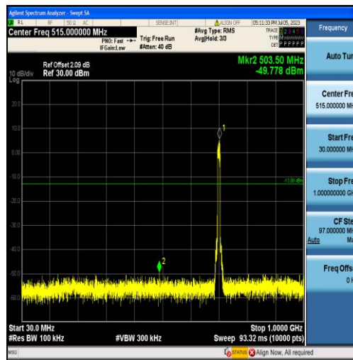
Band12-10MHz-16QAM-23095-50RB#0-Range1:30~1000MHz
