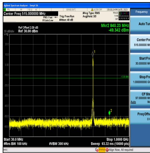
Band12-5MHz-16QAM-23095-25RB#0-Range1:30~1000MHz
