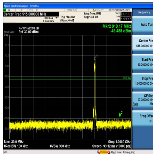
Band17-10MHz-QPSK-23790-50RB#0-Range1:30~1000MHz
