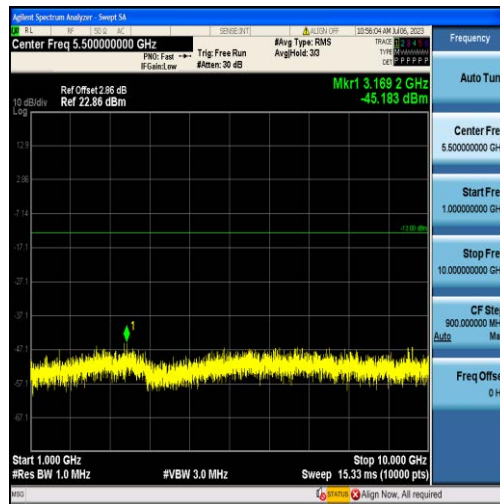
Band26-1.4MHz-16QAM-26797-6RB#0-Range2:1000~10000MHz
