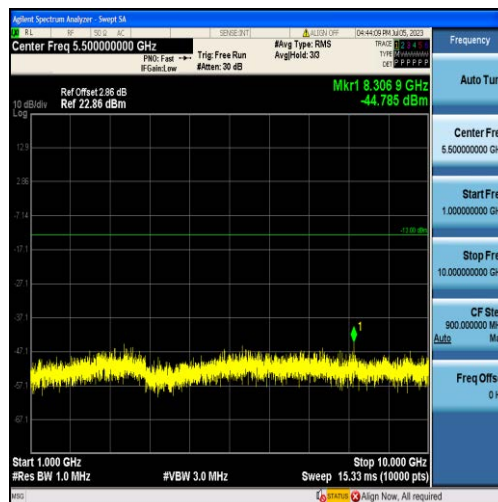
Band12-3MHz-16QAM-23165-15RB#0-Range2:1000~10000MHz
