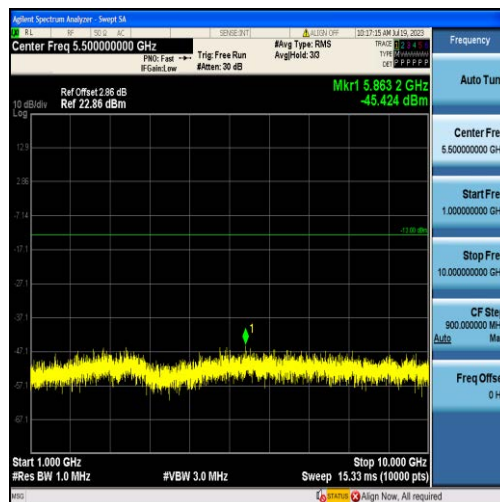
Band13-5MHz-16QAM-23255-25RB#0-Range2:1000~10000MHz
