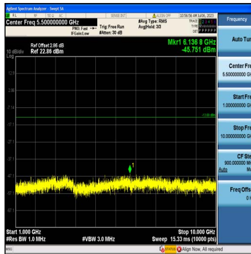
Band26-1.4MHz-QPSK-27033-6RB#0-Range2:1000~10000MHz
