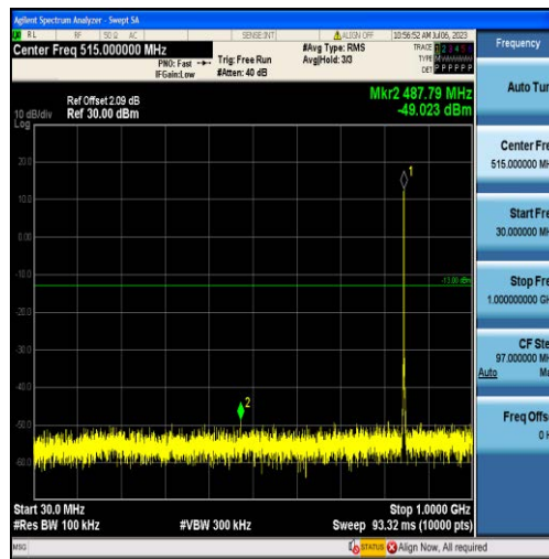
Band26-1.4MHz-QPSK-27033-6RB#0-Range1:30~1000MHz
