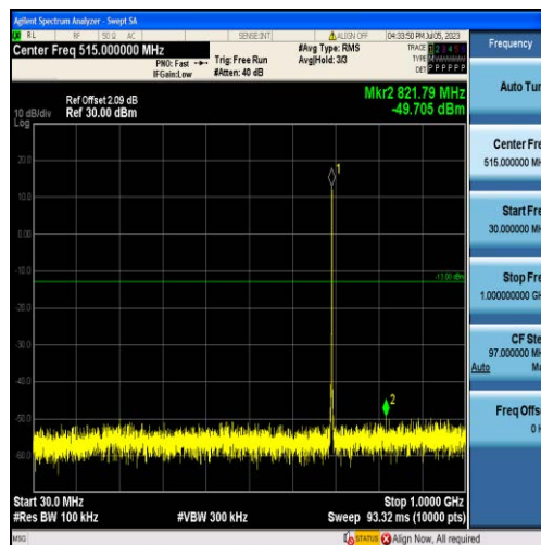
Band12-1.4MHz-16QAM-23017-6RB#0-Range1:30~1000MHz
