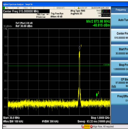
Band17-10MHz-QPSK-23780-50RB#0-Range1:30~1000MHz
