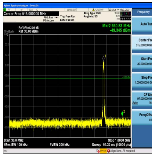
Band13-10MHz-QPSK-23230-50RB#0-Range1:30~1000MHz
