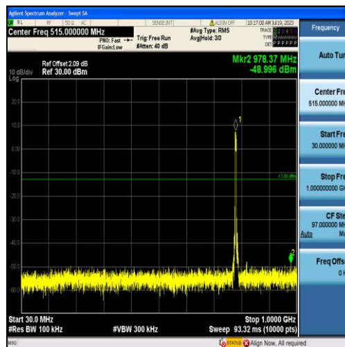
Band13-5MHz-QPSK-23255-25RB#0-Range1:30~1000MHz
