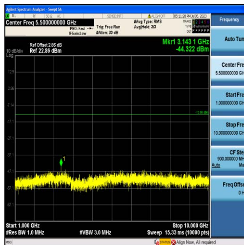
Band12-10MHz-QPSK-23095-50RB#0-Range2:1000~10000MHz
