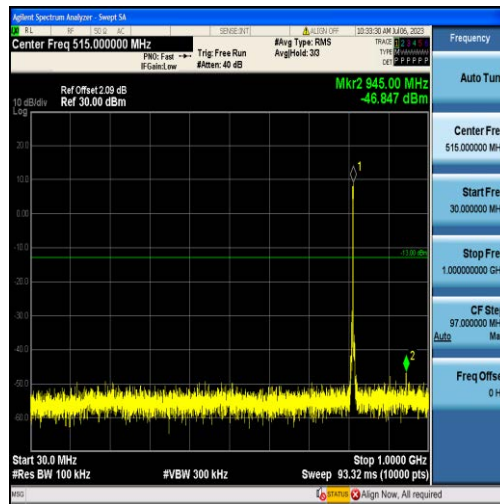
Band26-3MHz-QPSK-26705-15RB#0-Range1:30~1000MHz
