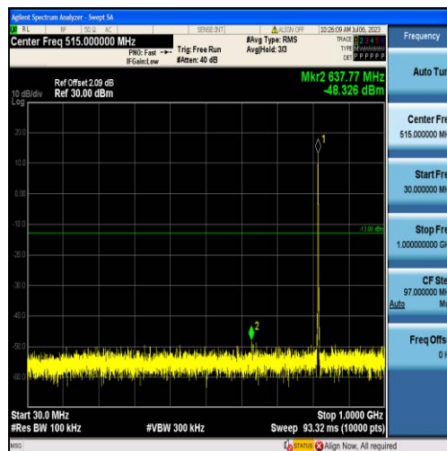
Band26-1.4MHz-QPSK-26740-6RB#0-Range1:30~1000MHz
