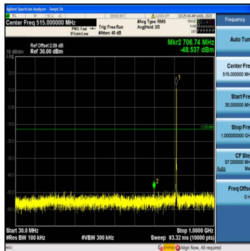
Band26-1.4MHz-QPSK-26697-6RB#0-Range1:30~1000MHz
