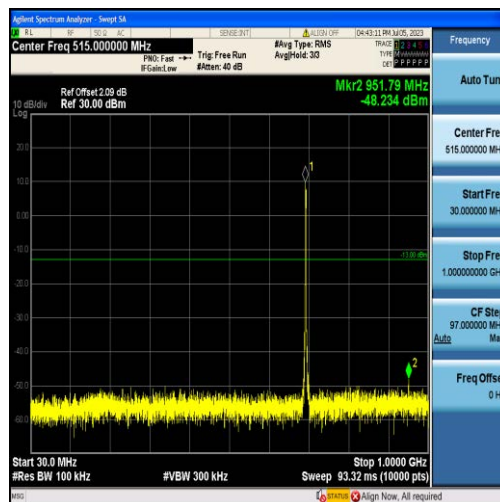
Band12-3MHz-16QAM-23025-15RB#0-Range1:30~1000MHz
