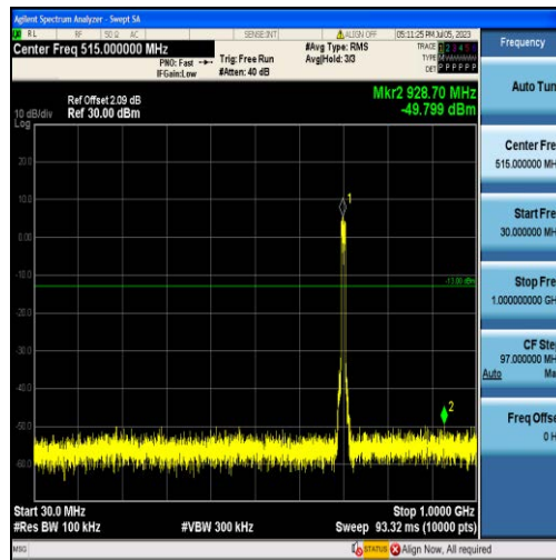
Band12-10MHz-QPSK-23095-50RB#0-Range1:30~1000MHz
