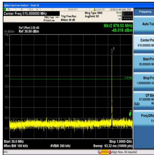
Band26-1.4MHz-16QAM-26915-6RB#0-Range1:30~1000MHz
