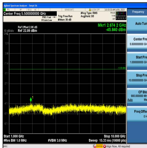
Band26-3MHz-QPSK-26705-15RB#0-Range2:1000~10000MHz
