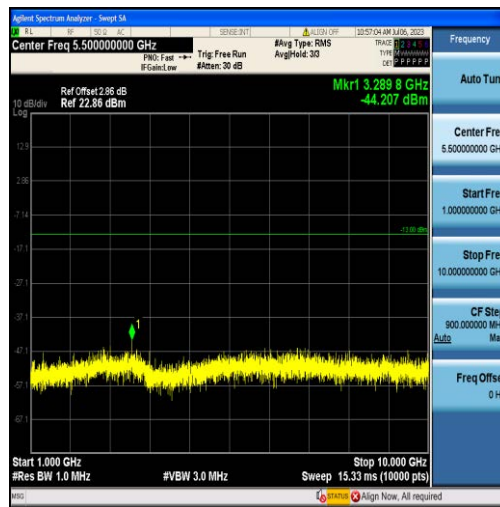
Band26-1.4MHz-16QAM-27033-6RB#0-Range2:1000~10000MHz
