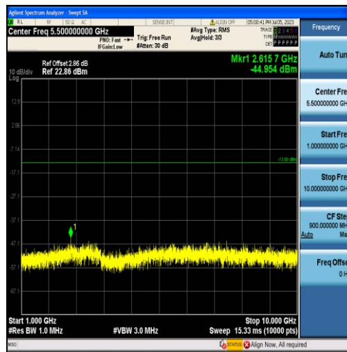
Band12-5MHz-QPSK-23155-25RB#0-Range2:1000~10000MHz
