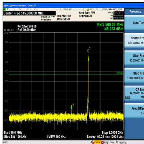
Band12-5MHz-16QAM-23035-25RB#0-Range1:30~1000MHz
