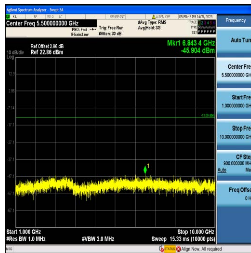
Band17-5MHz-QPSK-23755-25RB#0-Range2:1000~10000MHz
