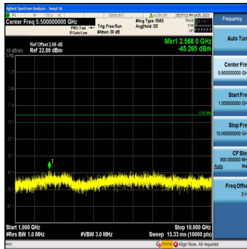
Band17-5MHz-QPSK-23825-25RB#0-Range2:1000~10000MHz
