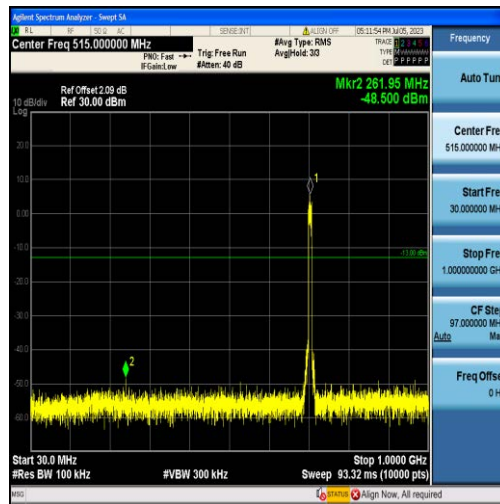
Band12-10MHz-16QAM-23130-50RB#0-Range1:30~1000MHz
