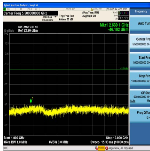
Band17-10MHz-16QAM-23780-50RB#0-Range2:1000~10000MHz
