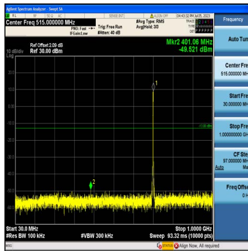
Band12-3MHz-16QAM-23095-15RB#0-Range1:30~1000MHz
