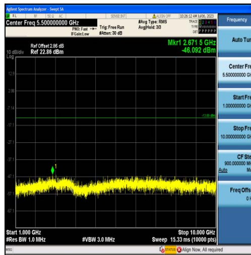
Band26-1.4MHz-QPSK-26740-6RB#0-Range2:1000~10000MHz
