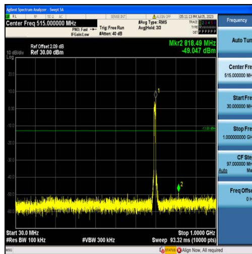
Band12-10MHz-16QAM-23060-50RB#0-Range1:30~1000MHz
