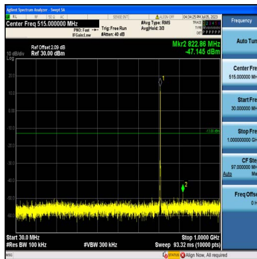
Band12-1.4MHz-QPSK-23173-6RB#0-Range1:30~1000MHz
