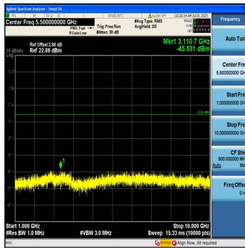
Band17-5MHz-QPSK-23790-25RB#0-Range2:1000~10000MHz
