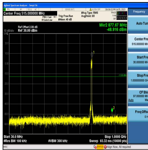
Band17-10MHz-16QAM-23780-50RB#0-Range1:30~1000MHz
