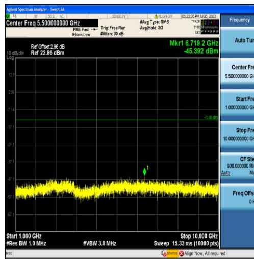
Band13-5MHz-16QAM-23205-25RB#0-Range2:1000~10000MHz
