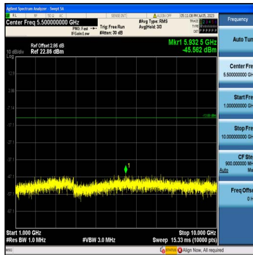
Band12-10MHz-QPSK-23060-50RB#0-Range2:1000~10000MHz
