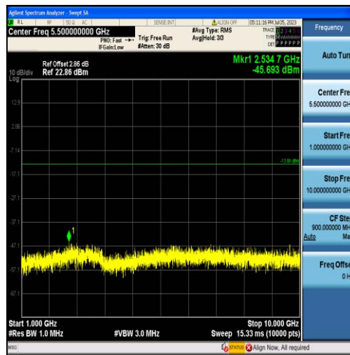
Band12-10MHz-16QAM-23060-50RB#0-Range2:1000~10000MHz
