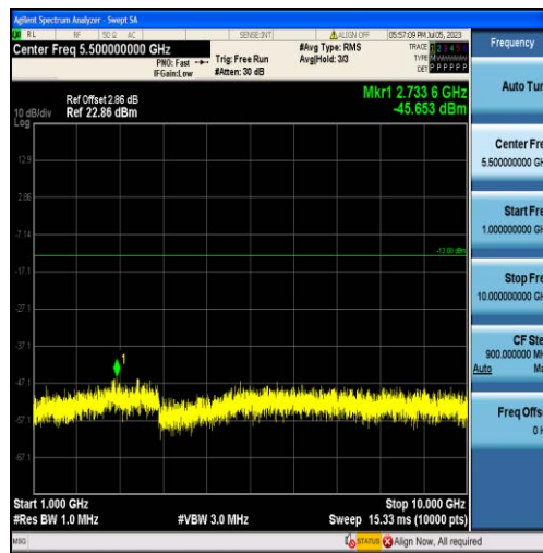
Band17-5MHz-16QAM-23825-25RB#0-Range2:1000~10000MHz
