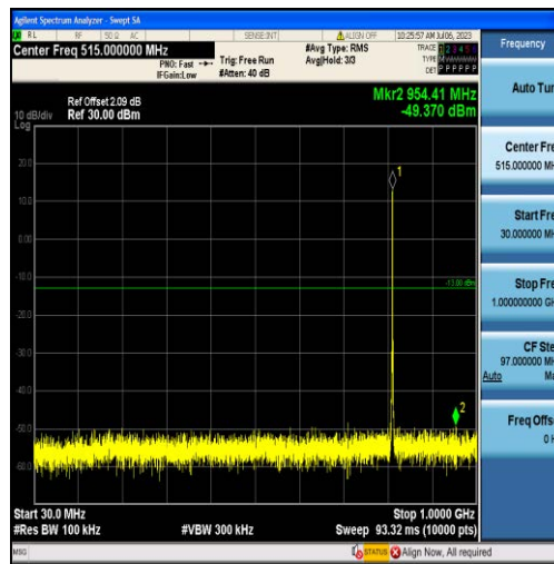
Band26-1.4MHz-16QAM-26697-6RB#0-Range1:30~1000MHz
