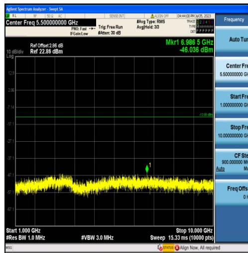
Band12-3MHz-QPSK-23165-15RB#0-Range2:1000~10000MHz
