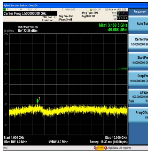
Band26-1.4MHz-QPSK-26915-6RB#0-Range2:1000~10000MHz
