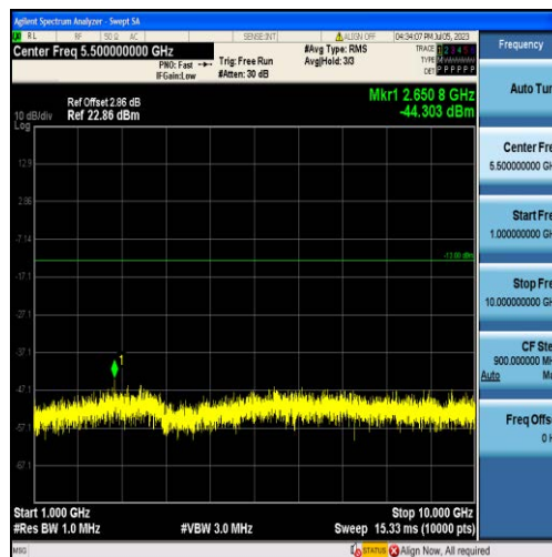
Band12-1.4MHz-QPSK-23095-6RB#0-Range2:1000~10000MHz
