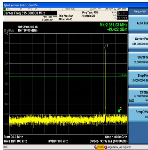
Band26-1.4MHz-16QAM-26740-6RB#0-Range1:30~1000MHz
