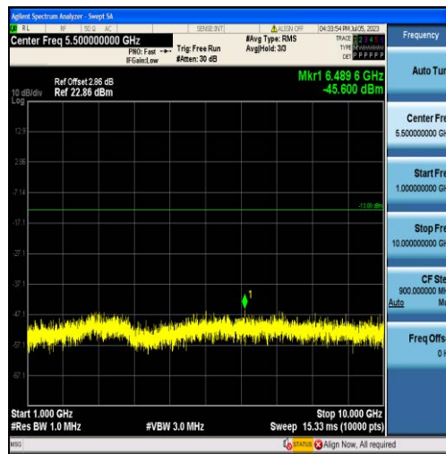
Band12-1.4MHz-16QAM-23017-6RB#0-Range2:1000~10000MHz
