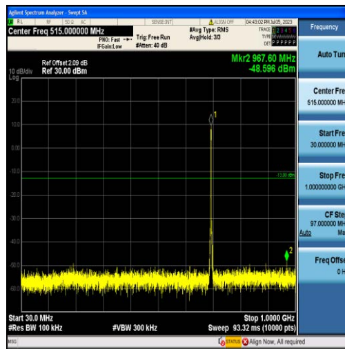
Band12-3MHz-QPSK-23025-15RB#0-Range1:30~1000MHz
