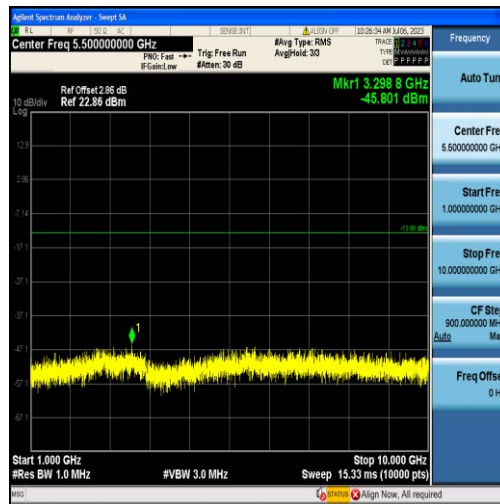
Band26-1.4MHz-QPSK-26783-6RB#0-Range2:1000~10000MHz
