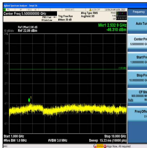
Band26-1.4MHz-16QAM-26915-6RB#0-Range2:1000~10000MHz
