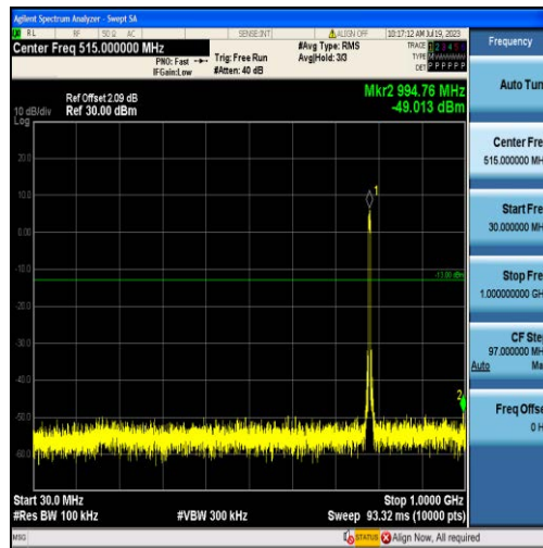
Band13-5MHz-16QAM-23255-25RB#0-Range1:30~1000MHz
