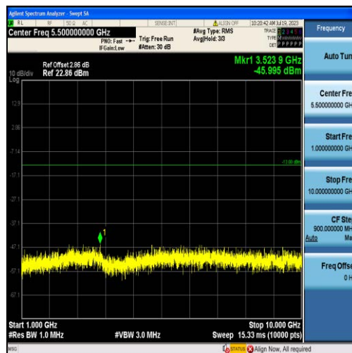
Band17-5MHz-16QAM-23790-25RB#0-Range2:1000~10000MHz
