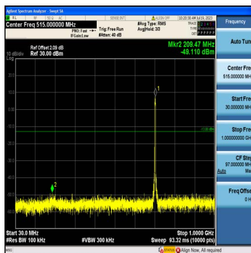
Band17-5MHz-QPSK-23790-25RB#0-Range1:30~1000MHz
