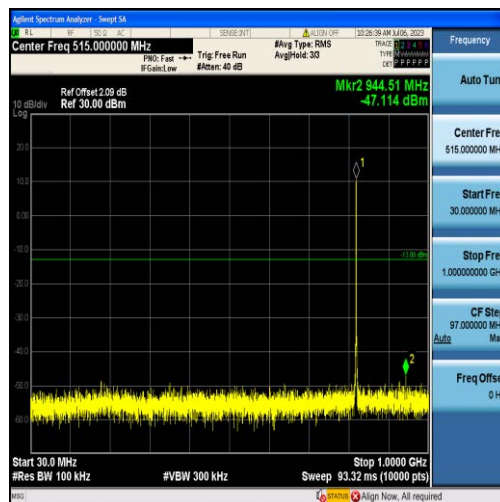
Band26-1.4MHz-16QAM-26783-6RB#0-Range1:30~1000MHz
