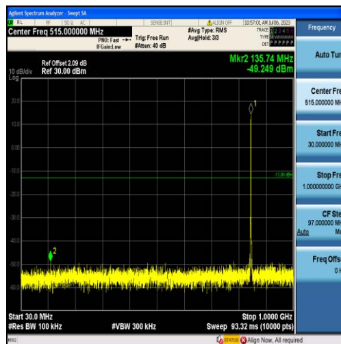
Band26-1.4MHz-16QAM-27033-6RB#0-Range1:30~1000MHz
