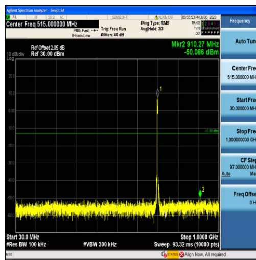
Band17-5MHz-16QAM-23755-25RB#0-Range1:30~1000MHz
