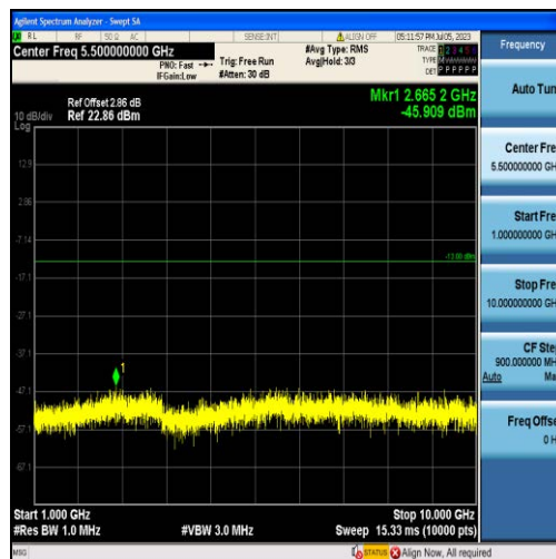
Band12-10MHz-16QAM-23130-50RB#0-Range2:1000~10000MHz
