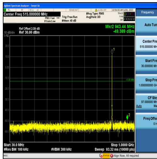
Band26-1.4MHz-16QAM-26797-6RB#0-Range1:30~1000MHz
