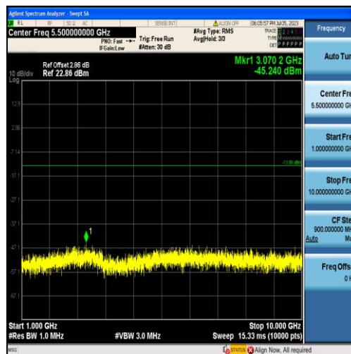
Band17-10MHz-QPSK-23780-50RB#0-Range2:1000~10000MHz
