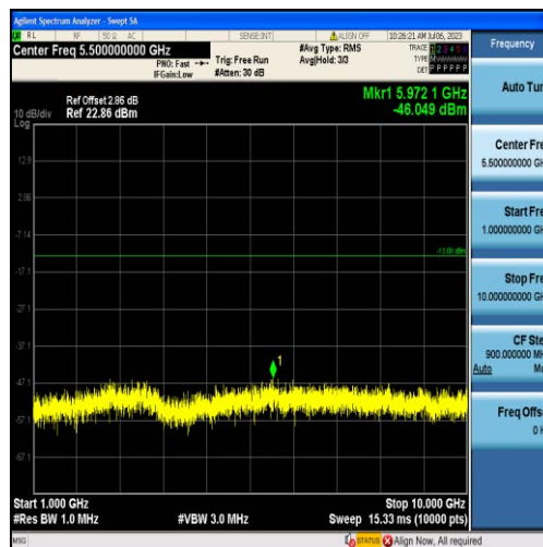
Band26-1.4MHz-16QAM-26740-6RB#0-Range2:1000~10000MHz
