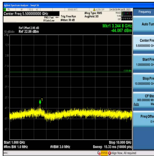
Band12-5MHz-QPSK-23035-25RB#0-Range2:1000~10000MHz
