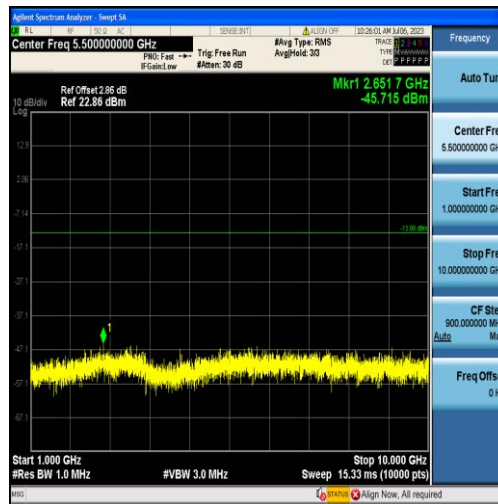
Band26-1.4MHz-16QAM-26697-6RB#0-Range2:1000~10000MHz
