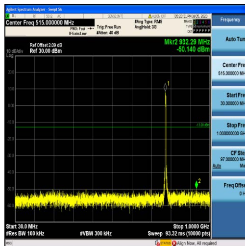
Band13-5MHz-16QAM-23205-25RB#0-Range1:30~1000MHz
