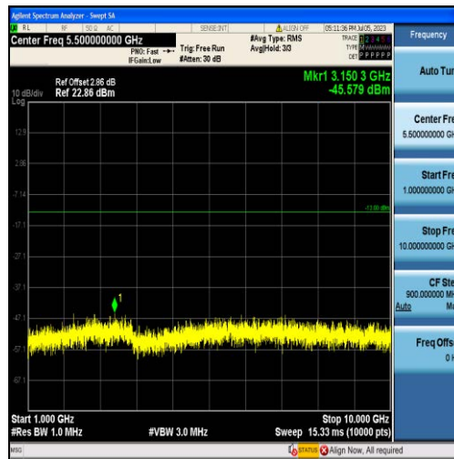
Band12-10MHz-16QAM-23095-50RB#0-Range2:1000~10000MHz
