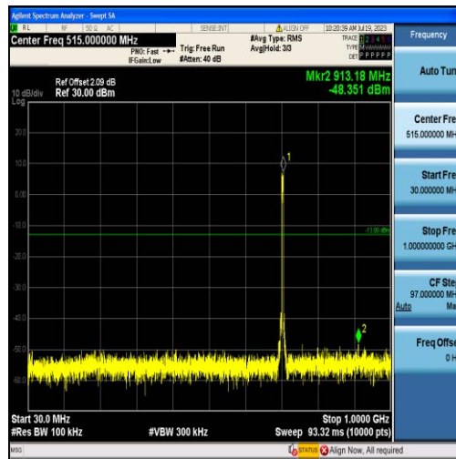
Band17-5MHz-16QAM-23790-25RB#0-Range1:30~1000MHz
