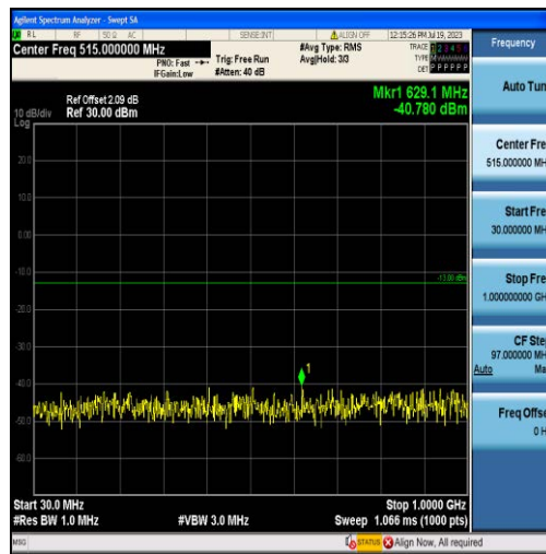
Band4-15MHz-16QAM-20175-75RB#0-Range1:30~1000MHz
