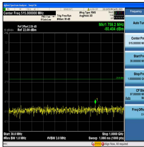
Band7-5MHz-QPSK-21425-25RB#0-Range1:30~1000MHz
