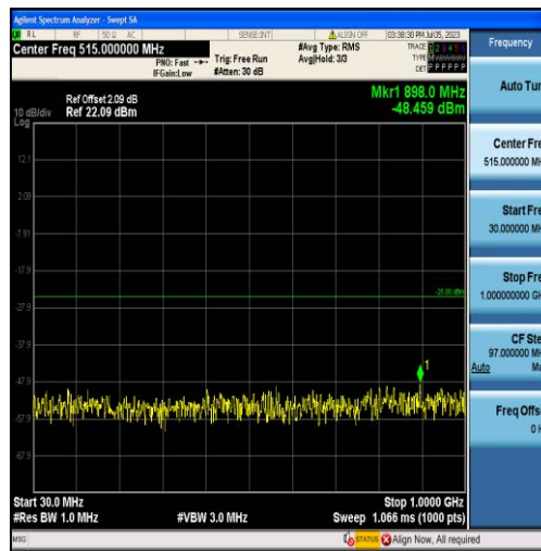
Band7-10MHz-16QAM-20800-50RB#0-Range1:30~1000MHz
