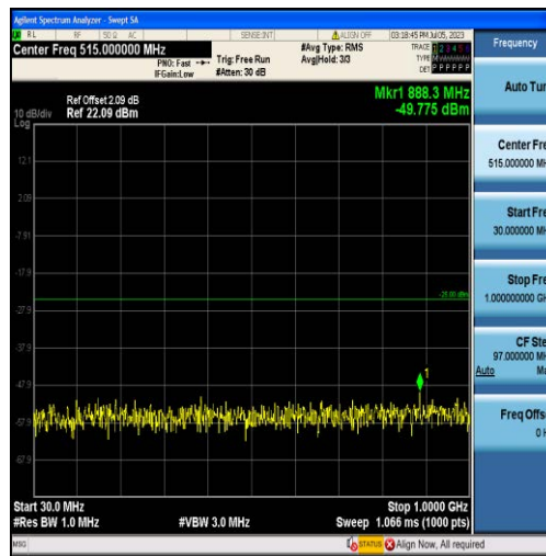
Band7-5MHz-16QAM-20775-25RB#0-Range1:30~1000MHz
