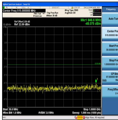
Band7-15MHz-QPSK-21375-75RB#0-Range1:30~1000MHz
