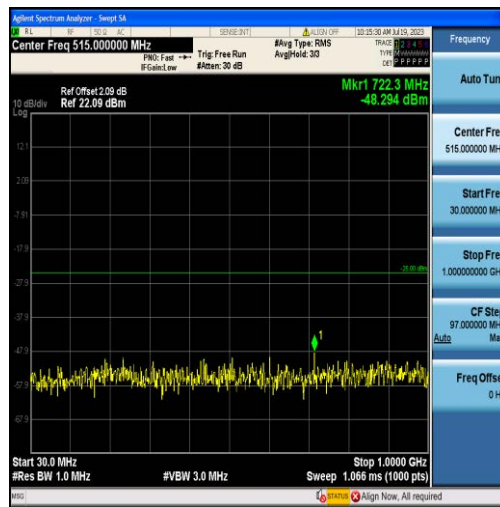
Band7-5MHz-QPSK-21100-25RB#0-Range1:30~1000MHz
