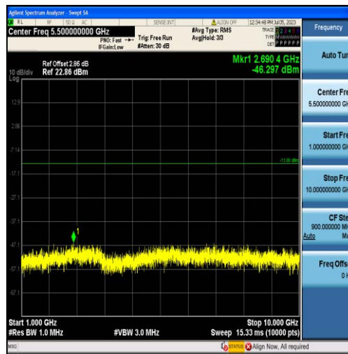
Band5-1.4MHz-16QAM-20407-6RB#0-Range2:1000~10000MHz
