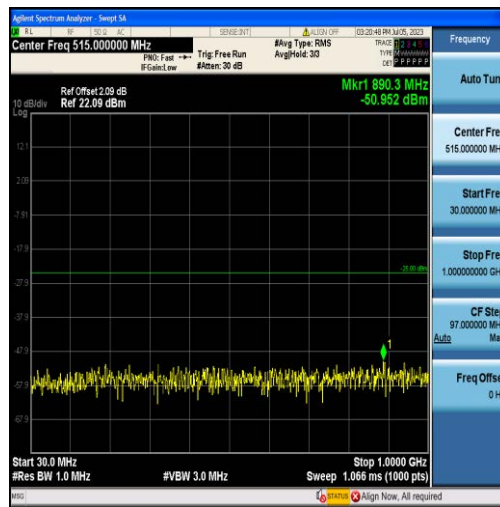
Band7-5MHz-16QAM-21425-25RB#0-Range1:30~1000MHz
