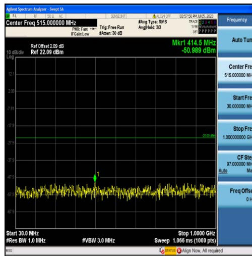
Band7-15MHz-16QAM-20825-75RB#0-Range1:30~1000MHz
