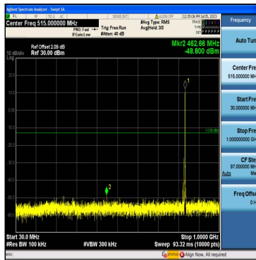
Band5-1.4MHz-16QAM-20525-6RB#0-Range1:30~1000MHz
