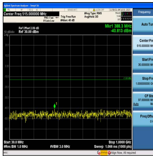
Band4-20MHz-16QAM-20175-100RB#0-Range1:30~1000MHz
