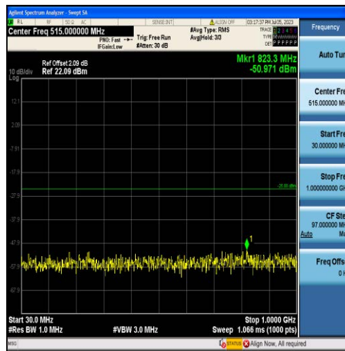
Band7-5MHz-QPSK-20775-25RB#0-Range1:30~1000MHz
