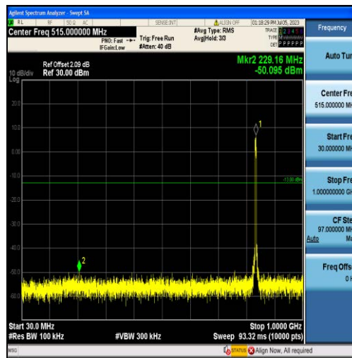
Band5-5MHz-16QAM-20525-25RB#0-Range1:30~1000MHz
