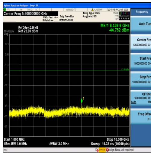
Band5-3MHz-QPSK-20635-15RB#0-Range2:1000~10000MHz
