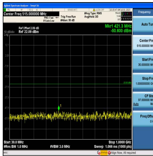
Band7-5MHz-16QAM-21100-25RB#0-Range1:30~1000MHz
