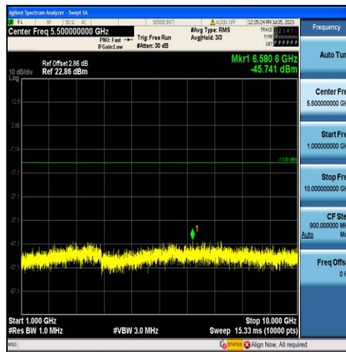
Band5-1.4MHz-QPSK-20643-6RB#0-Range2:1000~10000MHz
