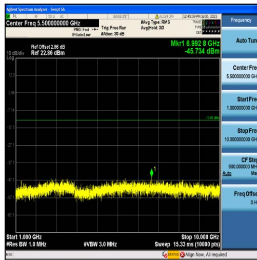
Band5-3MHz-16QAM-20415-15RB#0-Range2:1000~10000MHz
