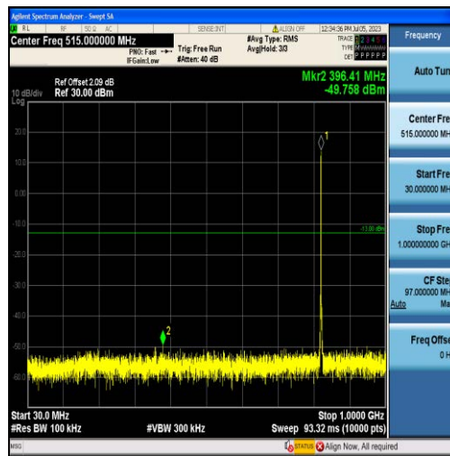
Band5-1.4MHz-QPSK-20407-6RB#0-Range1:30~1000MHz
