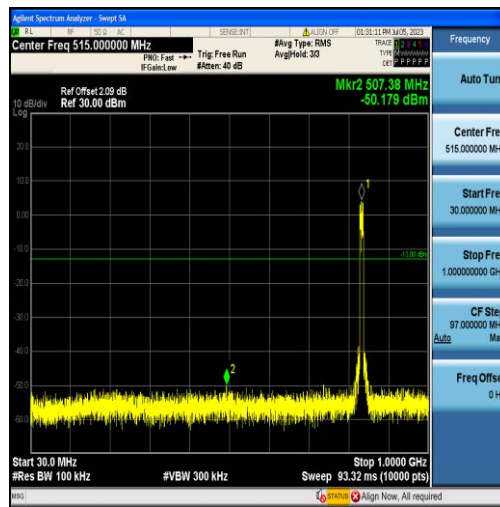
Band5-10MHz-16QAM-20525-50RB#0-Range1:30~1000MHz
