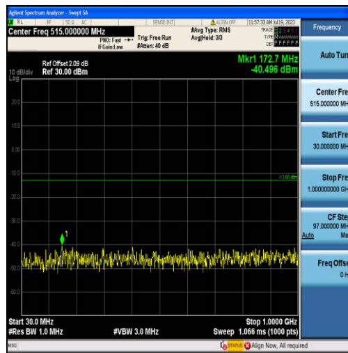
Band4-20MHz-QPSK-20050-100RB#0-Range1:30~1000MHz
