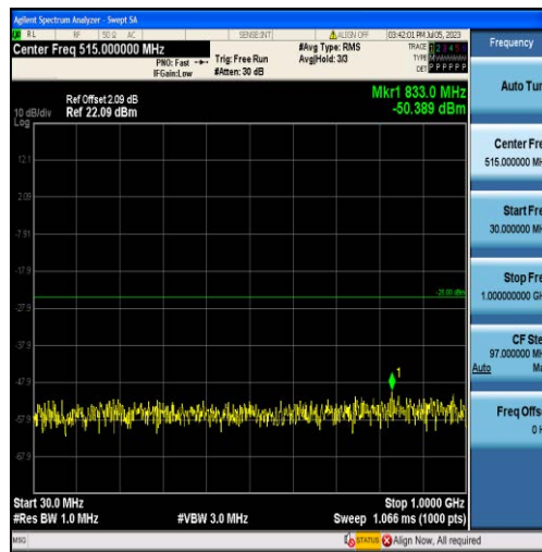
Band7-10MHz-16QAM-21100-50RB#0-Range1:30~1000MHz
