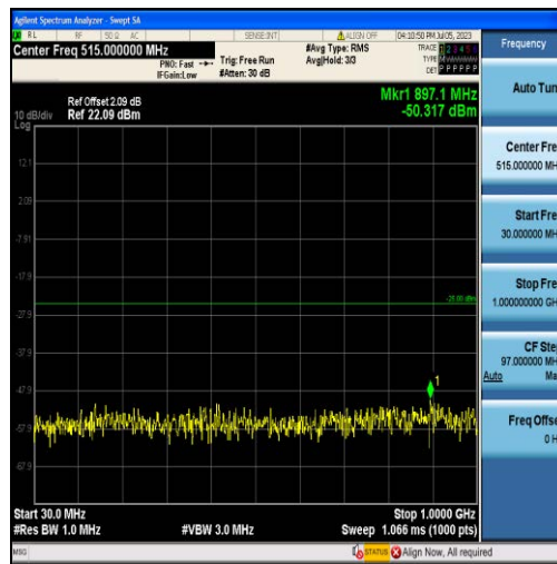
Band7-15MHz-16QAM-21100-75RB#0-Range1:30~1000MHz
