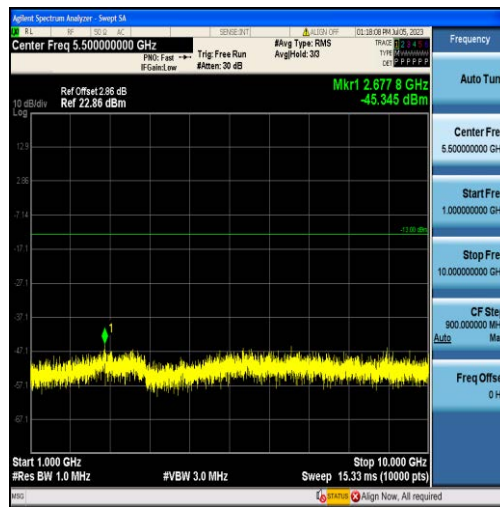
Band5-5MHz-16QAM-20425-25RB#0-Range2:1000~10000MHz
