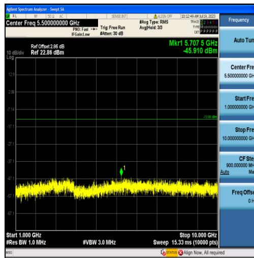
Band5-5MHz-QPSK-20625-25RB#0-Range2:1000~10000MHz
