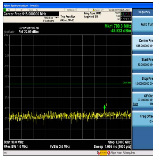
Band7-15MHz-QPSK-21100-75RB#0-Range1:30~1000MHz
