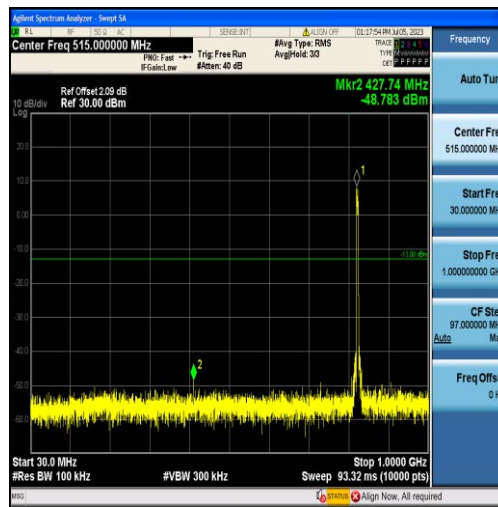
Band5-5MHz-QPSK-20425-25RB#0-Range1:30~1000MHz
