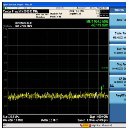
Band7-10MHz-16QAM-21400-50RB#0-Range1:30~1000MHz
