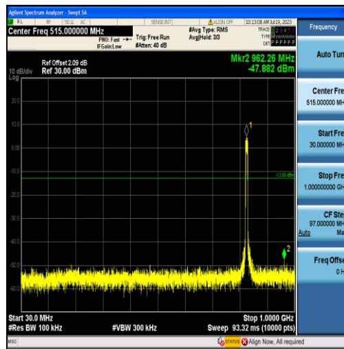
Band5-10MHz-QPSK-20450-50RB#0-Range1:30~1000MHz
