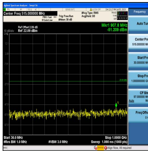
Band7-15MHz-16QAM-21375-75RB#0-Range1:30~1000MHz
