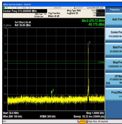
Band5-3MHz-16QAM-20525-15RB#0-Range1:30~1000MHz
