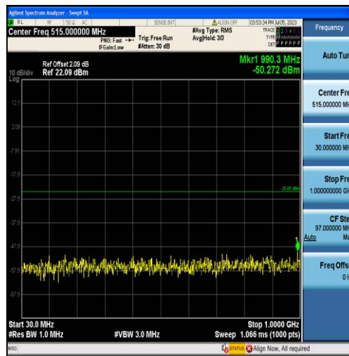
Band7-15MHz-QPSK-20825-75RB#0-Range1:30~1000MHz
