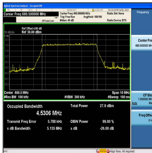
Band71-5MHz-QPSK-133297-25RB#0-4.5306
