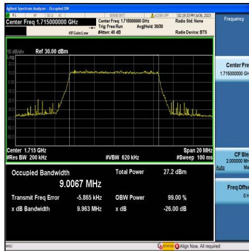
Band66-10MHz-16QAM-132022-50RB#0-9.0067
