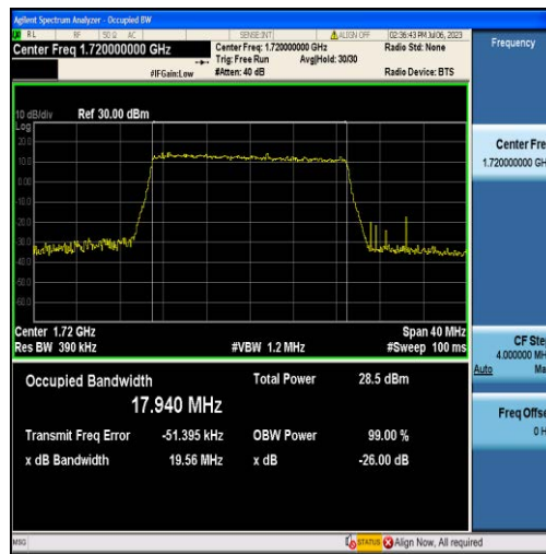
Band66-20MHz-QPSK-132072-100RB#0-17.940
