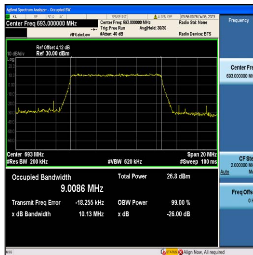
Band71-10MHz-16QAM-133422-50RB#0-9.0086
