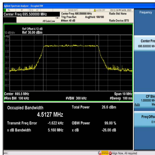
Band71-5MHz-16QAM-133447-25RB#0-4.5127
