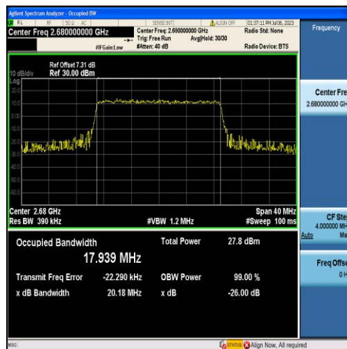
Band41-20MHz-16QAM-41490-100RB#0-17.939
