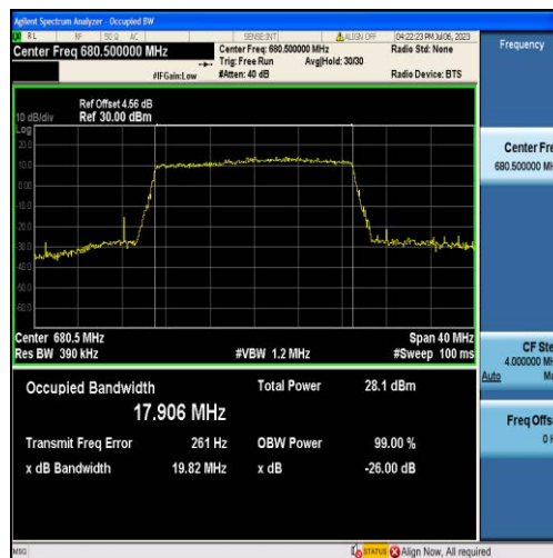
Band71-20MHz-QPSK-133297-100RB#0-17.906
