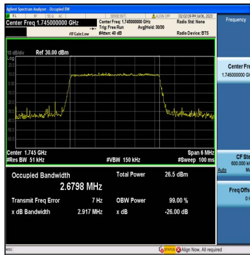
Band66-3MHz-16QAM-132322-15RB#0-2.6798
