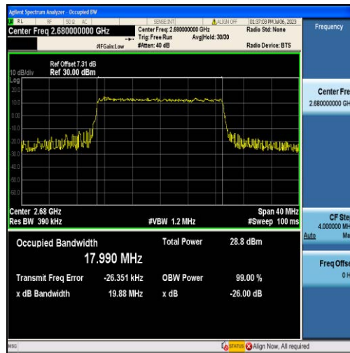
Band41-20MHz-QPSK-41490-100RB#0-17.990
