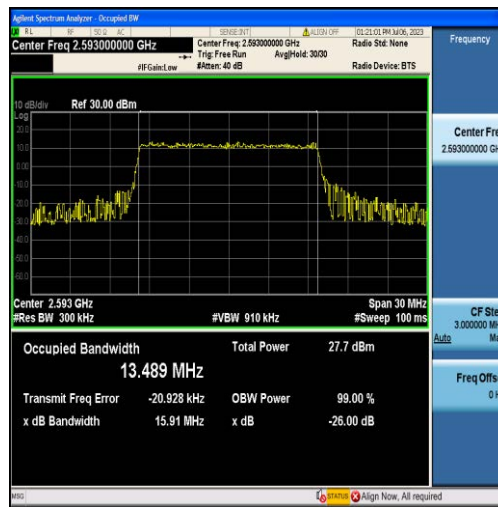
Band41-15MHz-16QAM-40620-75RB#0-13.489
