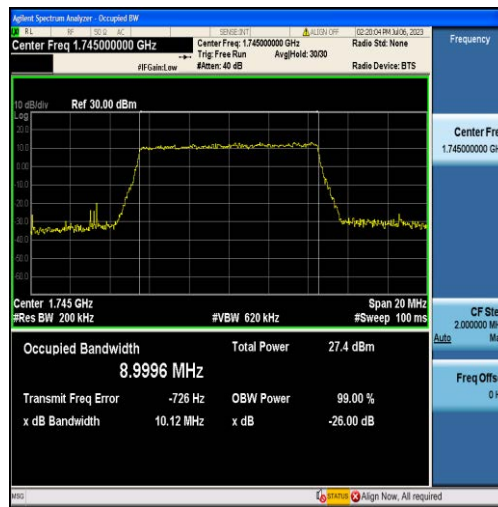
Band66-10MHz-16QAM-132322-50RB#0-8.9996
