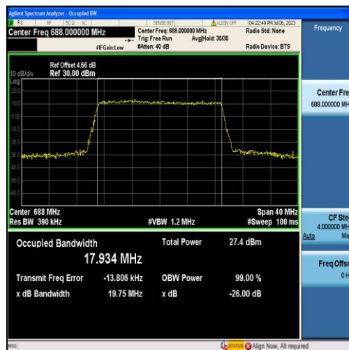
Band71-20MHz-16QAM-133372-100RB#0-17.934
