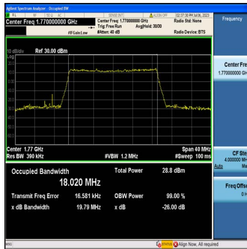
Band66-20MHz-QPSK-132572-100RB#0-18.020
