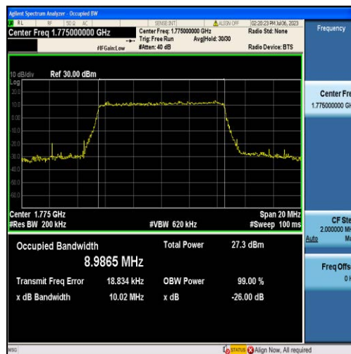
Band66-10MHz-16QAM-132622-50RB#0-8.9865
