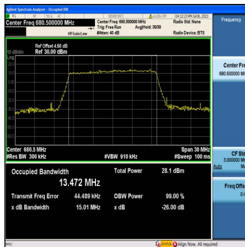
Band71-15MHz-QPSK-133297-75RB#0-13.472
