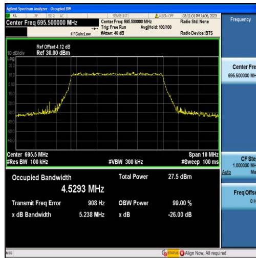
Band71-5MHz-QPSK-133447-25RB#0-4.5293
