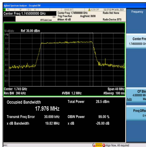
Band66-20MHz-QPSK-132322-100RB#0-17.976
