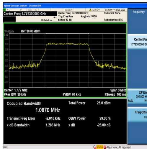
Band66-1.4MHz-16QAM-132665-6RB#0-1.0870
