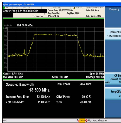
Band66-15MHz-QPSK-132047-75RB#0-13.500
