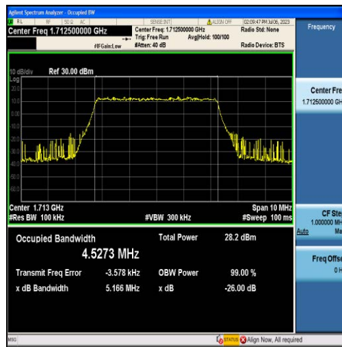
Band66-5MHz-QPSK-131997-25RB#0-4.5273
