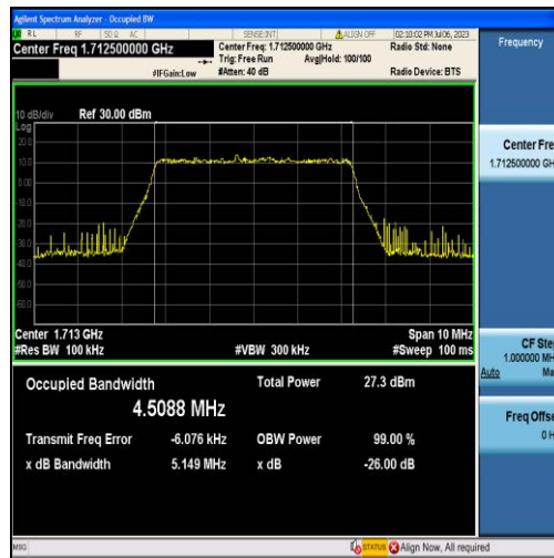
Band66-5MHz-16QAM-131997-25RB#0-4.5088
