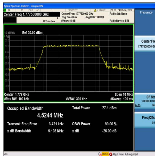
Band66-5MHz-16QAM-132647-25RB#0-4.5244
