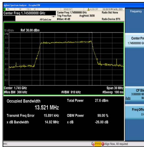
Band66-15MHz-16QAM-132322-75RB#0-13.521
