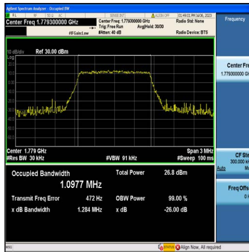
Band66-1.4MHz-QPSK-132665-6RB#0-1.0977
