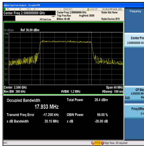
Band41-20MHz-QPSK-39750-100RB#0-17.933
