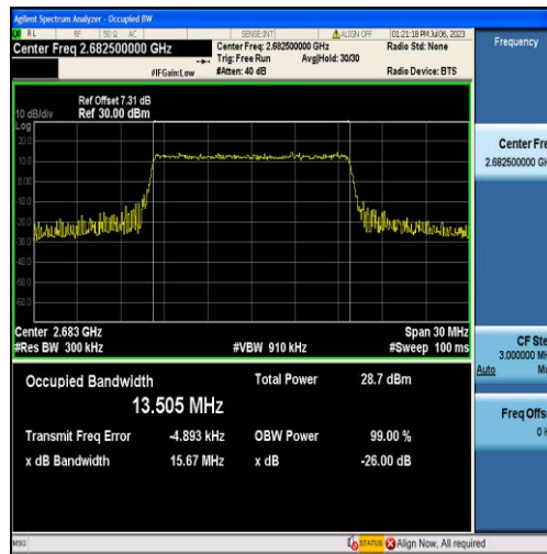
Band41-15MHz-QPSK-41515-75RB#0-13.505
