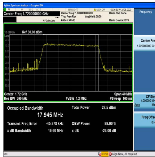
Band66-20MHz-16QAM-132072-100RB#0-17.945
