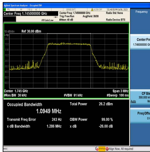
Band66-1.4MHz-16QAM-132322-6RB#0-1.0949
