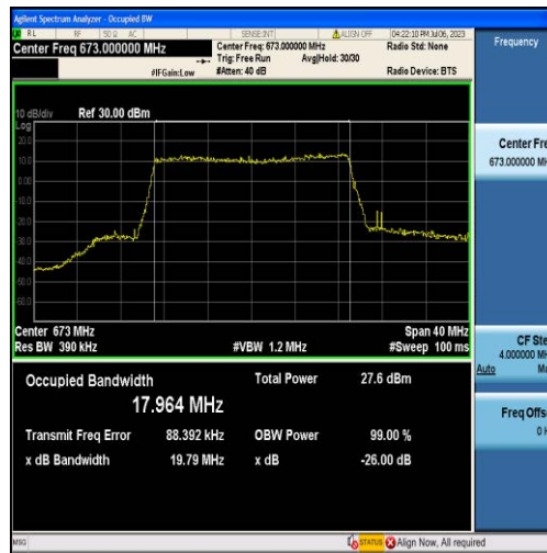
Band71-20MHz-16QAM-133222-100RB#0-17.964
