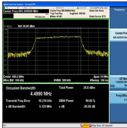
Band71-5MHz-16QAM-133147-25RB#0-4.4990
