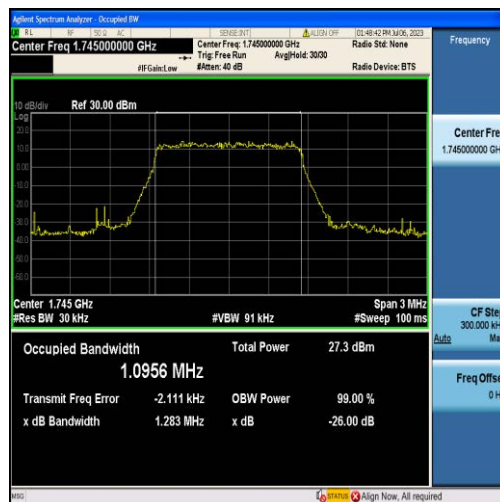
Band66-1.4MHz-QPSK-132322-6RB#0-1.0956
