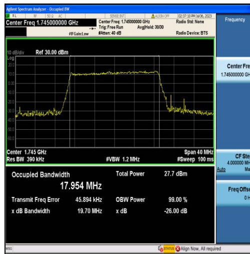
Band66-20MHz-16QAM-132322-100RB#0-17.954
