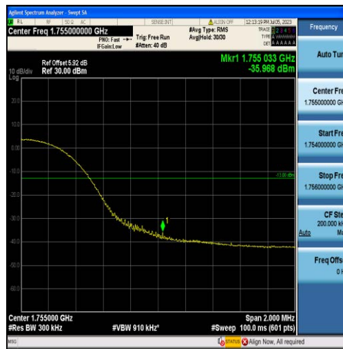
Band4-15MHz-QPSK-20325-75RB#0
