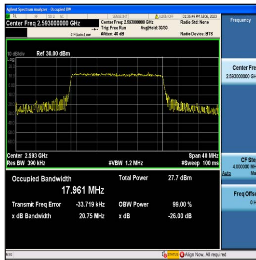
Band41-20MHz-16QAM-40620-100RB#0-17.961
