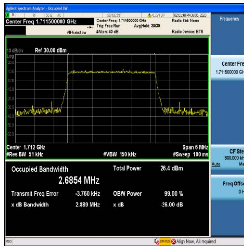
Band66-3MHz-16QAM-131987-15RB#0-2.6854
