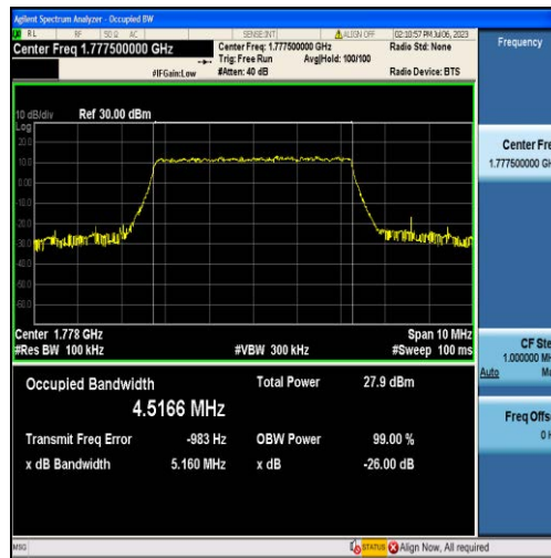
Band66-5MHz-QPSK-132647-25RB#0-4.5166
