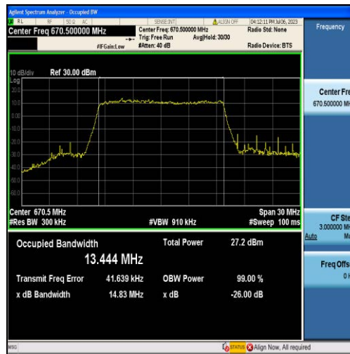
Band71-15MHz-16QAM-133197-75RB#0-13.444
