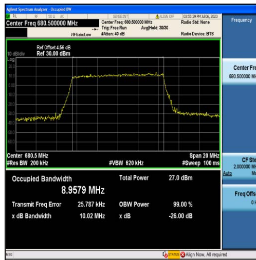
Band71-10MHz-16QAM-133297-50RB#0-8.9579
