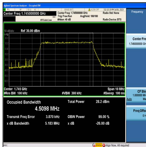
Band66-5MHz-QPSK-132322-25RB#0-4.5098
