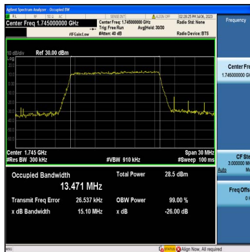
Band66-15MHz-QPSK-132322-75RB#0-13.471
