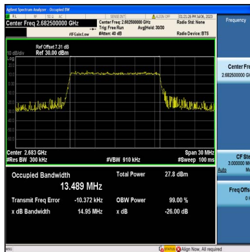
Band41-15MHz-16QAM-41515-75RB#0-13.489
