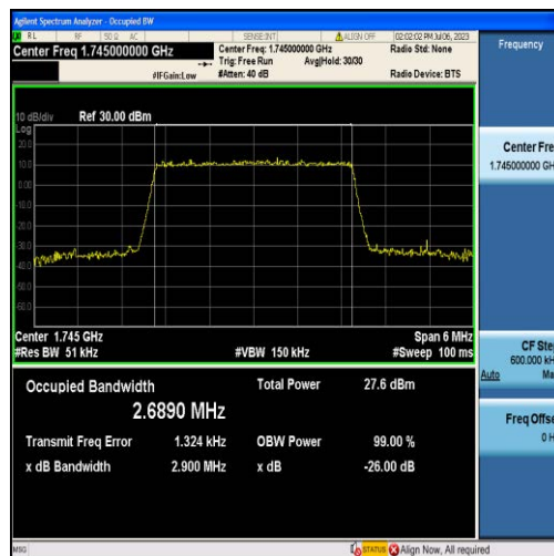
Band66-3MHz-QPSK-132322-15RB#0-2.6890
