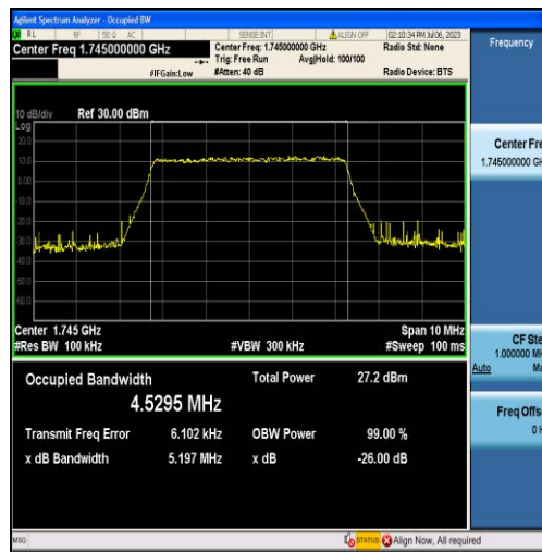
Band66-5MHz-16QAM-132322-25RB#0-4.5295
