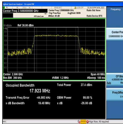
Band41-20MHz-16QAM-39750-100RB#0-17.923
