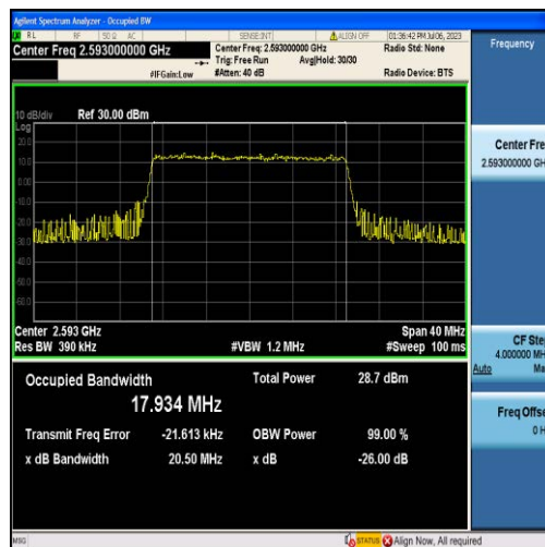
Band41-20MHz-QPSK-40620-100RB#0-17.934
