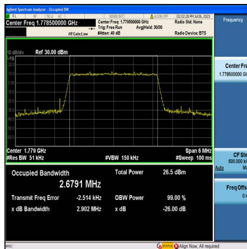
Band66-3MHz-16QAM-132657-15RB#0-2.6791
