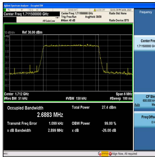
Band66-3MHz-QPSK-131987-15RB#0-2.6883
