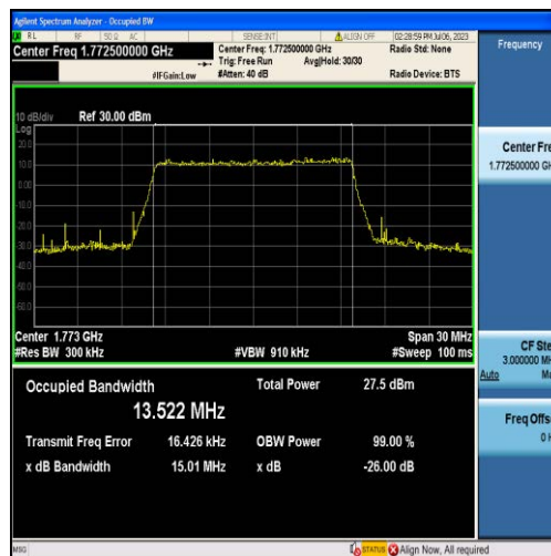
Band66-15MHz-16QAM-132597-75RB#0-13.522
