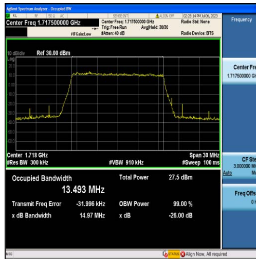
Band66-15MHz-16QAM-132047-75RB#0-13.493
