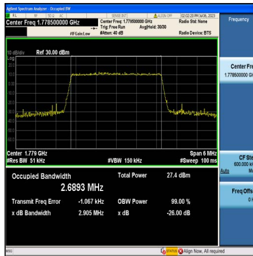
Band66-3MHz-QPSK-132657-15RB#0-2.6893
