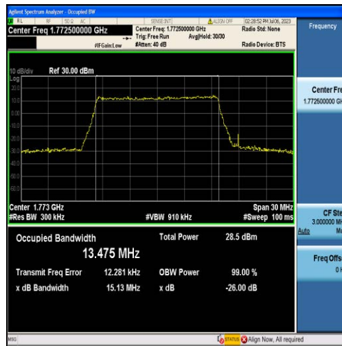
Band66-15MHz-QPSK-132597-75RB#0-13.475
