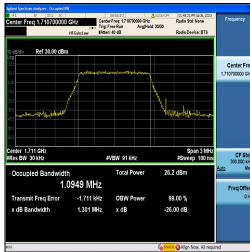
Band66-1.4MHz-16QAM-131979-6RB#0-1.0949
