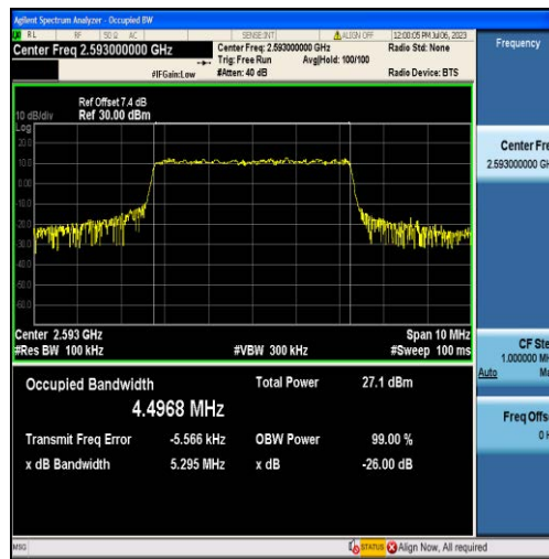
Band41-5MHz-16QAM-40620-25RB#0-4.4968
