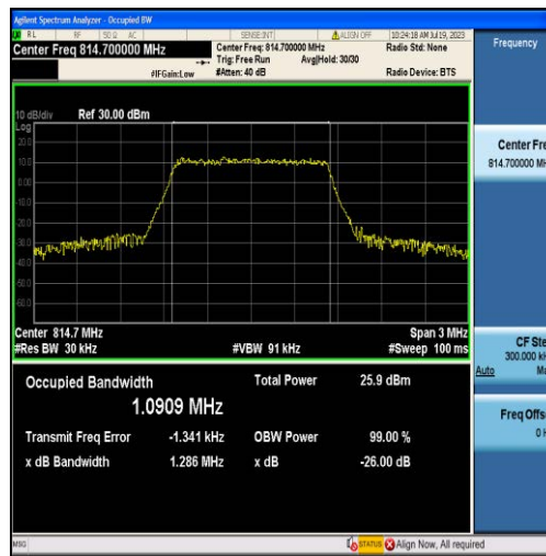
Band26-1.4MHz-16QAM-26697-6RB#0-1.0909
