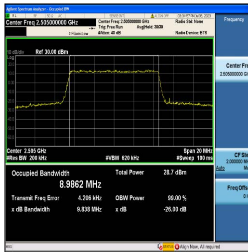
Band7-10MHz-QPSK-20800-50RB#0-8.9862
