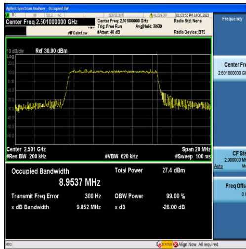
Band41-10MHz-16QAM-39700-50RB#0-8.9537
