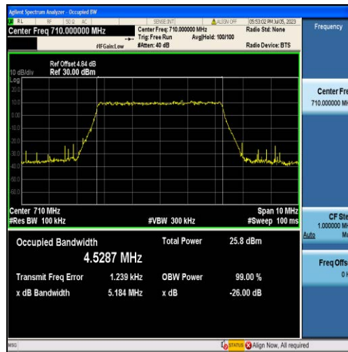
Band17-5MHz-QPSK-23790-25RB#0-4.5287
