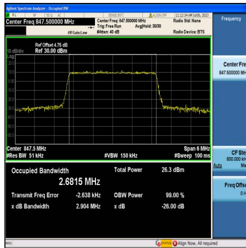
Band26-3MHz-16QAM-27025-15RB#0-2.6815
