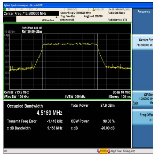
Band12-5MHz-QPSK-23155-25RB#0-4.5190
