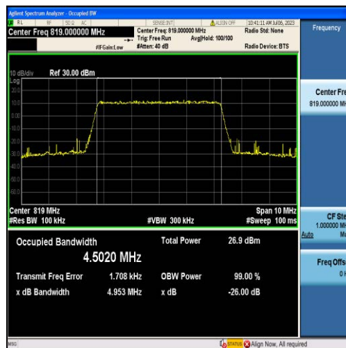
Band26-5MHz-16QAM-26740-25RB#0-4.5020
