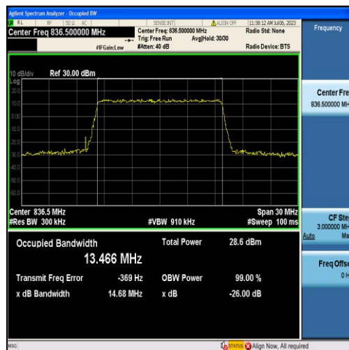
Band26-15MHz-QPSK-26915-75RB#0-13.466
