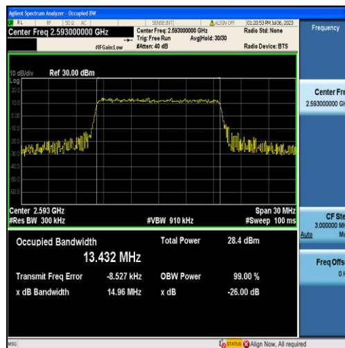
Band41-15MHz-QPSK-40620-75RB#0-13.432
