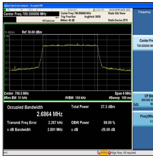
Band12-3MHz-QPSK-23025-15RB#0-2.6864
