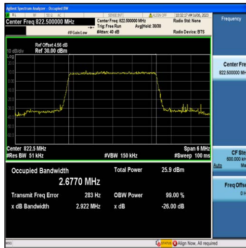
Band26-3MHz-16QAM-26775-15RB#0-2.6770
