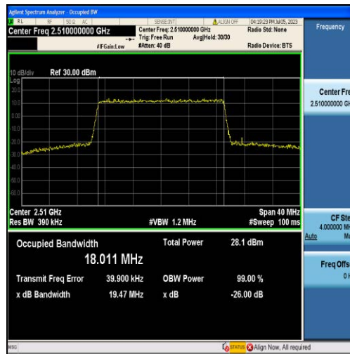
Band7-20MHz-16QAM-20850-100RB#0-18.011
