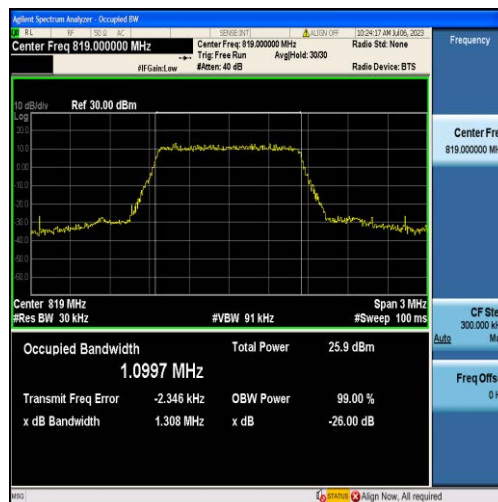
Band26-1.4MHz-16QAM-26740-6RB#0-1.0997
