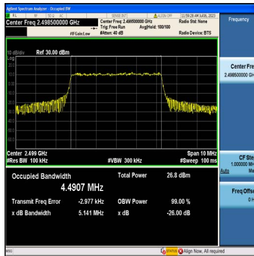
Band41-5MHz-16QAM-39675-25RB#0-4.4907
