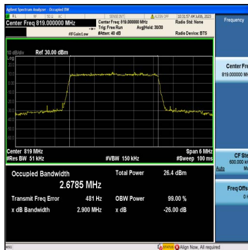
Band26-3MHz-16QAM-26740-15RB#0-2.6785
