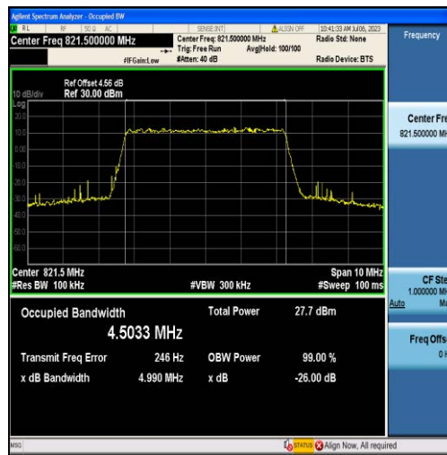
Band26-5MHz-QPSK-26765-25RB#0-4.5033
