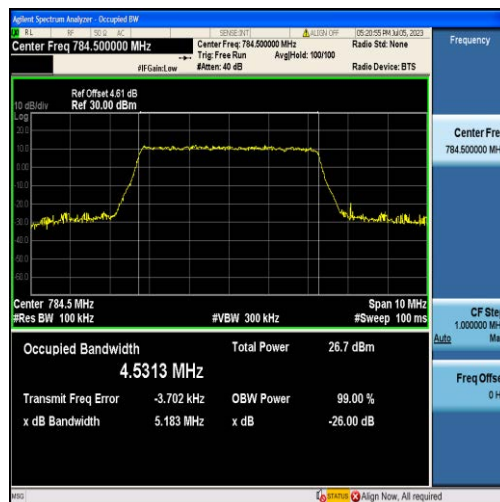
Band13-5MHz-16QAM-23255-25RB#0-4.5313
