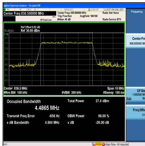
Band26-5MHz-16QAM-26915-25RB#0-4.4865
