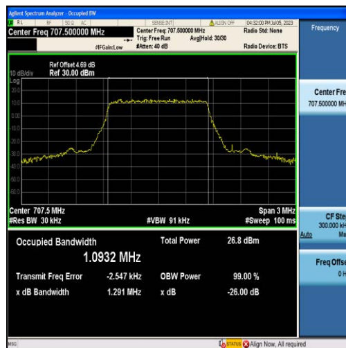
Band12-1.4MHz-QPSK-23095-6RB#0-1.0932
