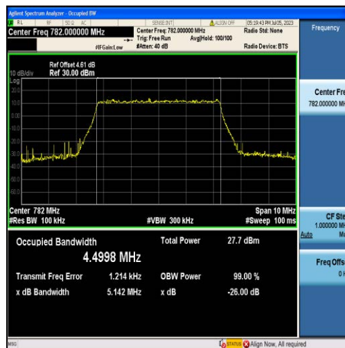
Band13-5MHz-QPSK-23230-25RB#0-4.4998
